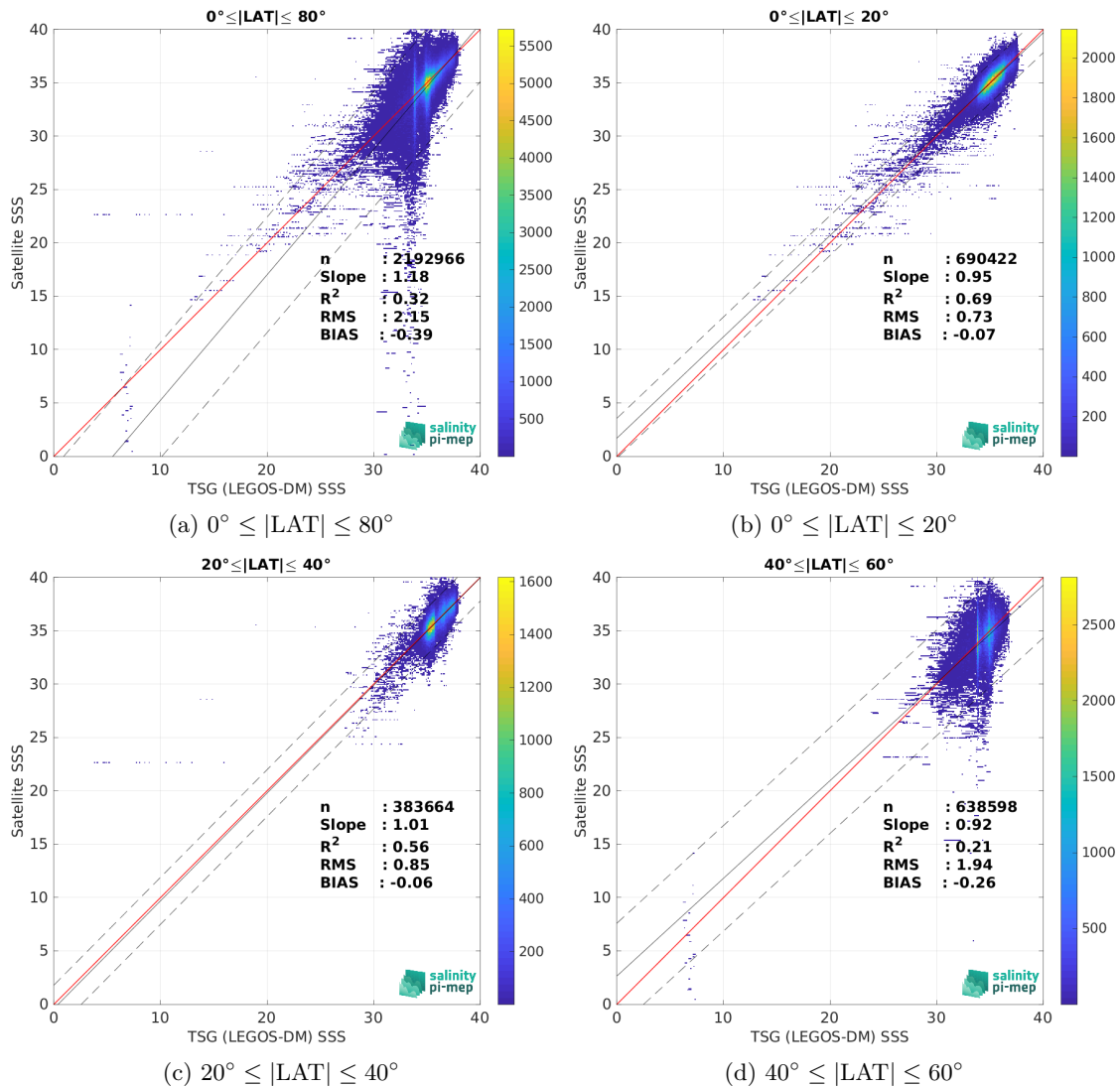
Figure 9: Contour maps of the concentration of SMOS SSS L2 v700 (ESA) SSS (y-axis) versus TSG (LEGOS-DM) SSS (x-axis) at match-up pairs for different latitude bands. For each plot, the red line shows x=y . The black thin and dashed lines indicate a linear fit through the data cloud and the \pm 95\% confidence levels, respectively. The number match-up pairs n , the slope and R^2 coefficient of the linear fit, the root mean square (RMS) and the mean bias between satellite and in situ data are indicated for each latitude band in each plots.
