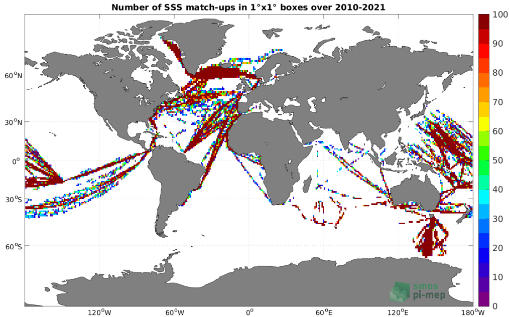
Figure 4: Number of SSS match-ups between TSG (LEGOS-DM) SSS and the SMOS SSS L2 v700 (ESA) SSS product for the Global Ocean Pi-MEP region over 1^\circ \times 1^\circ boxes and for the full satellite product period.
