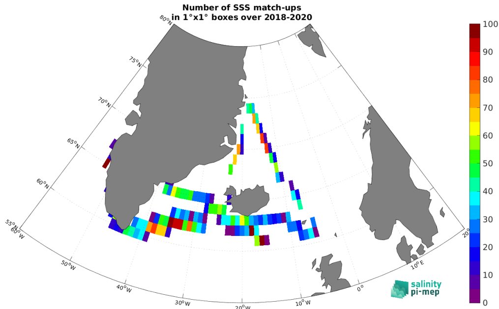
Figure 5: Number of SSS match-ups between TSG (Lauge-Koch) SSS and the SMOS SSS L2 v700 (ESA) SSS product for the Global Ocean Pi-MEP region over 1^\circ \times 1^\circ boxes and for the full satellite product period.
