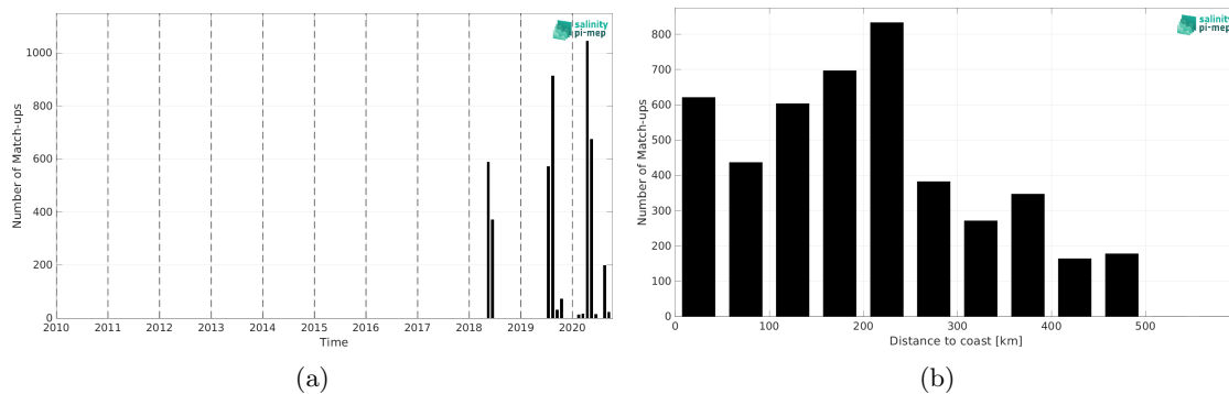
Figure 2: Number of match-ups between TSG (Lauge-Koch) and SMOS SSS L2 v700 (ESA) SSS as a function of time (a) and as function of the distance to coast (b) over the Global Ocean Pi-MEP region and for the full satellite product period.
