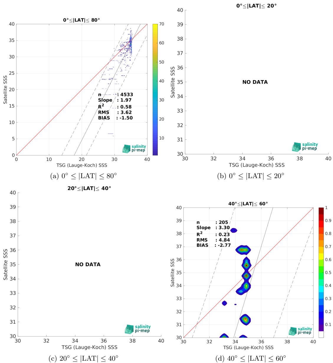
Figure 10: Contour maps of the concentration of SMOS SSS L2 v700 (ESA) SSS (y-axis) versus TSG (Lauge-Koch) SSS (x-axis) at match-up pairs for different latitude bands. For each plot, the red line shows x=y . The black thin and dashed lines indicate a linear fit through the data cloud and the \pm 95\% confidence levels, respectively. The number match-up pairs n , the slope and R^2 coefficient of the linear fit, the root mean square (RMS) and the mean bias between satellite and in situ data are indicated for each latitude band in each plots.
