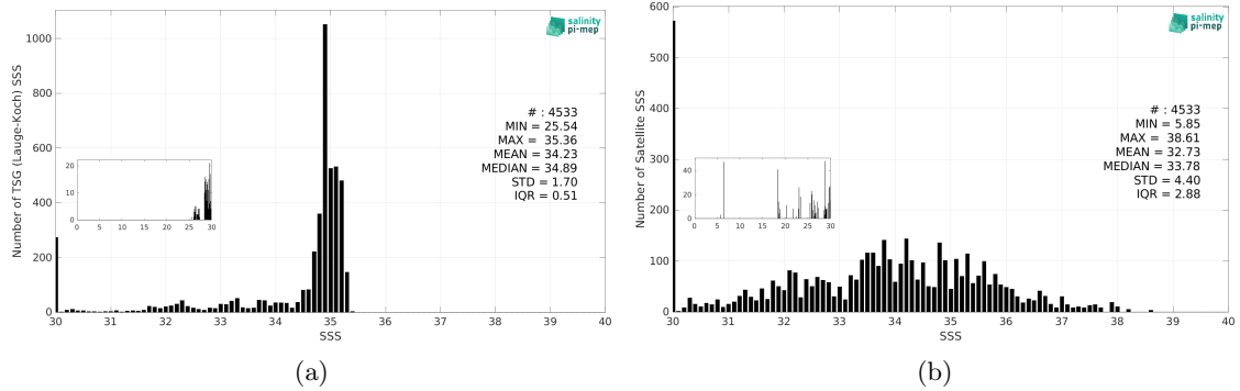
Figure 3: Histograms of SSS from TSG (Lauge-Koch) (a) and SMOS SSS L2 v700 (ESA) (b) considering all match-up pairs per bins of 0.1 over the Global Ocean Pi-MEP region and for the full satellite product period.
