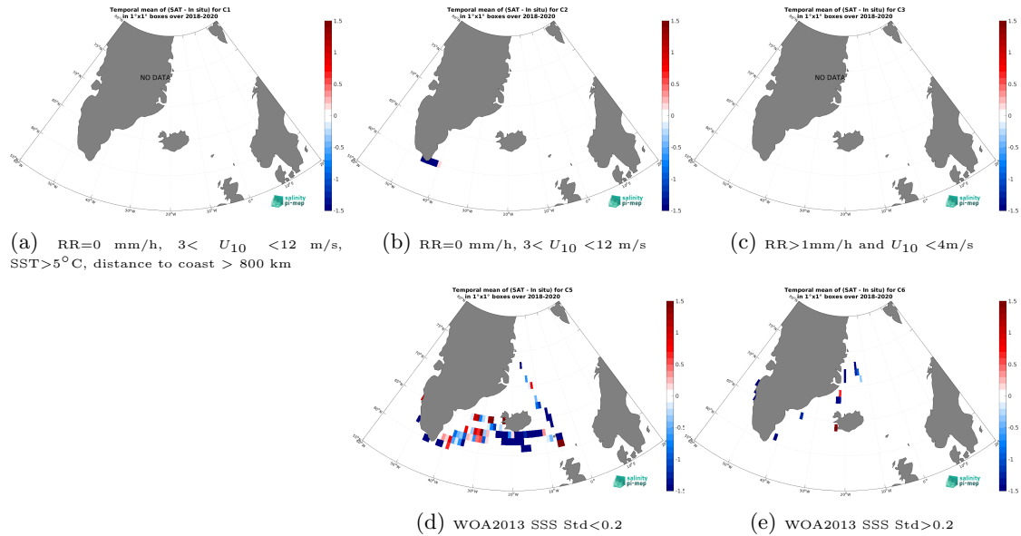
Figure 12: Temporal mean gridded over spatial boxes of size 1^{\circ}\times 1^{\circ} of \Delta\text{SSS} (SMOS SSS L2 v700 (ESA) - TSG (Lauge-Koch)) for 5 different subdatasets corresponding to:RR=0 mm/h, 3 < U_{10} < 12 m/s, SST > 5^{\circ}\text{C} , distance to coast > 800 km (a), RR=0 mm/h, 3 < U_{10} < 12 m/s (b), RR > 1\text{mm/h} and U_{10} < 4\text{m/s} (c), WOA2013 SSS Std < 0.2 (d), WOA2013 SSS Std > 0.2 (e).
