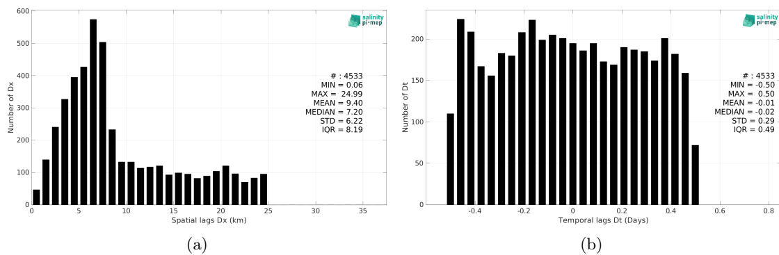
Figure 5: Histograms of the spatial (a) and temporal (b) lags between the location/time of the TSG (Lauge-Koch) measurement and the date of the corresponding SMOS SSS L2 v700 (ESA) SSS pixel.
