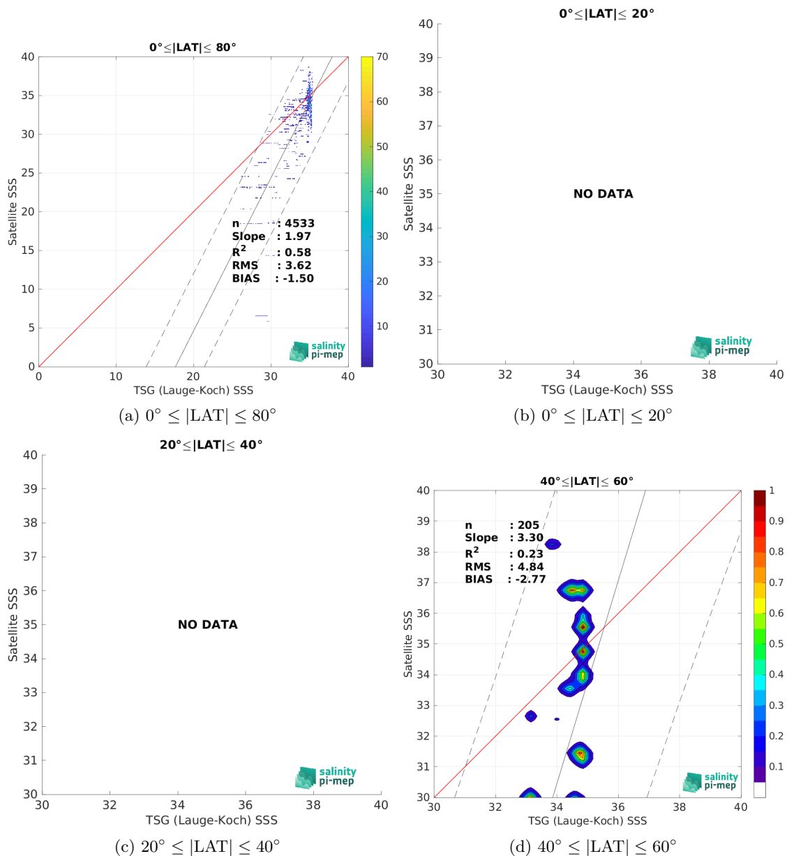
Figure 9: Contour maps of the concentration of SMOS SSS L2 v700 (ESA) SSS (y-axis) versus TSG (Lauge-Koch) SSS (x-axis) at match-up pairs for different latitude bands. For each plot, the red line shows x=y . The black thin and dashed lines indicate a linear fit through the data cloud and the \pm 95\% confidence levels, respectively. The number match-up pairs n , the slope and R^2 coefficient of the linear fit, the root mean square (RMS) and the mean bias between satellite and in situ data are indicated for each latitude band in each plots.
