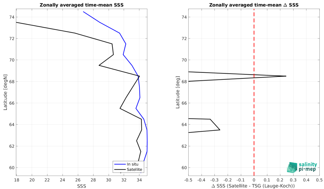
Figure 8: Left panel: Zonal mean SSS from SMOS SSS L2 v700 (ESA) satellite product (black) and from TSG (Lauge-Koch) (blue). Right panel: Zonal mean of \Delta SSS (Satellite - TSG (Lauge-Koch)) for all the collected Pi-MEP match-up pairs estimated over the full satellite product period.
