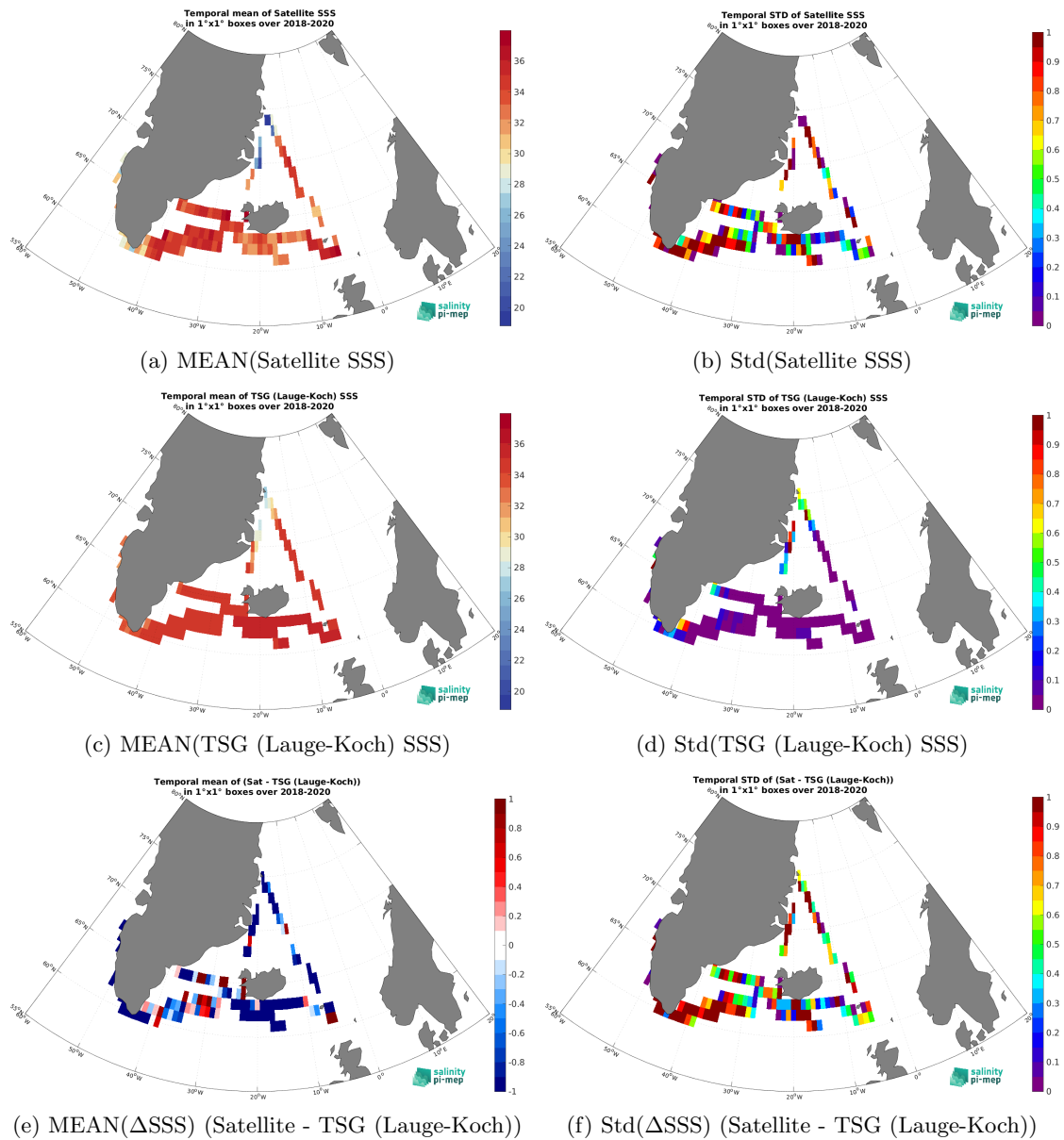
Figure 6: Temporal mean (left) and Std (right) of SSS from SMOS SSS L2 v700 (ESA) (top), TSG (Lauge-Koch) (middle), and of \Delta SSS (Satellite - TSG (Lauge-Koch)). Only match-up pairs are used to generate these maps.
