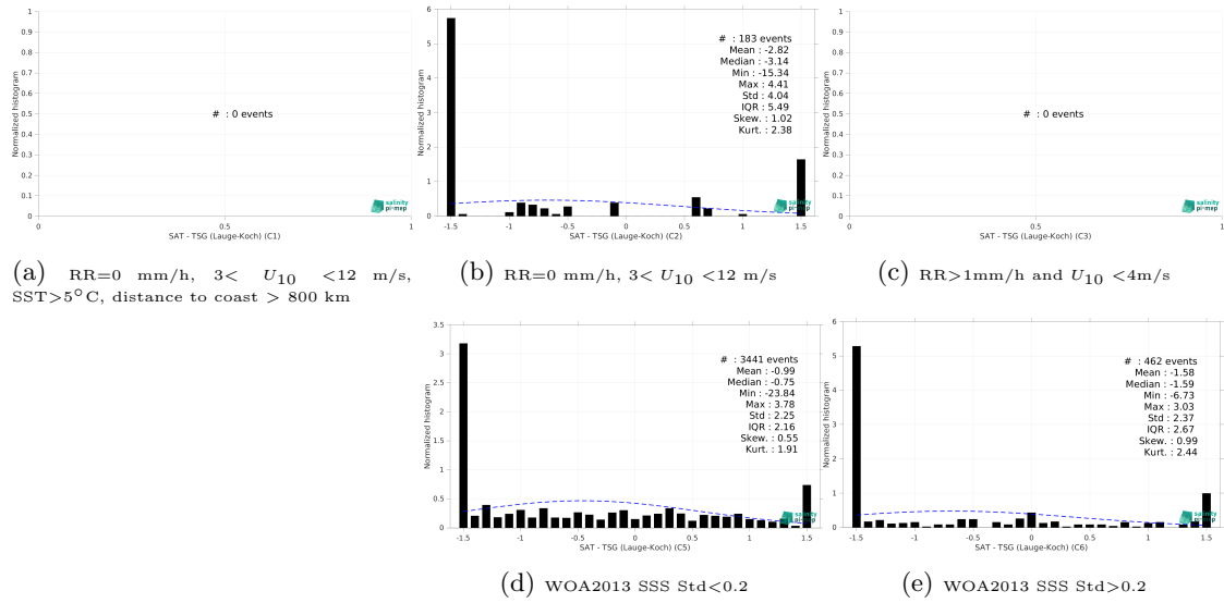
Figure 13: Normalized histogram of \Delta SSS (SMOS SSS L2 v700 (ESA) - TSG (Lauge-Koch)) for 5 different subdatasets corresponding to: RR=0 mm/h, 3 < U_{10} < 12 m/s, SST > 5°C, distance to coast > 800 km (a), RR=0 mm/h, 3 < U_{10} < 12 m/s (b), RR > 1mm/h and U_{10} < 4 m/s (c), WOA2013 SSS Std < 0.2 (d), WOA2013 SSS Std > 0.2 (e).
