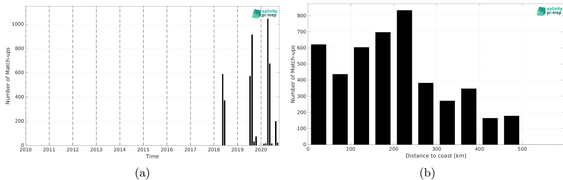
Figure 1: Number of match-ups between TSG (Lauge-Koch) and SMOS SSS L2 v700 (ESA) SSS as a function of time (a) and as function of the distance to coast (b) over the Global Ocean Pi-MEP region and for the full satellite product period.
