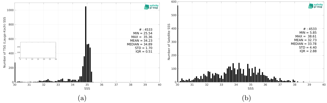
Figure 2: Histograms of SSS from TSG (Lauge-Koch) (a) and SMOS SSS L2 v700 (ESA) (b) considering all match-up pairs per bins of 0.1 over the Global Ocean Pi-MEP region and for the full satellite product period.
