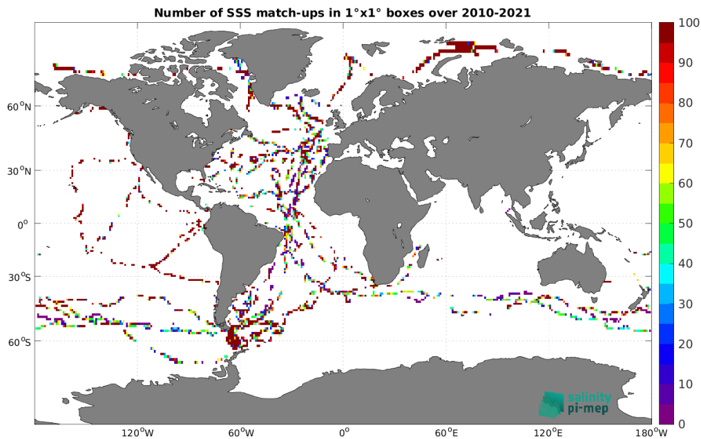
Figure 5: Number of SSS match-ups between TSG (GOSUD-Sailing-ship) SSS and the SMOS SSS L2 v700 (ESA) SSS product for the Global Ocean Pi-MEP region over 1^\circ \times 1^\circ boxes and for the full satellite product period.
