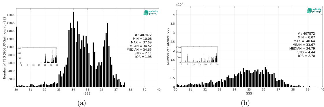
Figure 3: Histograms of SSS from TSG (GOSUD-Sailing-ship) (a) and SMOS SSS L2 v700 (ESA) (b) considering all match-up pairs per bins of 0.1 over the Global Ocean Pi-MEP region and for the full satellite product period.
