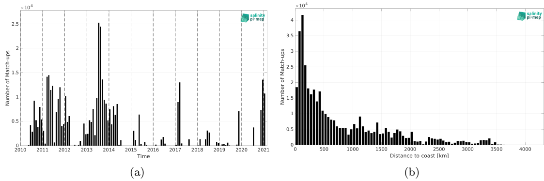
Figure 2: Number of match-ups between TSG (GOSUD-Sailing-ship) and SMOS SSS L2 v700 (ESA) SSS as a function of time (a) and as function of the distance to coast (b) over the Global Ocean Pi-MEP region and for the full satellite product period.
