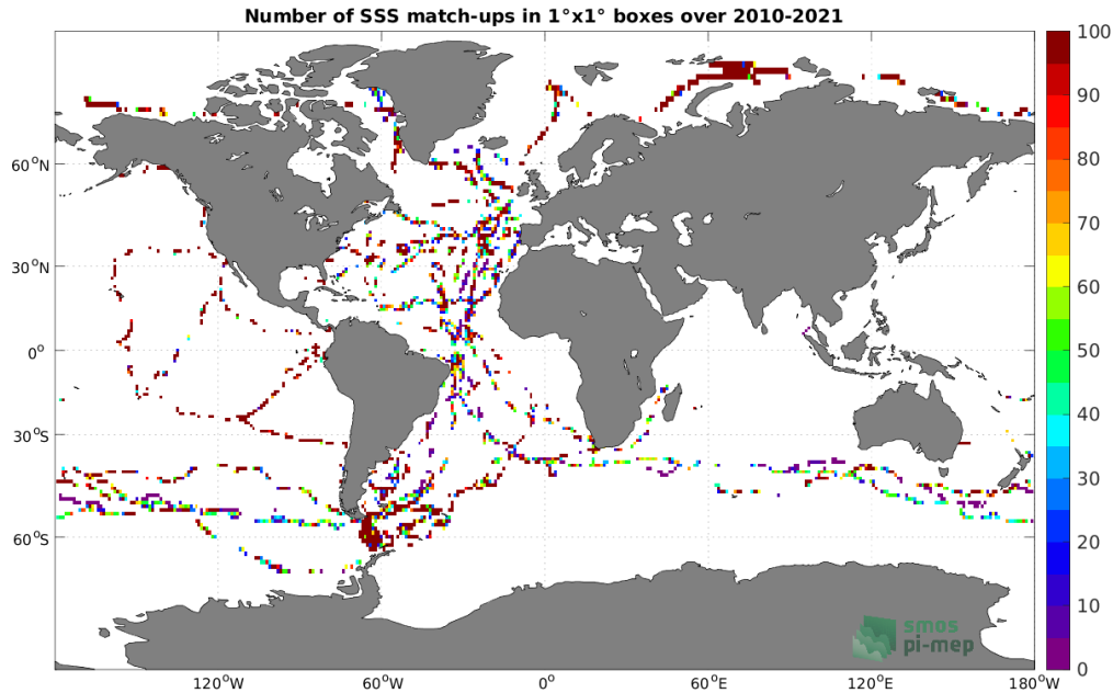
Figure 4: Number of SSS match-ups between TSG (GOSUD-Sailing-ship) SSS and the SMOS SSS L2 v700 (ESA) SSS product for the Global Ocean Pi-MEP region over 1^\circ \times 1^\circ boxes and for the full satellite product period.
