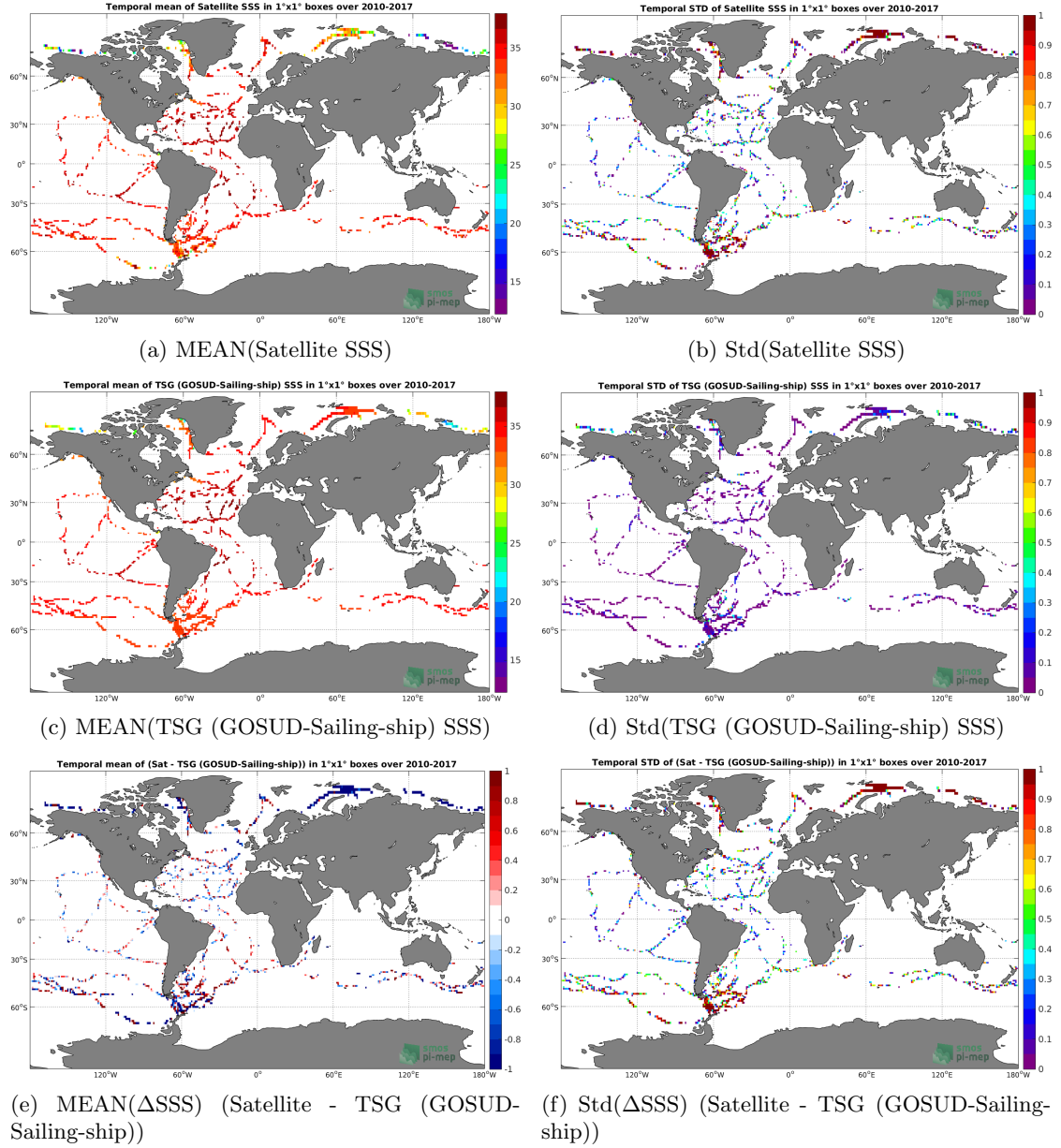
Figure 6: Temporal mean (left) and Std (right) of SSS from SMOS SSS L2 v700 (ESA) (top), TSG (GOSUD-Sailing-ship) (middle), and of \Delta SSS (Satellite - TSG (GOSUD-Sailing-ship)). Only match-up pairs are used to generate these maps.
