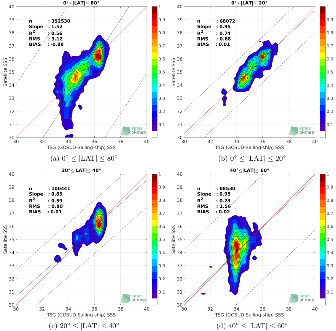
Figure 9: Contour maps of the concentration of SMOS SSS L2 v700 (ESA) SSS (y-axis) versus TSG (GOSUD-Sailing-ship) SSS (x-axis) at match-up pairs for different latitude bands. For each plot, the red line shows x=y . The black thin and dashed lines indicate a linear fit through the data cloud and the \pm 95\% confidence levels, respectively. The number match-up pairs n , the slope and R^2 coefficient of the linear fit, the root mean square (RMS) and the mean bias between satellite and in situ data are indicated for each latitude band in each plots.
