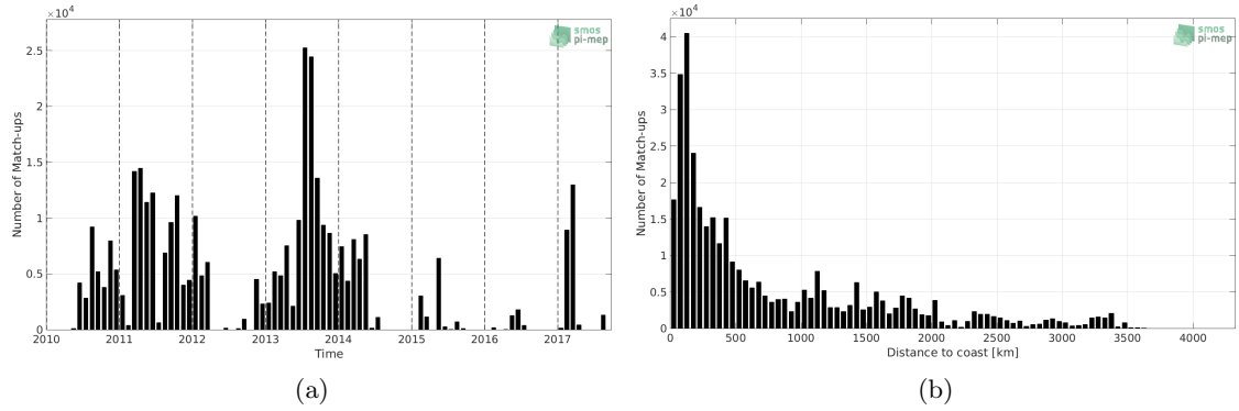
Figure 1: Number of match-ups between TSG (GOSUD-Sailing-ship) and SMOS SSS L2 v700 (ESA) SSS as a function of time (a) and as function of the distance to coast (b) over the Global Ocean Pi-MEP region and for the full satellite product period.
