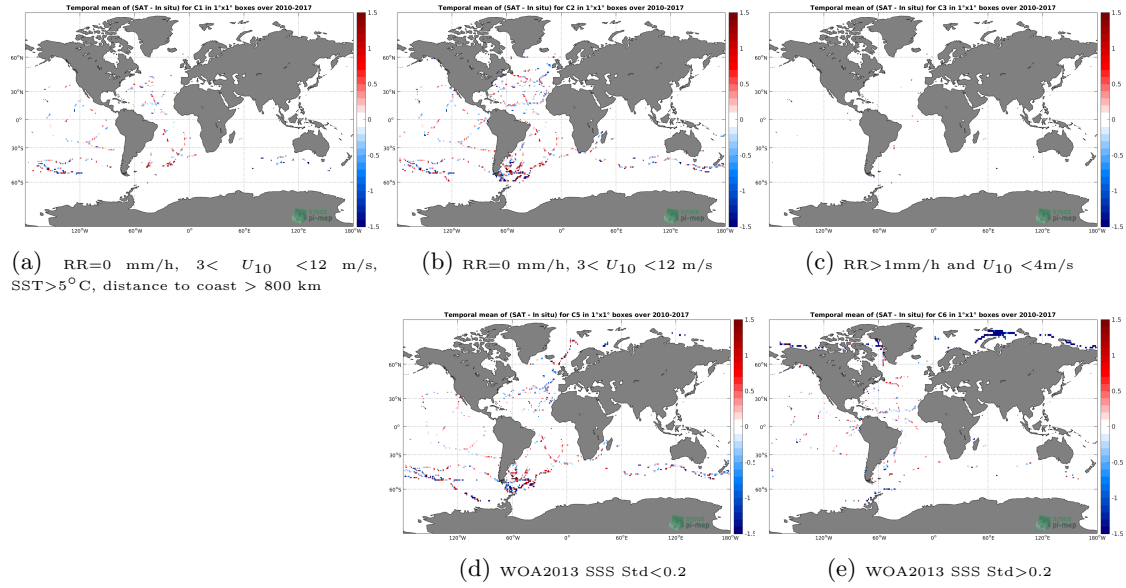
Figure 12: Temporal mean gridded over spatial boxes of size 1^\circ \times 1^\circ of \Delta SSS (SMOS SSS L2 v700 (ESA) - TSG (GOSUD-Sailing-ship)) for 5 different subdatasets corresponding to:RR=0 mm/h, 3 < U_{10} < 12 m/s, SST >5^\circ\text{C} , distance to coast > 800 km (a), RR=0 mm/h, 3 < U_{10} < 12 m/s (b), RR >1 mm/h and U_{10} < 4 m/s (c), WOA2013 SSS Std <0.2 (d), WOA2013 SSS Std >0.2 (e).
