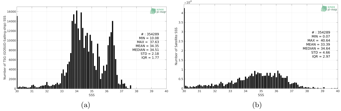
Figure 2: Histograms of SSS from TSG (GOSUD-Sailing-ship) (a) and SMOS SSS L2 v700 (ESA) (b) considering all match-up pairs per bins of 0.1 over the Global Ocean Pi-MEP region and for the full satellite product period.
