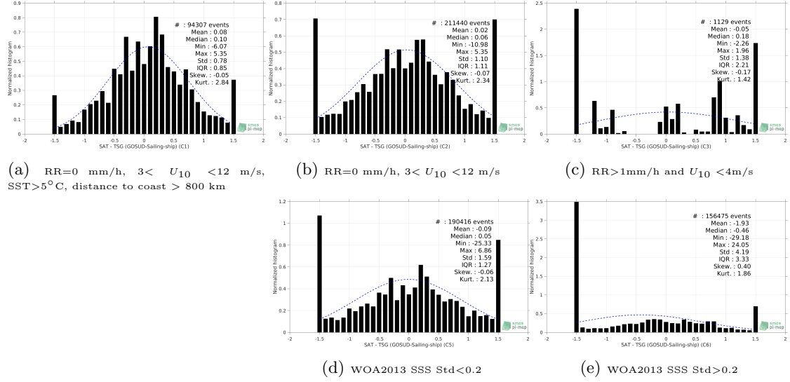
Figure 13: Normalized histogram of \Delta SSS (SMOS SSS L2 v700 (ESA) - TSG (GOSUD-Sailing-ship)) for 5 different subdatasets corresponding to: RR=0 mm/h, 3 < U_{10} < 12 m/s, SST>5°C, distance to coast > 800 km (a), RR=0 mm/h, 3 < U_{10} < 12 m/s (b), RR>1mm/h and U_{10} < 4 m/s (c), WOA2013 SSS Std<0.2 (d), WOA2013 SSS Std>0.2 (e).
