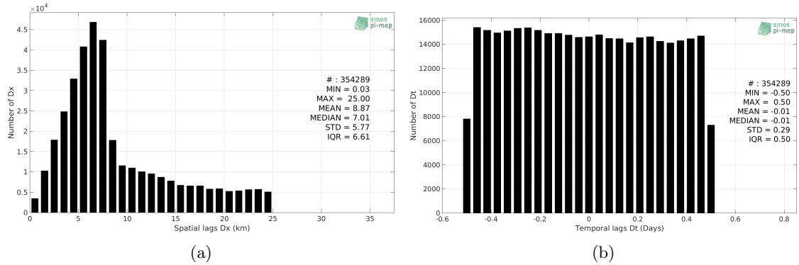
Figure 5: Histograms of the spatial (a) and temporal (b) lags between the location/time of the TSG (GOSUD-Sailing-ship) measurement and the date of the corresponding SMOS SSS L2 v700 (ESA) SSS pixel.
