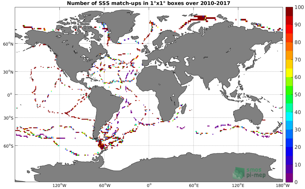
Figure 4: Number of SSS match-ups between TSG (GOSUD-Sailing-ship) SSS and the SMOS SSS L2 v700 (ESA) SSS product for the Global Ocean Pi-MEP region over 1^\circ \times 1^\circ boxes and for the full satellite product period.
