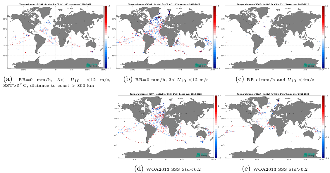
Figure 14: Temporal mean gridded over spatial boxes of size 1^\circ \times 1^\circ of \Delta SSS (SMOS SSS L2 v700 (ESA) - TSG (GOSUD-Research-vessel)) for 5 different subdatasets corresponding to:RR=0 mm/h, 3 < U_{10} < 12 m/s, SST > 5^\circ\text{C} , distance to coast > 800 km (a), RR=0 mm/h, 3 < U_{10} < 12 m/s (b), RR > 1 mm/h and U_{10} < 4 m/s (c), WOA2013 SSS Std < 0.2 (d), WOA2013 SSS Std > 0.2 (e).
