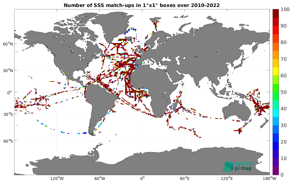
Figure 5: Number of SSS match-ups between TSG (GOSUD-Research-vessel) SSS and the SMOS SSS L2 v700 (ESA) SSS product for the Global Ocean Pi-MEP region over 1^\circ \times 1^\circ boxes and for the full satellite product period.
