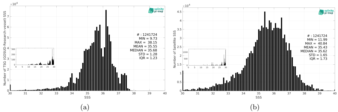
Figure 3: Histograms of SSS from TSG (GOSUD-Research-vessel) (a) and SMOS SSS L2 v700 (ESA) (b) considering all match-up pairs per bins of 0.1 over the Global Ocean Pi-MEP region and for the full satellite product period.
