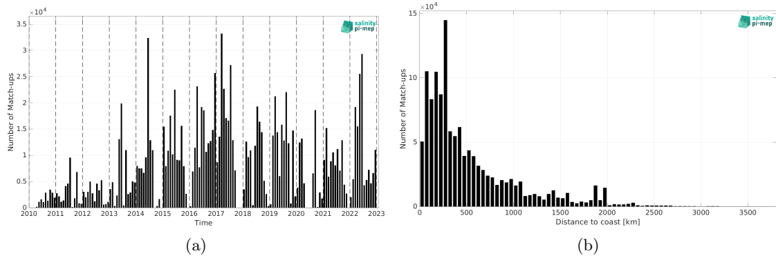
Figure 2: Number of match-ups between TSG (GOSUD-Research-vessel) and SMOS SSS L2 v700 (ESA) SSS as a function of time (a) and as function of the distance to coast (b) over the Global Ocean Pi-MEP region and for the full satellite product period.
