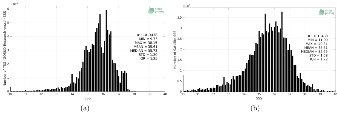
Figure 2: Histograms of SSS from TSG (GOSUD-Research-vessel) (a) and SMOS SSS L2 v700 (ESA) (b) considering all match-up pairs per bins of 0.1 over the Global Ocean Pi-MEP region and for the full satellite product period.
