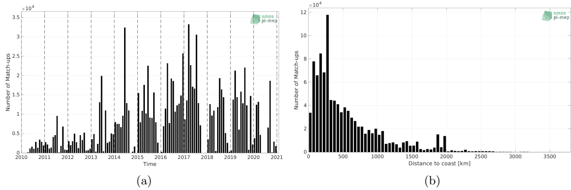
Figure 1: Number of match-ups between TSG (GOSUD-Research-vessel) and SMOS SSS L2 v700 (ESA) SSS as a function of time (a) and as function of the distance to coast (b) over the Global Ocean Pi-MEP region and for the full satellite product period.
