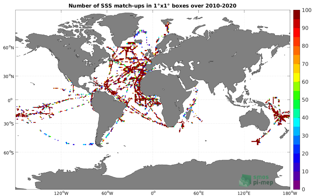
Figure 4: Number of SSS match-ups between TSG (GOSUD-Research-vessel) SSS and the SMOS SSS L2 v700 (ESA) SSS product for the Global Ocean Pi-MEP region over 1^\circ \times 1^\circ boxes and for the full satellite product period.
