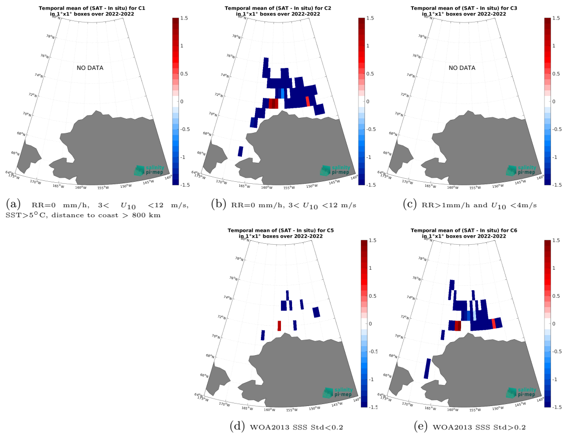
Figure 14: Temporal mean gridded over spatial boxes of size 1^\circ \times 1^\circ of \Delta SSS (SMOS SSS L2 v700 (ESA) - SASSIE) for 5 different subdatasets corresponding to:RR=0 mm/h, 3 < U_{10} < 12 m/s, SST >5^\circ\text{C} , distance to coast > 800 km (a), RR=0 mm/h, 3 < U_{10} < 12 m/s (b), RR >1 mm/h and U_{10} < 4 m/s (c), WOA2013 SSS Std <0.2 (d), WOA2013 SSS Std >0.2 (e).
