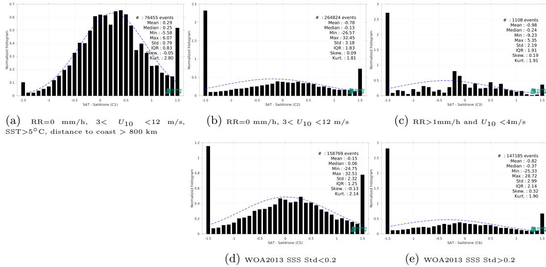
Figure 15: Normalized histogram of \Delta SSS (SMOS SSS L2 v700 (ESA) - Sairdrone) for 5 different subdatasets corresponding to: RR=0 mm/h, 3 < U_{10} < 12 m/s, SST>5°C, distance to coast > 800 km (a), RR=0 mm/h, 3 < U_{10} < 12 m/s (b), RR>1mm/h and U_{10} < 4 m/s (c), WOA2013 SSS Std<0.2 (d), WOA2013 SSS Std>0.2 (e).
