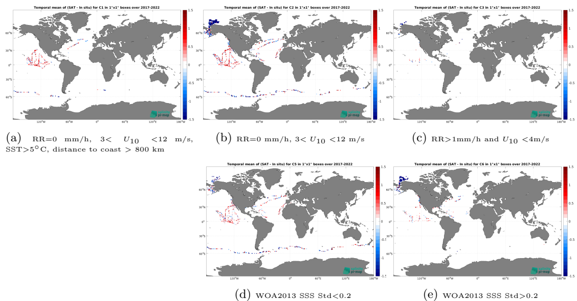
Figure 14: Temporal mean gridded over spatial boxes of size 1^\circ \times 1^\circ of \Delta SSS (SMOS SSS L2 v700 (ESA) - Sairdron) for 5 different subdatasets corresponding to:RR=0 mm/h, 3 < U_{10} < 12 m/s, SST > 5^\circ\text{C} , distance to coast > 800 km (a), RR=0 mm/h, 3 < U_{10} < 12 m/s (b), RR > 1 mm/h and U_{10} < 4 m/s (c), WOA2013 SSS Std < 0.2 (d), WOA2013 SSS Std > 0.2 (e).
