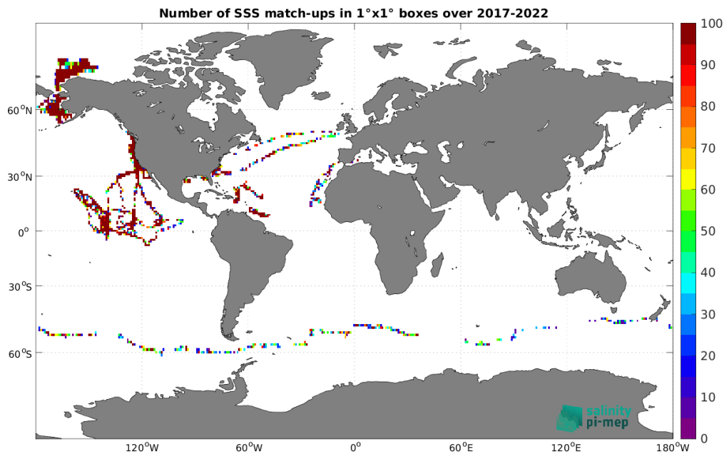
Figure 4: Number of SSS match-ups between Saildrone SSS and the SMOS SSS L2 v700 (ESA) SSS product for the Global Ocean Pi-MEP region over 1^\circ \times 1^\circ boxes and for the full satellite product period.
