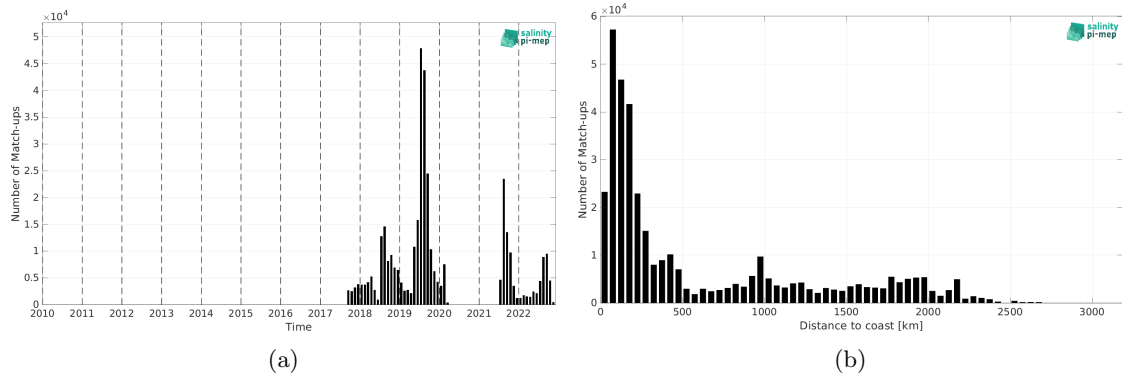
Figure 1: Number of match-ups between Saildrone and SMOS SSS L2 v700 (ESA) SSS as a function of time (a) and as function of the distance to coast (b) over the Global Ocean Pi-MEP region and for the full satellite product period.
