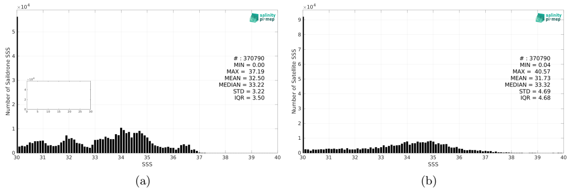
Figure 2: Histograms of SSS from Saildrone (a) and SMOS SSS L2 v700 (ESA) (b) considering all match-up pairs per bins of 0.1 over the Global Ocean Pi-MEP region and for the full satellite product period.
