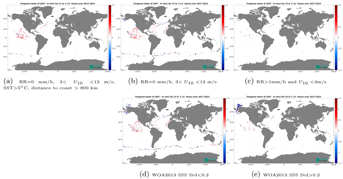
Figure 12: Temporal mean gridded over spatial boxes of size 1^\circ \times 1^\circ of \Delta SSS (SMOS SSS L2 v700 (ESA) - Saldrone) for 5 different subdatasets corresponding to:RR=0 mm/h, 3 < U_{10} < 12 m/s, SST >5^\circ C, distance to coast > 800 km (a), RR=0 mm/h, 3 < U_{10} < 12 m/s (b), RR >1 mm/h and U_{10} < 4 m/s (c), WOA2013 SSS Std <0.2 (d), WOA2013 SSS Std >0.2 (e).
