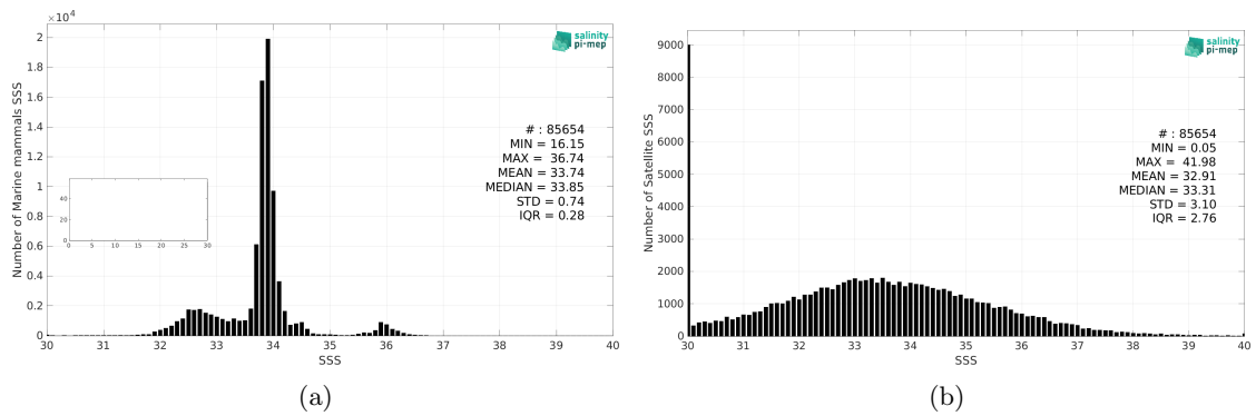
Figure 2: Histograms of SSS from Marine mammals (a) and SMOS SSS L2 v700 (ESA) (b) considering all match-up pairs per bins of 0.1 over the Global Ocean Pi-MEP region and for the full satellite product period.
