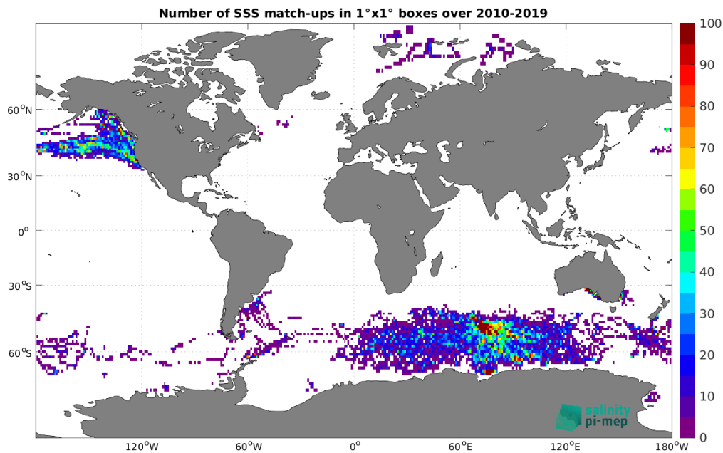
Figure 4: Number of SSS match-ups between Marine mammals SSS and the SMOS SSS L2 v700 (ESA) SSS product for the Global Ocean Pi-MEP region over 1^\circ \times 1^\circ boxes and for the full satellite product period.
