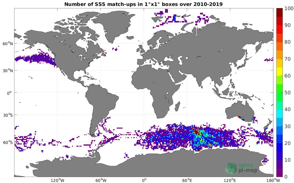
Figure 4: Number of SSS match-ups between Marine mammals SSS and the SMOS SSS L2 v700 (ESA) SSS product for the Global Ocean Pi-MEP region over 1°x1° boxes and for the full satellite product period.
