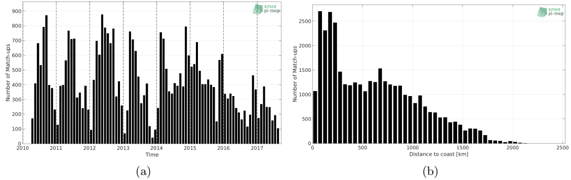
Figure 1: Number of match-ups between Sea mammals and SMOS SSS L2 v700 (ESA) SSS as a function of time (a) and as function of the distance to coast (b) over the Global Ocean Pi-MEP region and for the full satellite product period.
