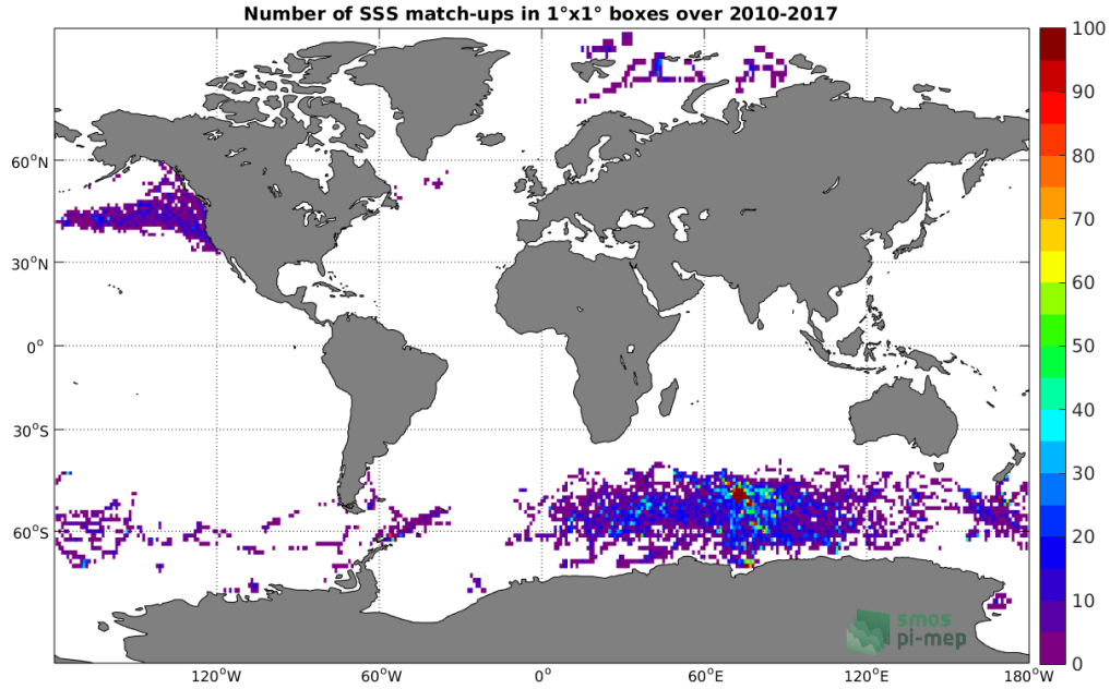
Figure 4: Number of SSS match-ups between Sea mammals SSS and the SMOS SSS L2 v700 (ESA) SSS product for the Global Ocean Pi-MEP region over 1^\circ \times 1^\circ boxes and for the full satellite product period.
