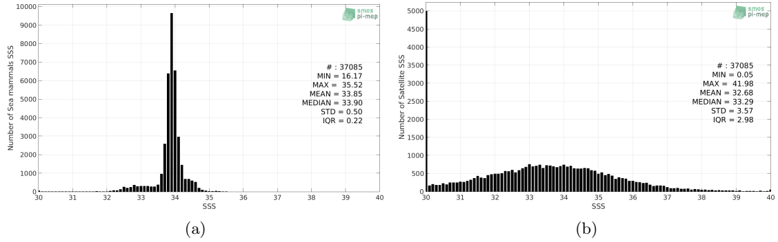
Figure 2: Histograms of SSS from Sea mammals (a) and SMOS SSS L2 v700 (ESA) (b) considering all match-up pairs per bins of 0.1 over the Global Ocean Pi-MEP region and for the full satellite product period.
