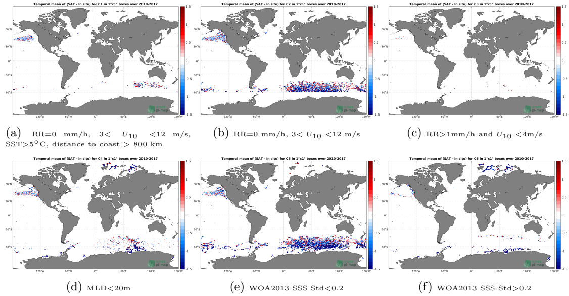
Figure 12: Temporal mean gridded over spatial boxes of size 1^\circ \times 1^\circ of \Delta SSS (SMOS SSS L2 v700 (ESA) - Sea mammals) for 6 different subdatasets corresponding to: RR=0 mm/h, 3 < U_{10} < 12 m/s, SST > 5^\circ C , distance to coast > 800 km (a), RR=0 mm/h, 3 < U_{10} < 12 m/s (b), RR > 1 mm/h and U_{10} < 4 m/s (c), MLD < 20 m (d), WOA2013 SSS Std < 0.2 (e), WOA2013 SSS Std > 0.2 (f).
