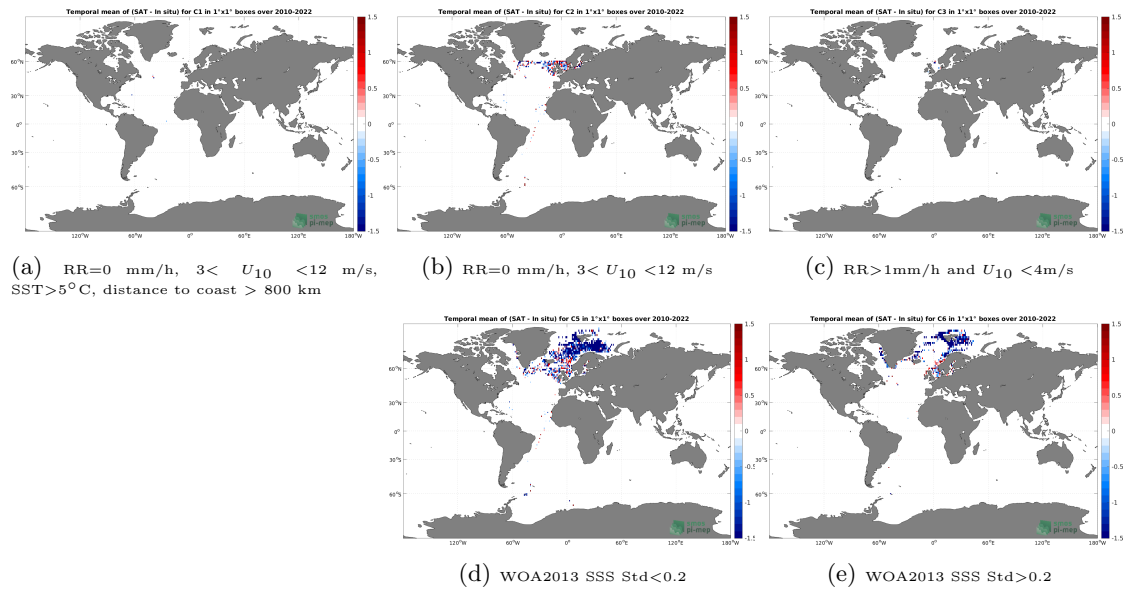
Figure 12: Temporal mean gridded over spatial boxes of size 1^\circ \times 1^\circ of \Delta SSS (SMOS SSS L2 v700 (ESA) - ICES) for 5 different subdatasets corresponding to:RR=0 mm/h, 3 < U_{10} < 12 m/s, SST > 5^\circ\text{C} , distance to coast > 800 km (a), RR=0 mm/h, 3 < U_{10} < 12 m/s (b), RR > 1 mm/h and U_{10} < 4 m/s (c), WOA2013 SSS Std < 0.2 (d), WOA2013 SSS Std > 0.2 (e).
