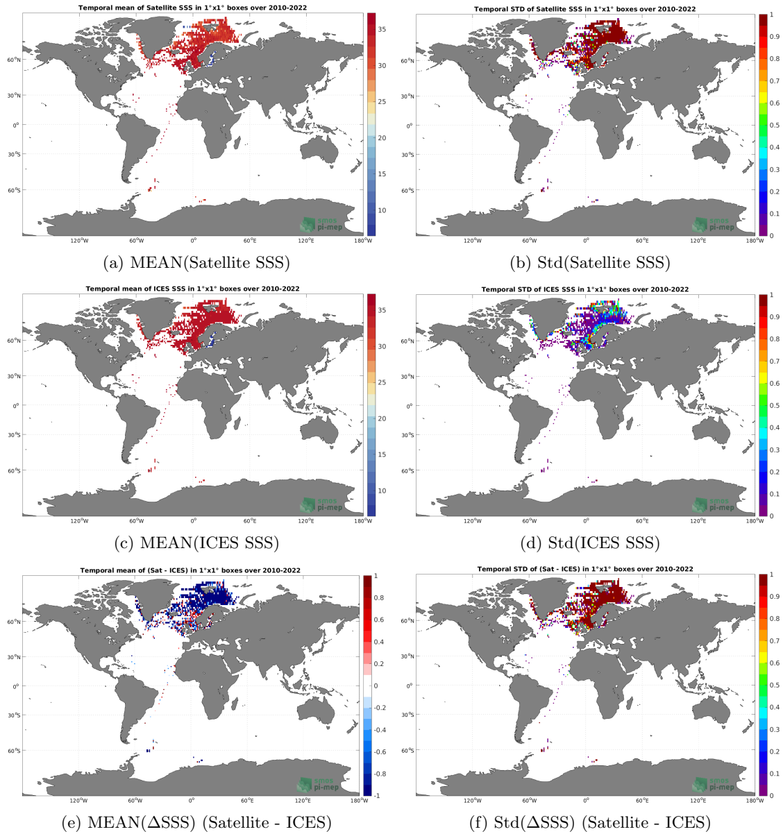
Figure 6: Temporal mean (left) and Std (right) of SSS from SMOS SSS L2 v700 (ESA) (top), ICES (middle), and of \Delta SSS (Satellite - ICES). Only match-up pairs are used to generate these maps.
