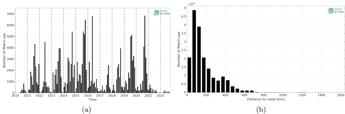
Figure 1: Number of match-ups between ICES and SMOS SSS L2 v700 (ESA) SSS as a function of time (a) and as function of the distance to coast (b) over the Global Ocean Pi-MEP region and for the full satellite product period.
