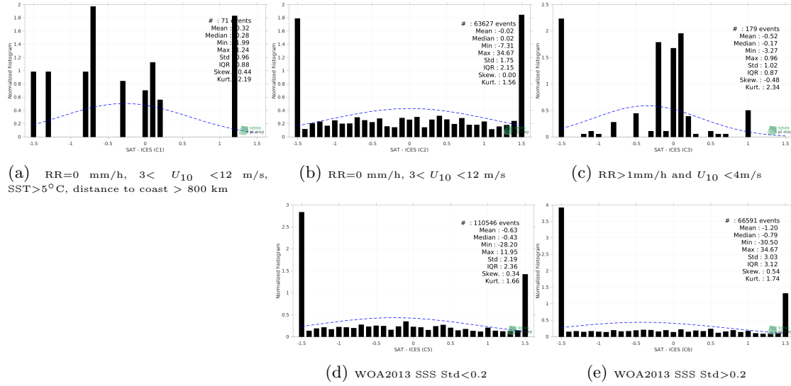
Figure 13: Normalized histogram of \Delta SSS (SMOS SSS L2 v700 (ESA) - ICES) for 5 different subdatasets corresponding to: RR=0 mm/h, 3 < U_{10} < 12 m/s, SST>5°C, distance to coast > 800 km (a), RR=0 mm/h, 3 < U_{10} < 12 m/s (b), RR>1mm/h and U_{10} < 4 m/s (c), WOA2013 SSS Std<0.2 (d), WOA2013 SSS Std>0.2 (e).
