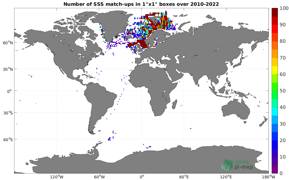
Figure 4: Number of SSS match-ups between ICES SSS and the SMOS SSS L2 v700 (ESA) SSS product for the Global Ocean Pi-MEP region over 1^\circ \times 1^\circ boxes and for the full satellite product period.
