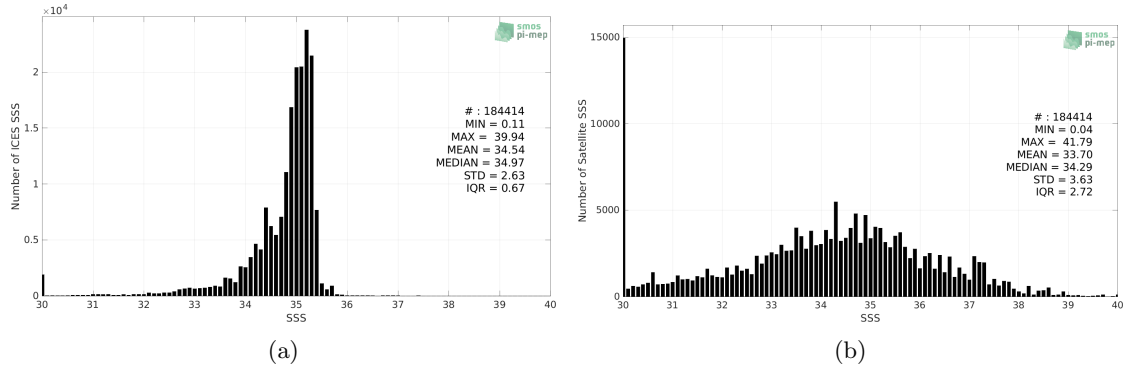
Figure 2: Histograms of SSS from ICES (a) and SMOS SSS L2 v700 (ESA) (b) considering all match-up pairs per bins of 0.1 over the Global Ocean Pi-MEP region and for the full satellite product period.
