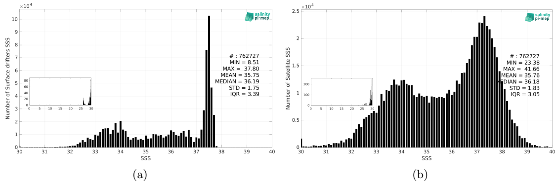
Figure 3: Histograms of SSS from Surface drifters (a) and SMOS SSS L2 v700 (ESA) (b) considering all match-up pairs per bins of 0.1 over the Global Ocean Pi-MEP region and for the full satellite product period.
