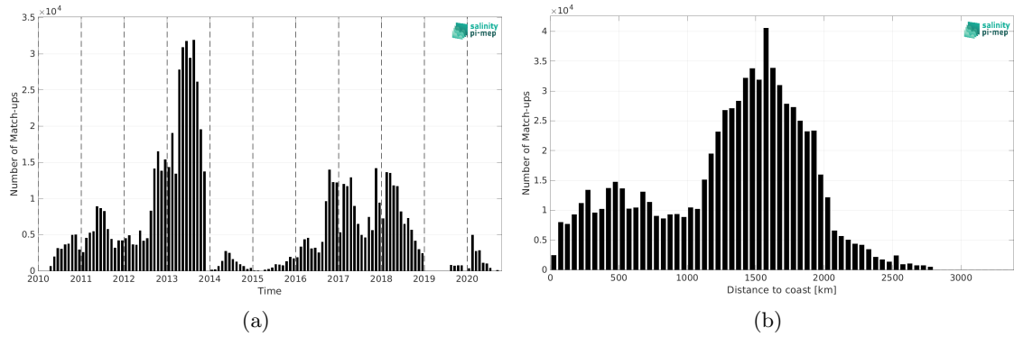
Figure 2: Number of match-ups between Surface drifters and SMOS SSS L2 v700 (ESA) SSS as a function of time (a) and as function of the distance to coast (b) over the Global Ocean Pi-MEP region and for the full satellite product period.
