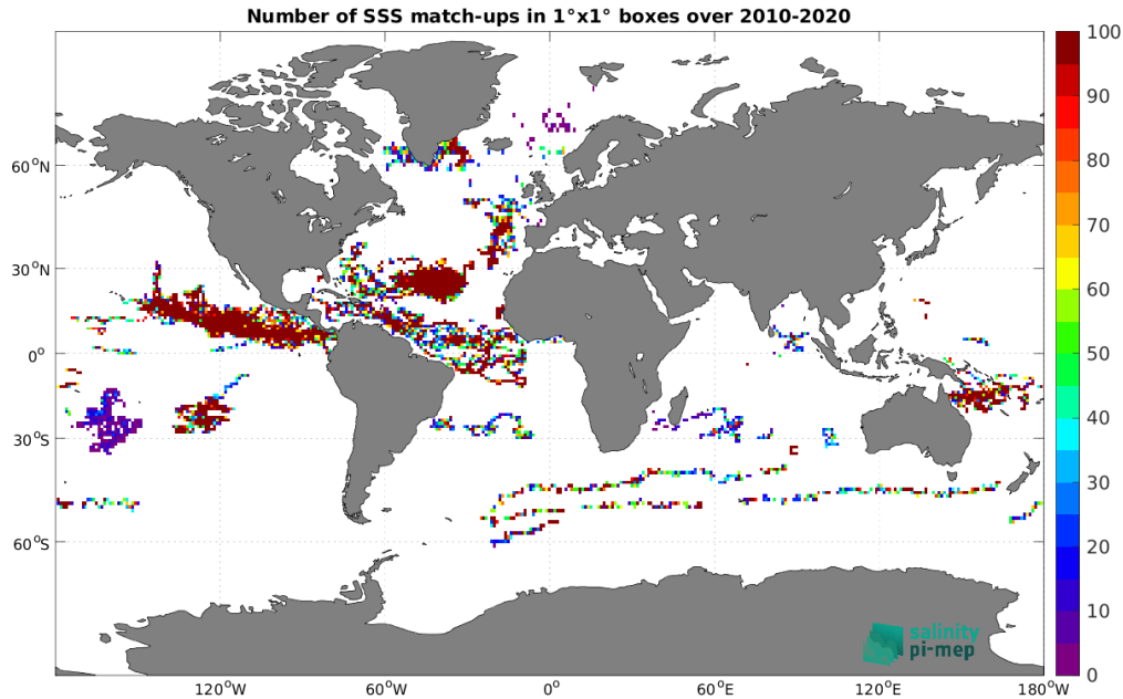
Figure 4: Number of SSS match-ups between Surface drifters SSS and the SMOS SSS L2 v700 (ESA) SSS product for the Global Ocean Pi-MEP region over 1^\circ \times 1^\circ boxes and for the full satellite product period.
