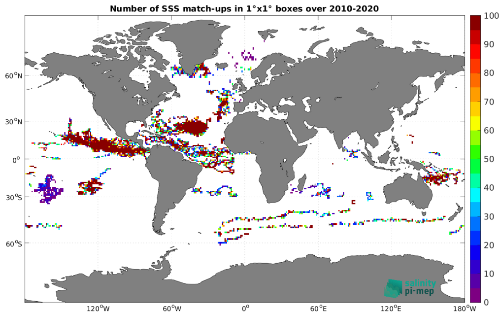
Figure 3: Number of SSS match-ups between Surface drifters SSS and the SMOS SSS L2 v700 (ESA) SSS product for the Global Ocean Pi-MEP region over 1^\circ \times 1^\circ boxes and for the full satellite product period.
