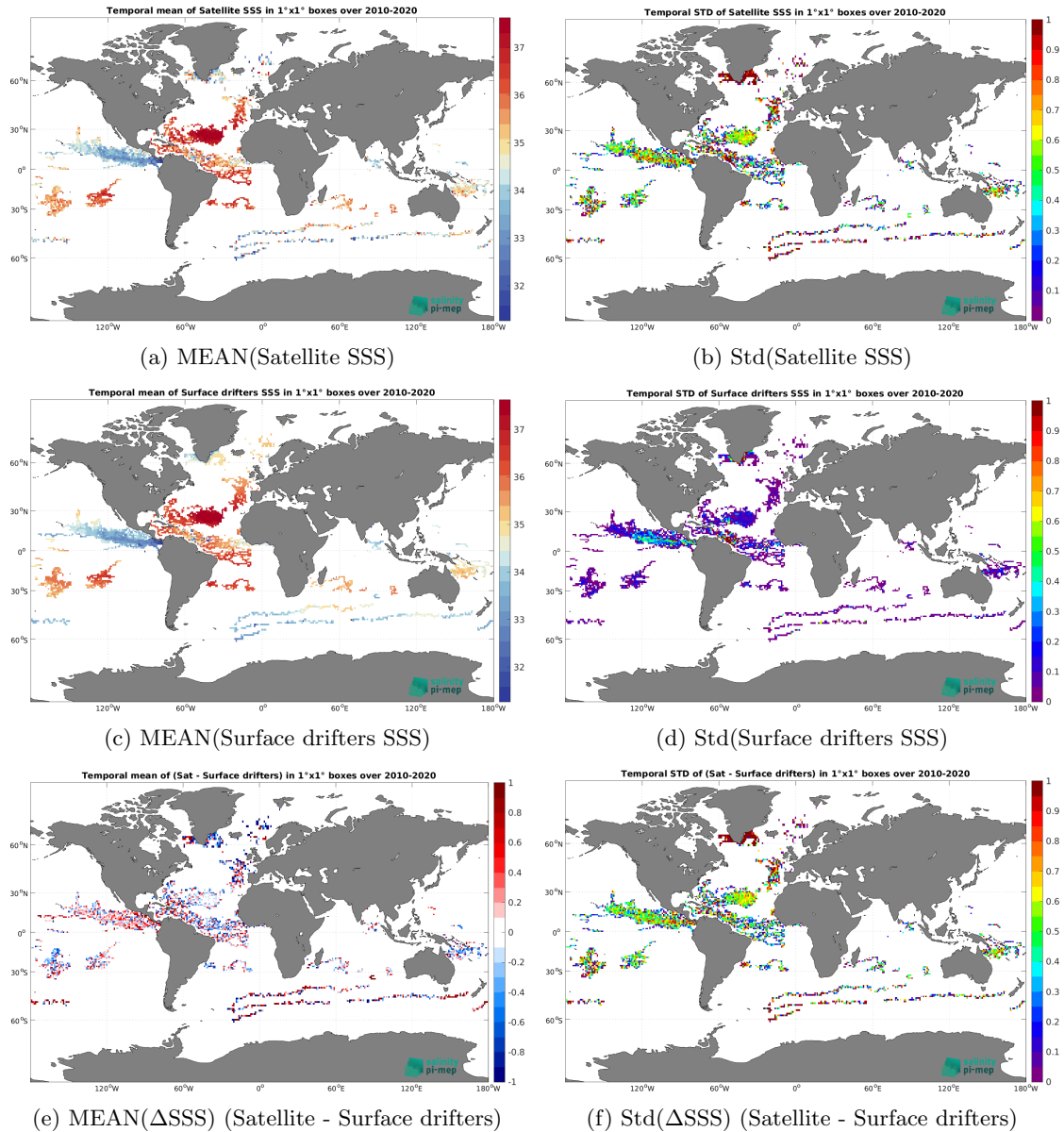
Figure 5: Temporal mean (left) and Std (right) of SSS from SMOS SSS L2 v700 (ESA) (top), Surface drifters (middle), and of \Delta SSS (Satellite - Surface drifters). Only match-up pairs are used to generate these maps.
