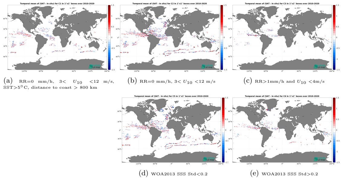
Figure 11: Temporal mean gridded over spatial boxes of size 1^\circ \times 1^\circ of \Delta SSS (SMOS SSS L2 v700 (ESA) - Surface drifters) for 5 different subdatasets corresponding to:RR=0 mm/h, 3 < U_{10} < 12 m/s, SST >5^\circ\text{C} , distance to coast > 800 km (a), RR=0 mm/h, 3 < U_{10} < 12 m/s (b), RR >1 mm/h and U_{10} < 4 m/s (c), WOA2013 SSS Std <0.2 (d), WOA2013 SSS Std >0.2 (e).
