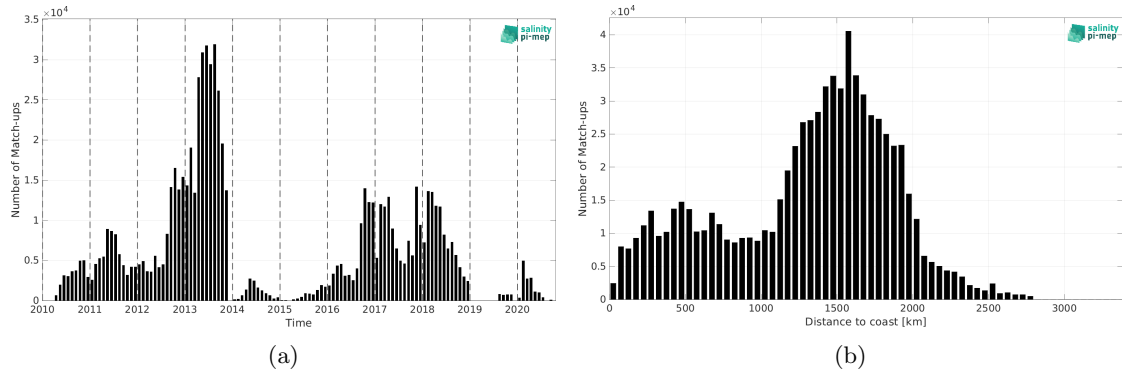
Figure 1: Number of match-ups between Surface drifters and SMOS SSS L2 v700 (ESA) SSS as a function of time (a) and as function of the distance to coast (b) over the Global Ocean Pi-MEP region and for the full satellite product period.
