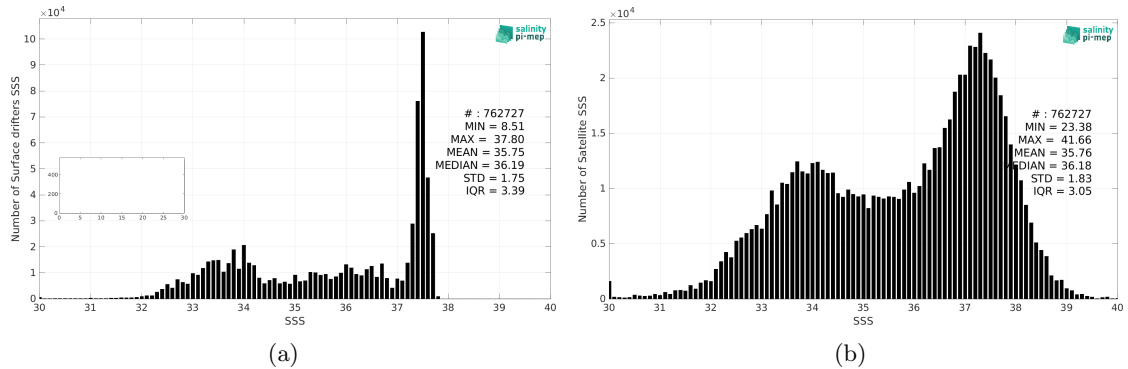
Figure 2: Histograms of SSS from Surface drifters (a) and SMOS SSS L2 v700 (ESA) (b) considering all match-up pairs per bins of 0.1 over the Global Ocean Pi-MEP region and for the full satellite product period.
