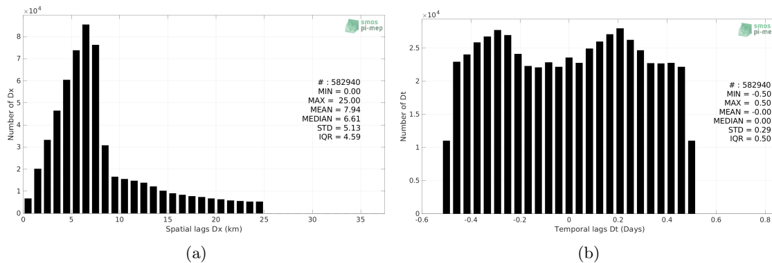
Figure 5: Histograms of the spatial (a) and temporal (b) lags between the location/time of the Argo measurement and the date of the corresponding SMOS SSS L2 v700 (ESA) SSS pixel.
