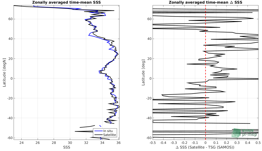
Figure 8: Left panel: Zonal mean SSS from SMOS SSS L2 v662 (ESA) satellite product (black) and from TSG (SAMOS) (blue). Right panel: Zonal mean of \Delta SSS (Satellite - TSG (SAMOS)) for all the collected Pi-MEP match-up pairs estimated over the full satellite product period.
