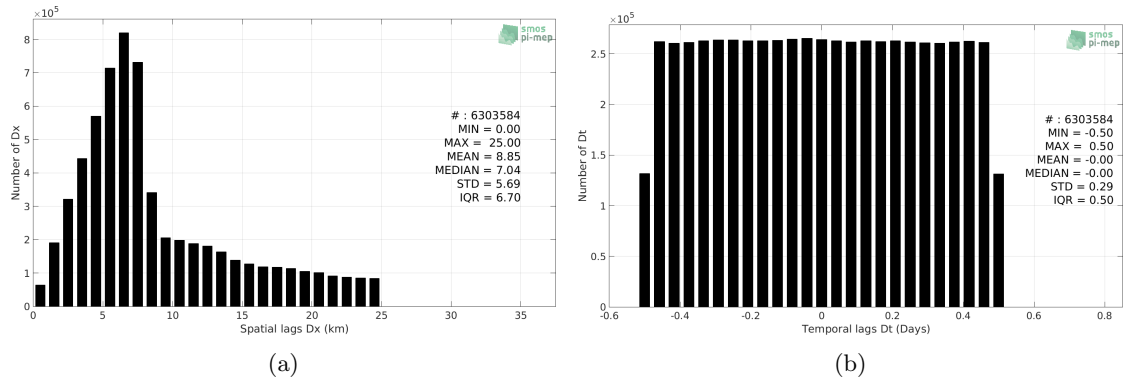
Figure 5: Histograms of the spatial (a) and temporal (b) lags between the location/time of the TSG (SAMOS) measurement and the date of the corresponding SMOS SSS L2 v662 (ESA) SSS pixel.
