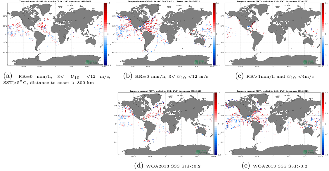
Figure 12: Temporal mean gridded over spatial boxes of size 1^\circ \times 1^\circ of \Delta SSS (SMOS SSS L2 v662 (ESA) - TSG (SAMOS)) for 5 different subdatasets corresponding to: RR=0 mm/h, 3 < U_{10} < 12 m/s, SST >5^\circ C, distance to coast > 800 km (a), RR=0 mm/h, 3 < U_{10} < 12 m/s (b), RR >1 mm/h and U_{10} < 4 m/s (c), WOA2013 SSS Std <0.2 (d), WOA2013 SSS Std >0.2 (e).
