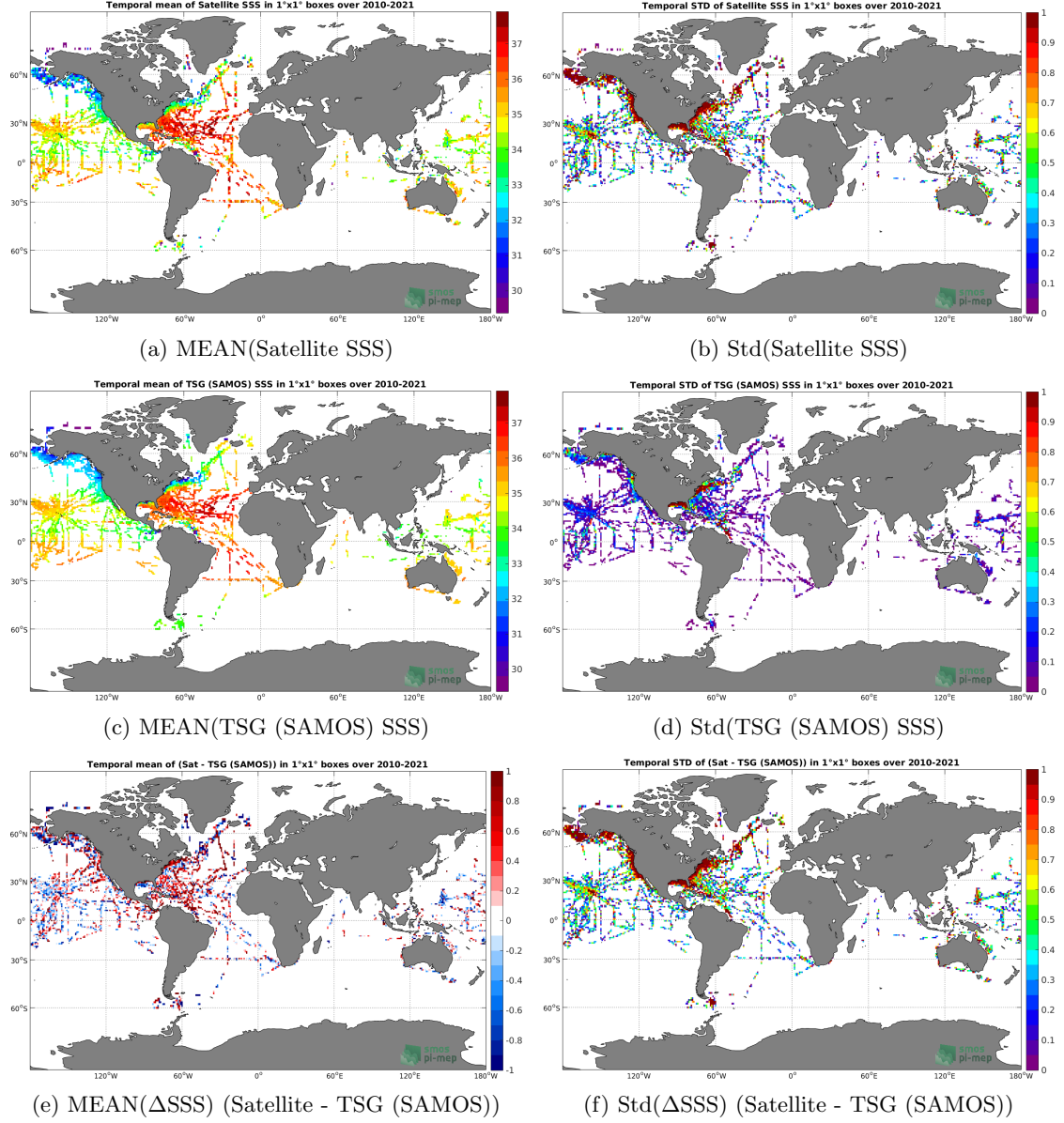
Figure 6: Temporal mean (left) and Std (right) of SSS from SMOS SSS L2 v662 (ESA) (top), TSG (SAMOS) (middle), and of \Delta SSS (Satellite - TSG (SAMOS)). Only match-up pairs are used to generate these maps.
