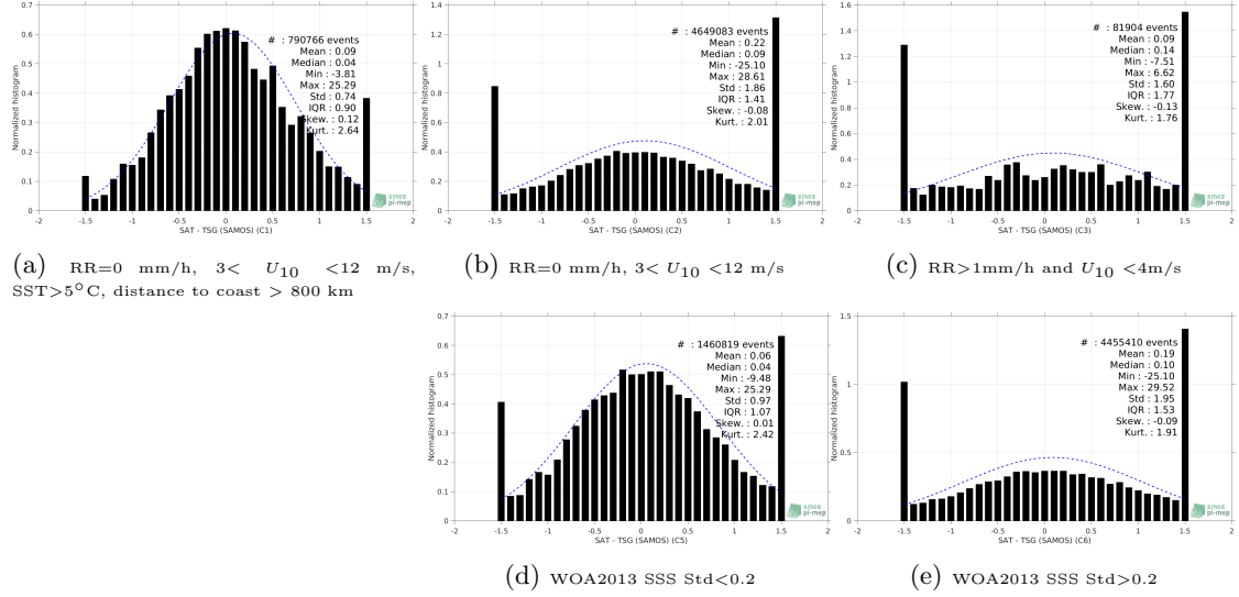
Figure 13: Normalized histogram of \Delta SSS (SMOS SSS L2 v662 (ESA) - TSG (SAMOS)) for 5 different subdatasets corresponding to: RR=0 mm/h, 3 < U_{10} < 12 m/s, SST>5°C, distance to coast > 800 km (a), RR=0 mm/h, 3 < U_{10} < 12 m/s (b), RR>1mm/h and U_{10} < 4 m/s (c), WOA2013 SSS Std<0.2 (d), WOA2013 SSS Std>0.2 (e).
