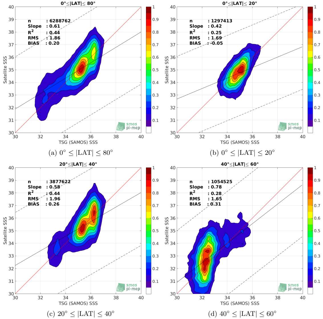
Figure 9: Contour maps of the concentration of SMOS SSS L2 v662 (ESA) SSS (y-axis) versus TSG (SAMOS) SSS (x-axis) at match-up pairs for different latitude bands. For each plot, the red line shows x=y . The black thin and dashed lines indicate a linear fit through the data cloud and the \pm 95\% confidence levels, respectively. The number match-up pairs n , the slope and R^2 coefficient of the linear fit, the root mean square (RMS) and the mean bias between satellite and in situ data are indicated for each latitude band in each plots.
