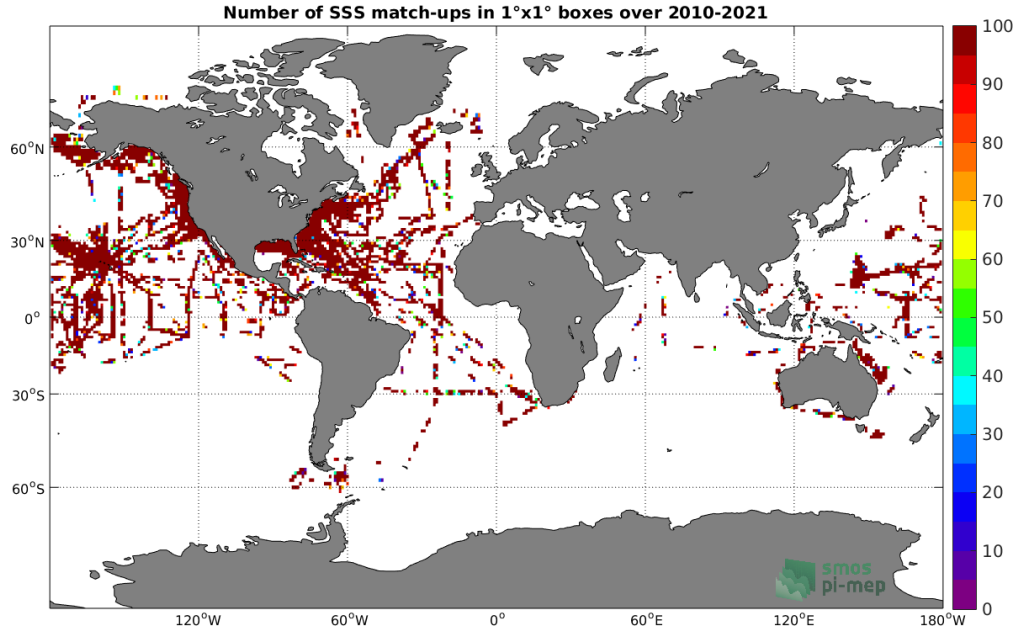
Figure 4: Number of SSS match-ups between TSG (SAMOS) SSS and the SMOS SSS L2 v662 (ESA) SSS product for the Global Ocean Pi-MEP region over 1^\circ \times 1^\circ boxes and for the full satellite product period.
