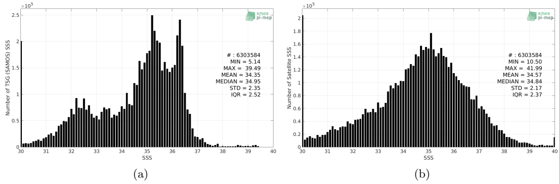
Figure 2: Histograms of SSS from TSG (SAMOS) (a) and SMOS SSS L2 v662 (ESA) (b) considering all match-up pairs per bins of 0.1 over the Global Ocean Pi-MEP region and for the full satellite product period.
