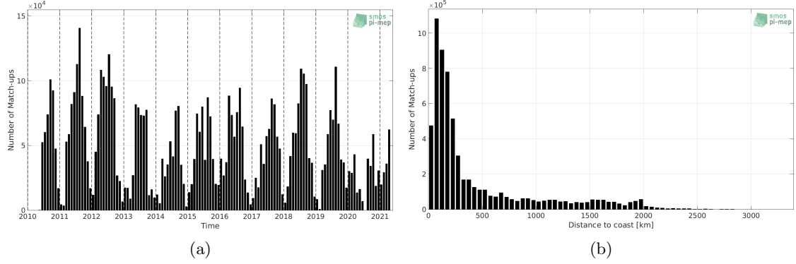
Figure 1: Number of match-ups between TSG (SAMOS) and SMOS SSS L2 v662 (ESA) SSS as a function of time (a) and as function of the distance to coast (b) over the Global Ocean Pi-MEP region and for the full satellite product period.
