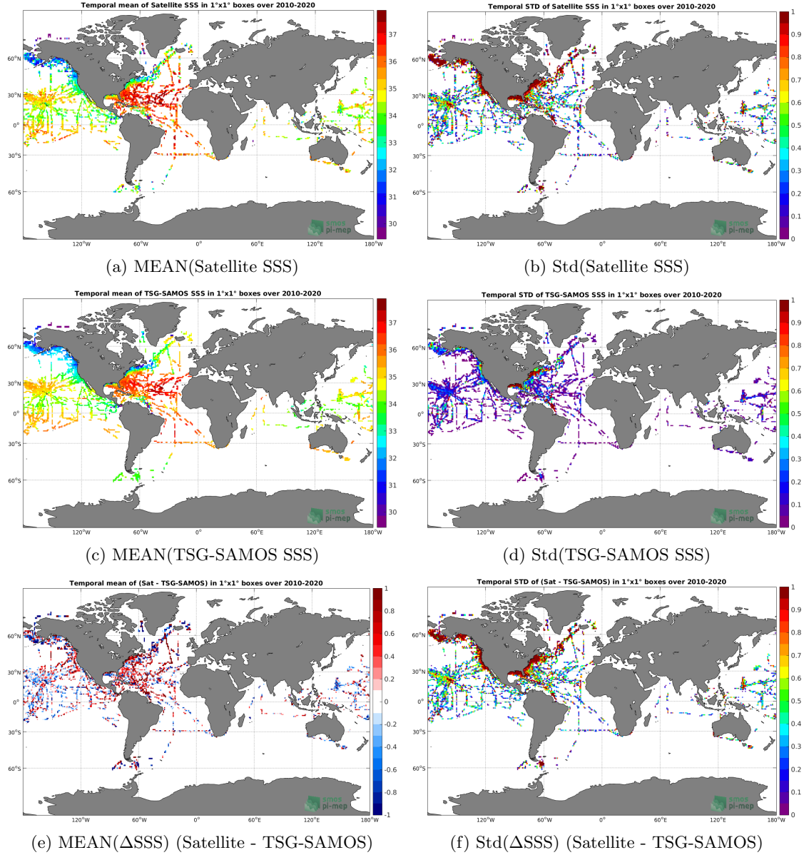
Figure 6: Temporal mean (left) and Std (right) of SSS from SMOS L2 v662 (ESA) (top), TSG-SAMOS (middle), and of \Delta SSS (Satellite - TSG-SAMOS). Only match-up pairs are used to generate these maps.
