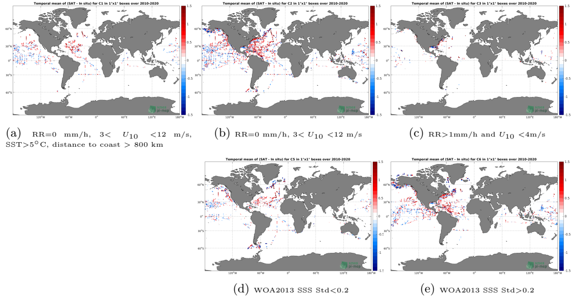
Figure 12: Temporal mean gridded over spatial boxes of size 1^\circ \times 1^\circ of \Delta SSS (SMOS L2 v662 (ESA) - TSG-SAMOS) for 5 different subdatasets corresponding to: RR=0 mm/h, 3 < U_{10} < 12 m/s, SST > 5^\circ C , distance to coast > 800 km (a), RR=0 mm/h, 3 < U_{10} < 12 m/s (b), RR > 1 mm/h and U_{10} < 4 m/s (c), WOA2013 SSS Std < 0.2 (d), WOA2013 SSS Std > 0.2 (e).
