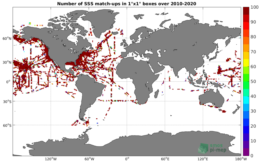
Figure 4: Number of SSS match-ups between TSG-SAMOS SSS and the SMOS L2 v662 (ESA) SSS product for the Global Ocean Pi-MEP region over 1°x1° boxes and for the full satellite product period.
