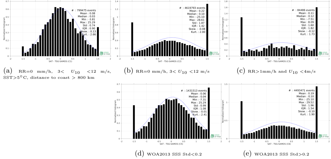
Figure 13: Normalized histogram of \Delta SSS (SMOS L2 v662 (ESA) - TSG-SAMOS) for 5 different subdatasets corresponding to: RR=0 mm/h, 3 < U_{10} < 12 m/s, SST>5°C, distance to coast > 800 km (a), RR=0 mm/h, 3 < U_{10} < 12 m/s (b), RR>1mm/h and U_{10} < 4 m/s (c), WOA2013 SSS Std<0.2 (d), WOA2013 SSS Std>0.2 (e).
