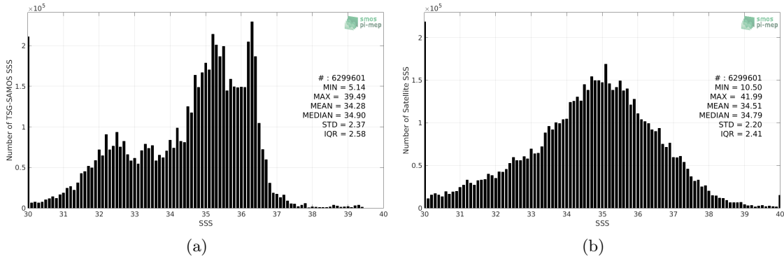
Figure 2: Histograms of SSS from TSG-SAMOS (a) and SMOS L2 v662 (ESA) (b) considering all match-up pairs per bins of 0.1 over the Global Ocean Pi-MEP region and for the full satellite product period.
