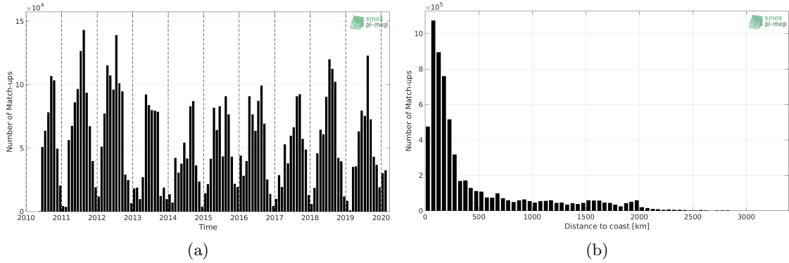
Figure 1: Number of match-ups between TSG-SAMOS and SMOS L2 v662 (ESA) SSS as a function of time (a) and as function of the distance to coast (b) over the Global Ocean Pi-MEP region and for the full satellite product period.
