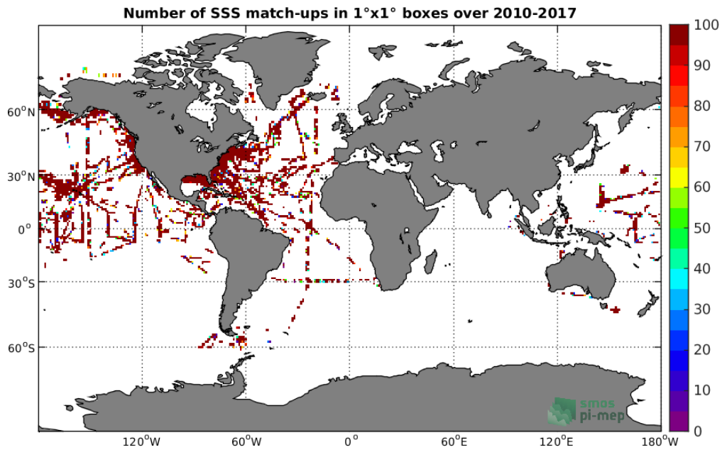
Figure 4: Number of SSS match-ups between TSG-SAMOS SSS and the SMOS-L2-DPGS-v662 SSS product for the Global Ocean Pi-MEP region over 1°x1° boxes and for the full satellite product period.
