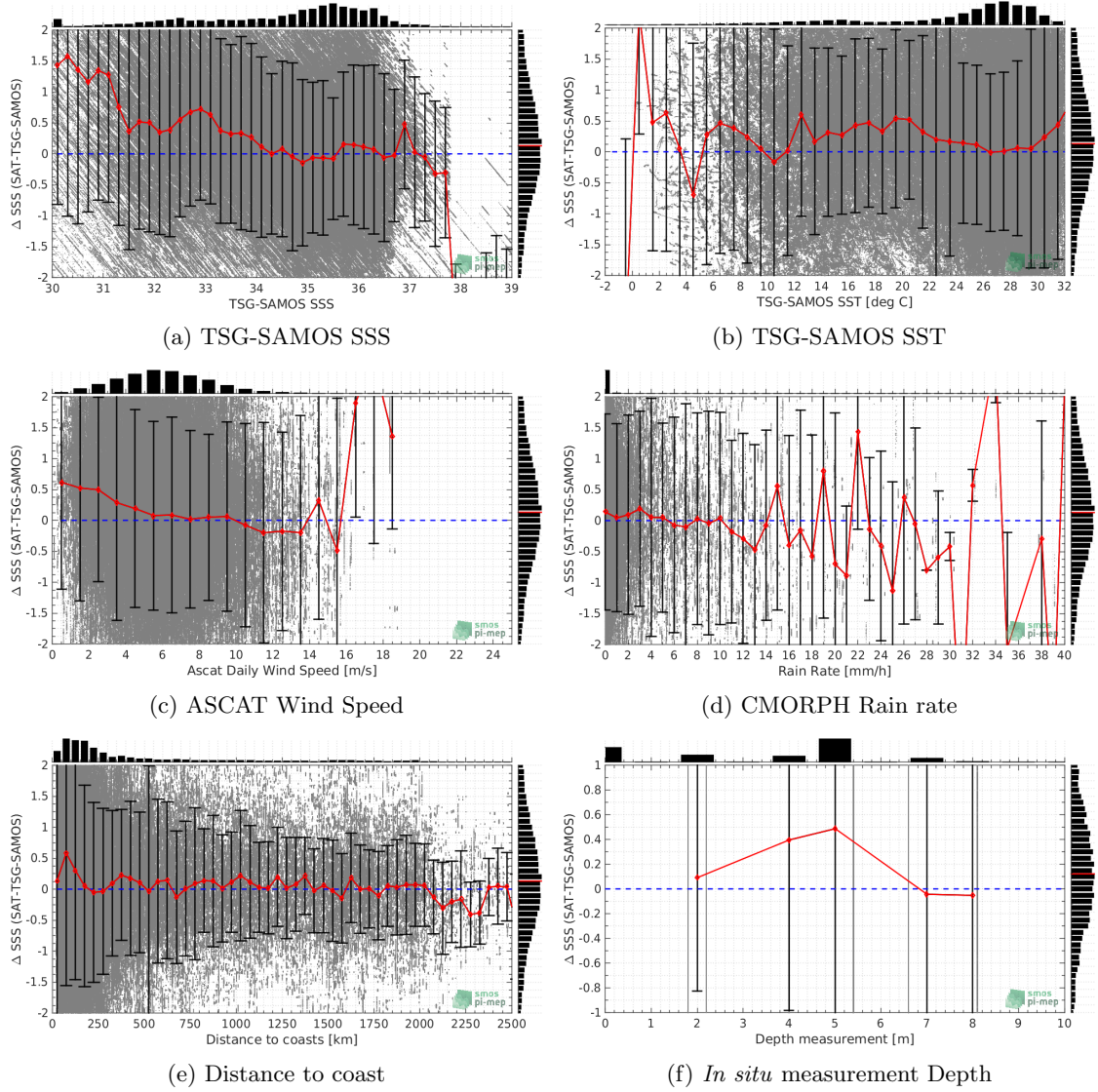
Figure 11: \Delta SSS (Satellite - TSG-SAMOS) sorted as function of TSG-SAMOS SSS values (a), TSG-SAMOS SST (b), ASCAT Wind speed (c), CMORPH rain rate (d), distance to coast (e) and in situ measurement depth (f). In all plots the median and Std of \Delta SSS for each bin is indicated by the red curves and black vertical thick bars ( \pm 1 Std)
