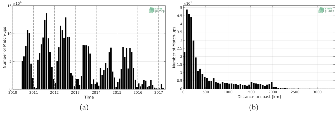
Figure 1: Number of match-ups between TSG-SAMOS and SMOS-L2-DPGS-v662 SSS as a function of time (a) and as function of the distance to coast (b) over the Global Ocean Pi-MEP region and for the full satellite product period.
