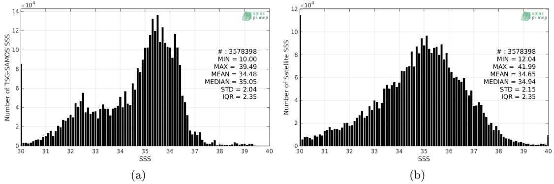
Figure 2: Histograms of SSS from TSG-SAMOS (a) and SMOS-L2-DPGS-v662 (b) considering all match-up pairs per bins of 0.1 over the Global Ocean Pi-MEP region and for the full satellite product period.
