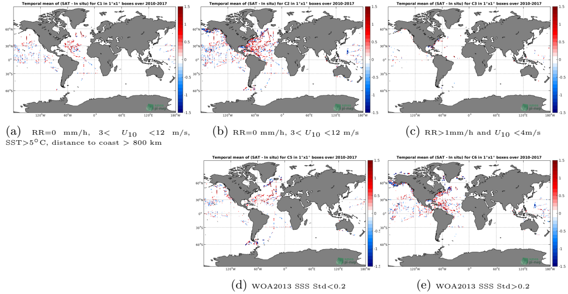
Figure 12: Temporal mean gridded over spatial boxes of size 1^\circ \times 1^\circ of \Delta SSS (SMOS-L2-DPGS-v662 - TSG-SAMOS) for 5 different subdatasets corresponding to:RR=0 mm/h, 3 < U_{10} < 12 m/s, SST >5^\circ C, distance to coast > 800 km (a), RR=0 mm/h, 3 < U_{10} < 12 m/s (b), RR >1 mm/h and U_{10} < 4 m/s (c), WOA2013 SSS Std <0.2 (d), WOA2013 SSS Std >0.2 (e).
