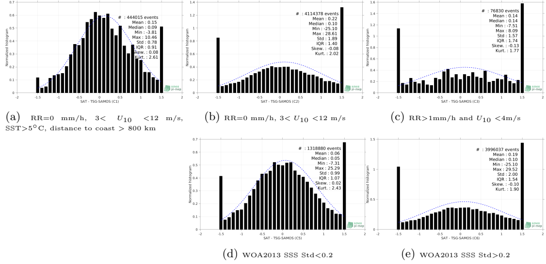
Figure 13: Normalized histogram of \Delta SSS (SMOS-L2-DPGS-v662 - TSG-SAMOS) for 5 different subdatasets corresponding to: RR=0 mm/h, 3 < U_{10} < 12 m/s, SST>5°C, distance to coast > 800 km (a), RR=0 mm/h, 3 < U_{10} < 12 m/s (b), RR>1mm/h and U_{10} < 4 m/s (c), WOA2013 SSS Std<0.2 (d), WOA2013 SSS Std>0.2 (e).
