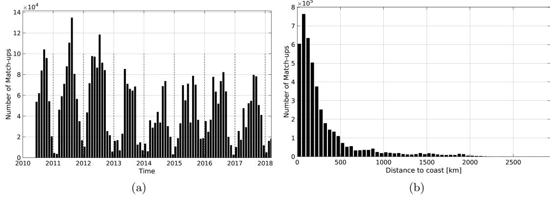
Figure 1: Number of match-ups between TSG-SAMOS and SMOS-L2-DPGS-v662 SSS as a function of time (a) and as function of the distance to coast (b) over the Global Ocean Pi-MEP region and for the full satellite product period.
