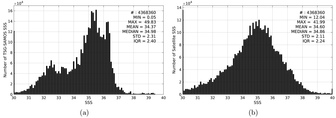
Figure 2: Histograms of SSS from TSG-SAMOS (a) and SMOS-L2-DPGS-v662 (b) considering all match-up pairs per bins of 0.1 over the Global Ocean Pi-MEP region and for the full satellite product period.
