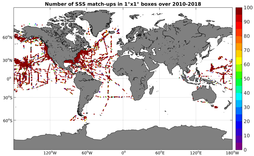
Figure 4: Number of SSS match-ups between TSG-SAMOS SSS and the SMOS-L2-DPGS-v662 SSS product for the Global Ocean Pi-MEP region over 1°x1° boxes and for the full satellite product period.
