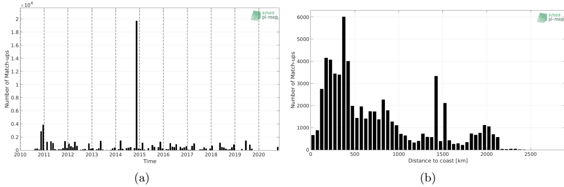
Figure 1: Number of match-ups between TSG (Polarstern) and SMOS SSS L2 v662 (ESA) SSS as a function of time (a) and as function of the distance to coast (b) over the Global Ocean Pi-MEP region and for the full satellite product period.
