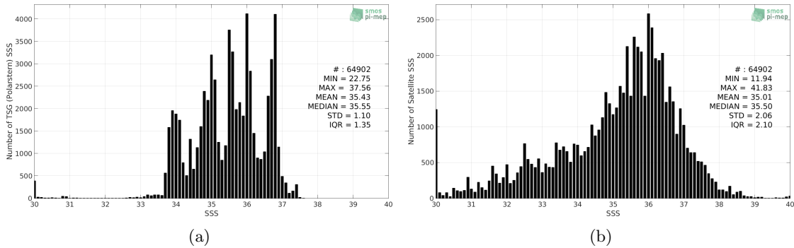
Figure 2: Histograms of SSS from TSG (Polarstern) (a) and SMOS SSS L2 v662 (ESA) (b) considering all match-up pairs per bins of 0.1 over the Global Ocean Pi-MEP region and for the full satellite product period.
