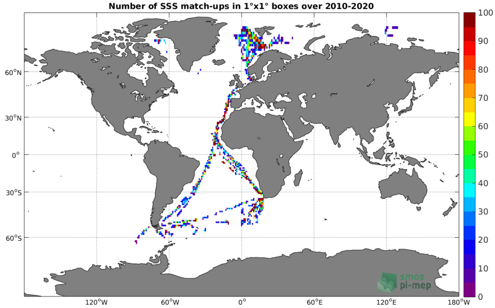
Figure 4: Number of SSS match-ups between TSG (Polarstern) SSS and the SMOS SSS L2 v662 (ESA) SSS product for the Global Ocean Pi-MEP region over 1^\circ \times 1^\circ boxes and for the full satellite product period.
