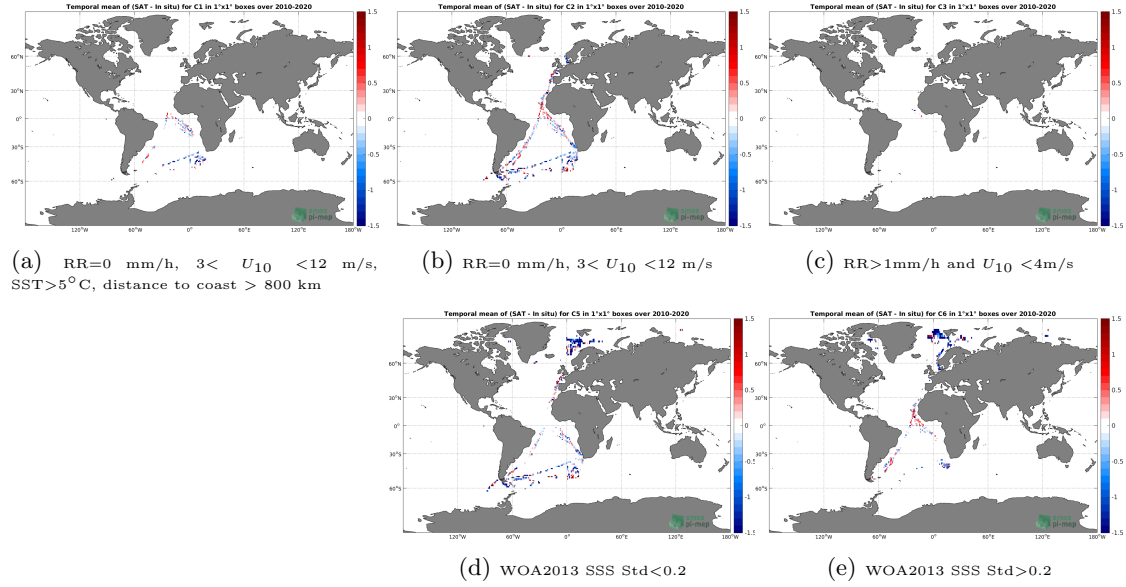
Figure 12: Temporal mean gridded over spatial boxes of size 1^\circ \times 1^\circ of \Delta SSS (SMOS SSS L2 v662 (ESA) - TSG (Polarstern)) for 5 different subdatasets corresponding to: RR=0 mm/h, 3 < U_{10} < 12 m/s, SST >5^\circ\text{C} , distance to coast > 800 km (a), RR=0 mm/h, 3 < U_{10} < 12 m/s (b), RR >1 mm/h and U_{10} < 4 m/s (c), WOA2013 SSS Std <0.2 (d), WOA2013 SSS Std >0.2 (e).
