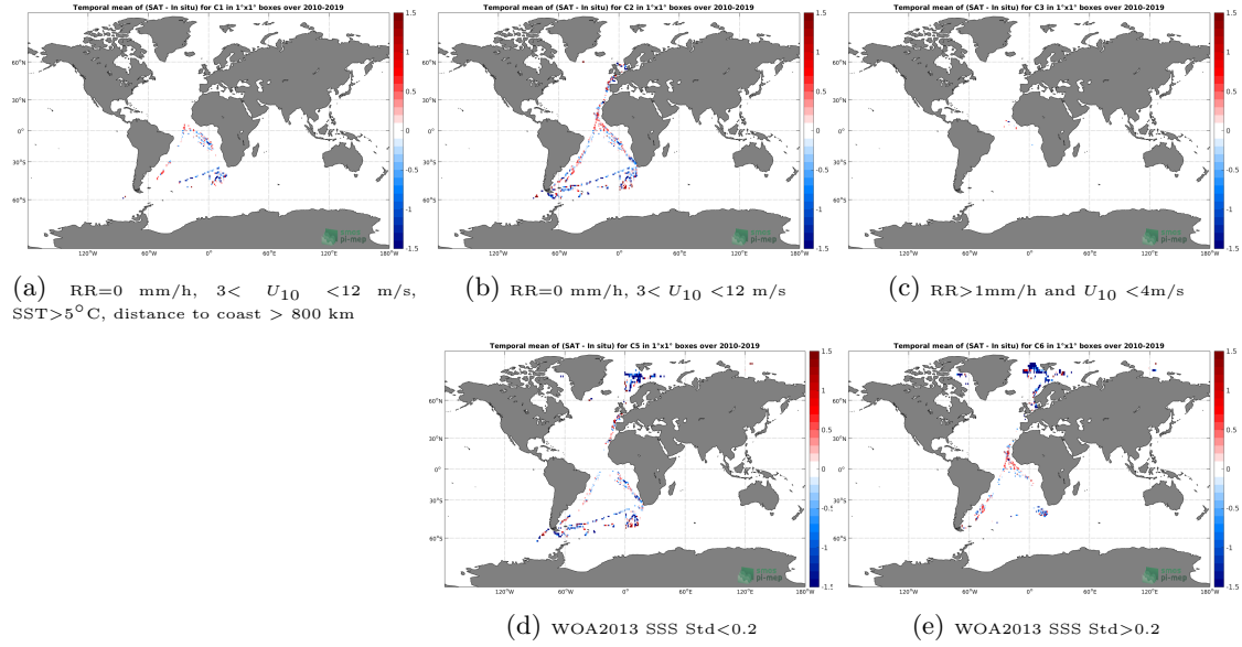
Figure 12: Temporal mean gridded over spatial boxes of size 1^\circ \times 1^\circ of \Delta SSS (SMOS L2 v662 (ESA) - TSG-POLARSTERN) for 5 different subdatasets corresponding to: RR=0 mm/h, 3 < U_{10} < 12 m/s, SST >5^\circ\text{C} , distance to coast > 800 km (a), RR=0 mm/h, 3 < U_{10} < 12 m/s (b), RR >1 mm/h and U_{10} < 4 m/s (c), WOA2013 SSS Std <0.2 (d), WOA2013 SSS Std >0.2 (e).
