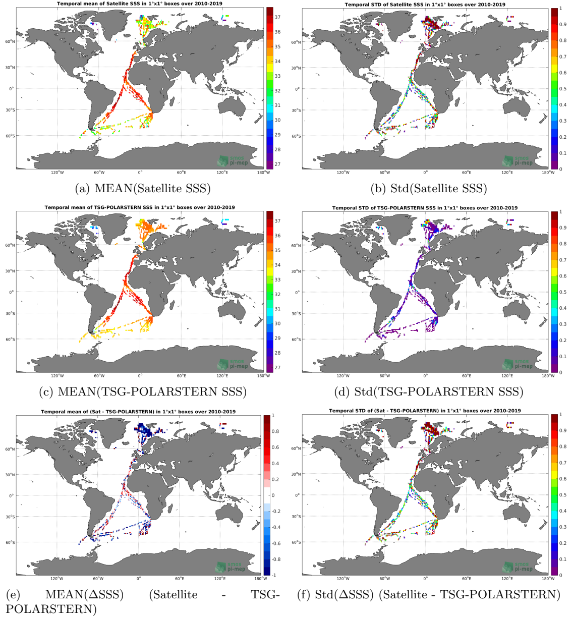
Figure 6: Temporal mean (left) and Std (right) of SSS from SMOS L2 v662 (ESA) (top), TSG-POLARSTERN (middle), and of \Delta SSS (Satellite - TSG-POLARSTERN). Only match-up pairs are used to generate these maps.
