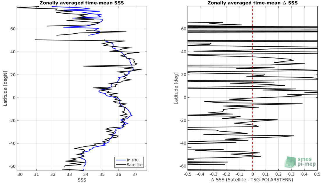
Figure 8: Left panel: Zonal mean SSS from SMOS L2 v662 (ESA) satellite product (black) and from TSG-POLARSTERN (blue). Right panel: Zonal mean of \Delta SSS (Satellite - TSG-POLARSTERN) for all the collected Pi-MEP match-up pairs estimated over the full satellite product period.
