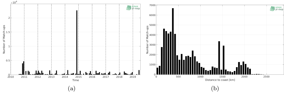
Figure 1: Number of match-ups between TSG-POLARSTERN and SMOS L2 v662 (ESA) SSS as a function of time (a) and as function of the distance to coast (b) over the Global Ocean Pi-MEP region and for the full satellite product period.
