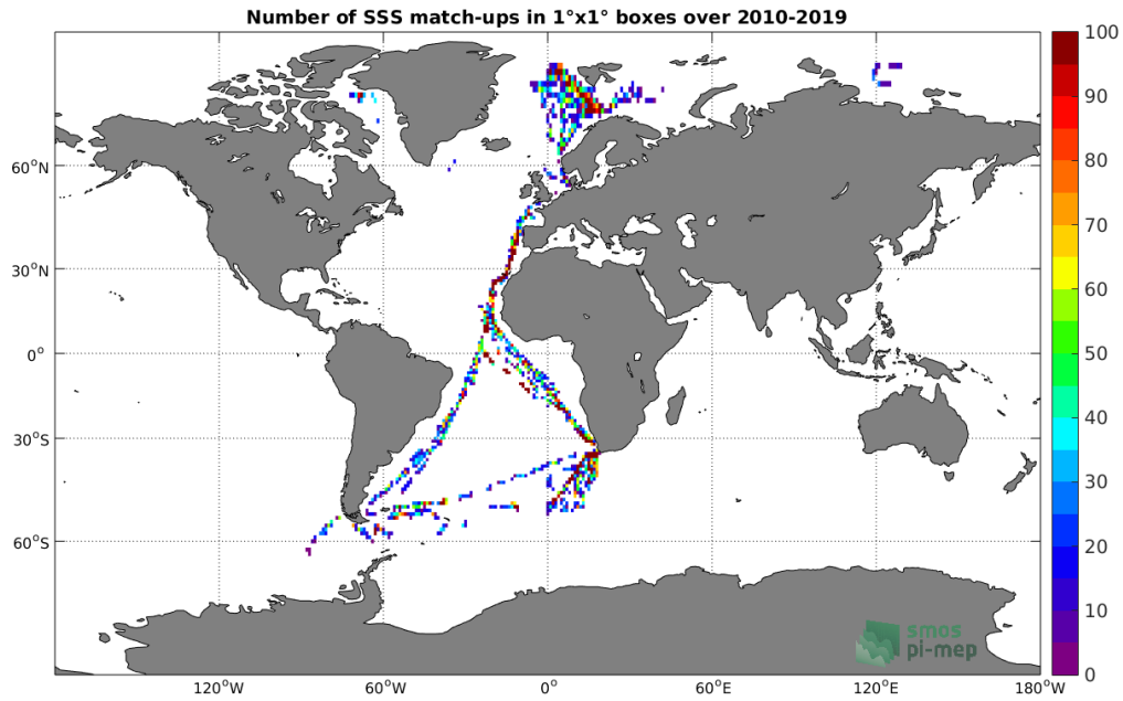
Figure 4: Number of SSS match-ups between TSG-POLARSTERN SSS and the SMOS L2 v662 (ESA) SSS product for the Global Ocean Pi-MEP region over 1^\circ \times 1^\circ boxes and for the full satellite product period.
