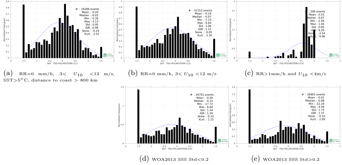
Figure 13: Normalized histogram of \Delta SSS (SMOS L2 v662 (ESA) - TSG-POLARSTERN) for 5 different subdatasets corresponding to: RR=0 mm/h, 3 < U_{10} < 12 m/s, SST>5°C, distance to coast > 800 km (a), RR=0 mm/h, 3 < U_{10} < 12 m/s (b), RR>1mm/h and U_{10} < 4 m/s (c), WOA2013 SSS Std<0.2 (d), WOA2013 SSS Std>0.2 (e).
