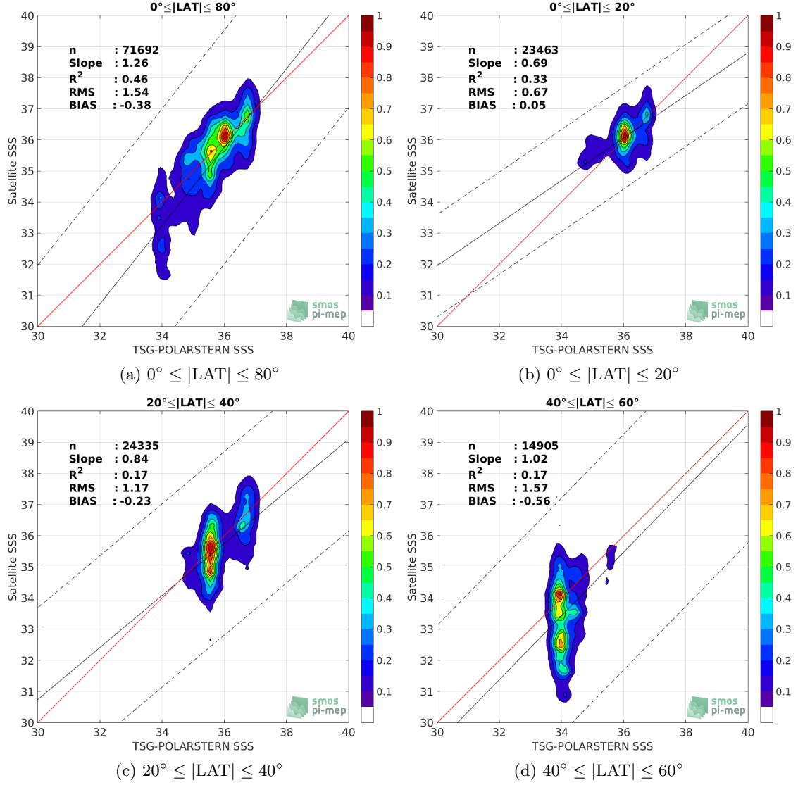
Figure 9: Contour maps of the concentration of SMOS L2 v662 (ESA) SSS (y-axis) versus TSG-POLARSTERN SSS (x-axis) at match-up pairs for different latitude bands. For each plot, the red line shows x=y . The black thin and dashed lines indicate a linear fit through the data cloud and the \pm 95\% confidence levels, respectively. The number match-up pairs n , the slope and R^2 coefficient of the linear fit, the root mean square (RMS) and the mean bias between satellite and in situ data are indicated for each latitude band in each plots.
