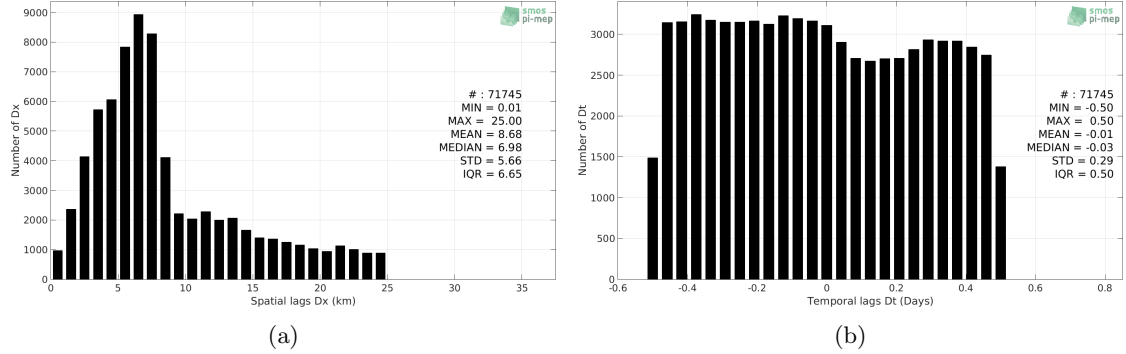
Figure 5: Histograms of the spatial (a) and temporal (b) lags between the time of the TSG-POLARSTERN measurements and the date of the corresponding SMOS L2 v662 (ESA) SSS product.
