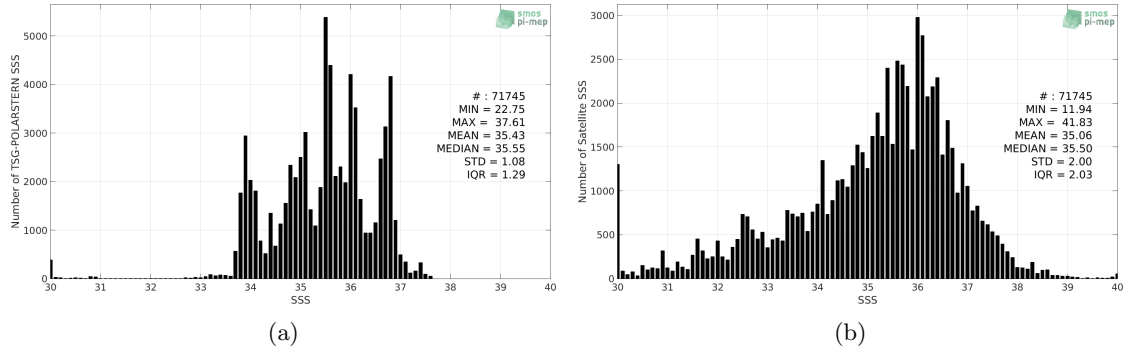
Figure 2: Histograms of SSS from TSG-POLARSTERN (a) and SMOS L2 v662 (ESA) (b) considering all match-up pairs per bins of 0.1 over the Global Ocean Pi-MEP region and for the full satellite product period.
