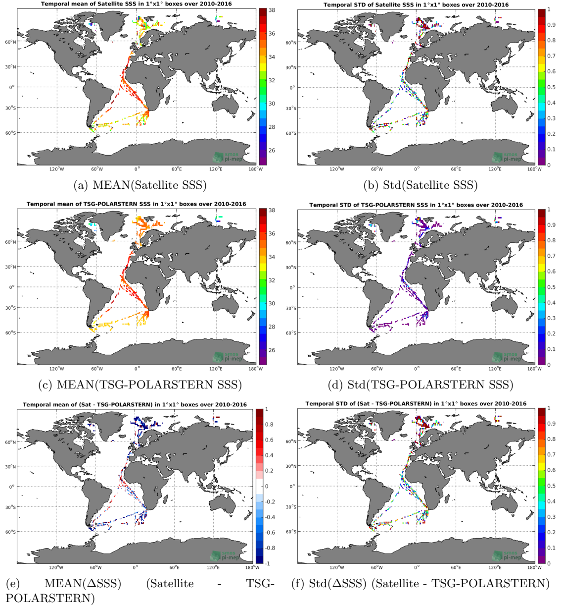
Figure 6: Temporal mean (left) and Std (right) of SSS from SMOS-L2-DPGS-v662 (top), TSG-POLARSTERN (middle), and of \Delta SSS (Satellite - TSG-POLARSTERN). Only match-up pairs are used to generate these maps.
