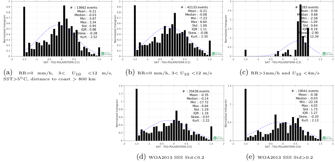
Figure 13: Normalized histogram of \Delta SSS (SMOS-L2-DPGS-v662 - TSG-POLARSTERN) for 5 different subdatasets corresponding to: RR=0 mm/h, 3 < U_{10} < 12 m/s, SST>5°C, distance to coast > 800 km (a), RR=0 mm/h, 3 < U_{10} < 12 m/s (b), RR>1mm/h and U_{10} < 4 m/s (c), WOA2013 SSS Std<0.2 (d), WOA2013 SSS Std>0.2 (e).
