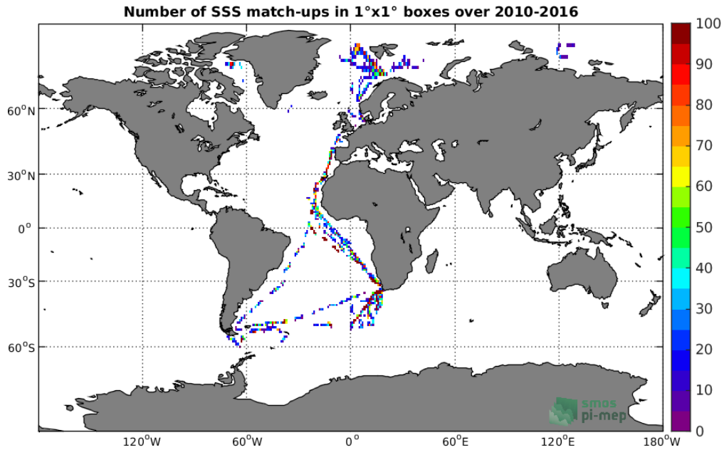
Figure 4: Number of SSS match-ups between TSG-POLARSTERN SSS and the SMOS-L2-DPGS-v662 SSS product for the Global Ocean Pi-MEP region over 1°x1° boxes and for the full satellite product period.
