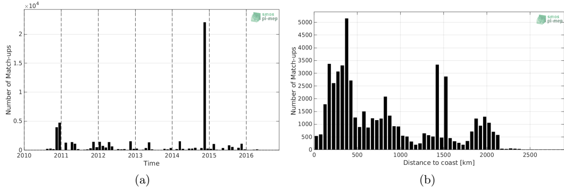
Figure 1: Number of match-ups between TSG-POLARSTERN and SMOS-L2-DPGS-v662 SSS as a function of time (a) and as function of the distance to coast (b) over the Global Ocean Pi-MEP region and for the full satellite product period.
