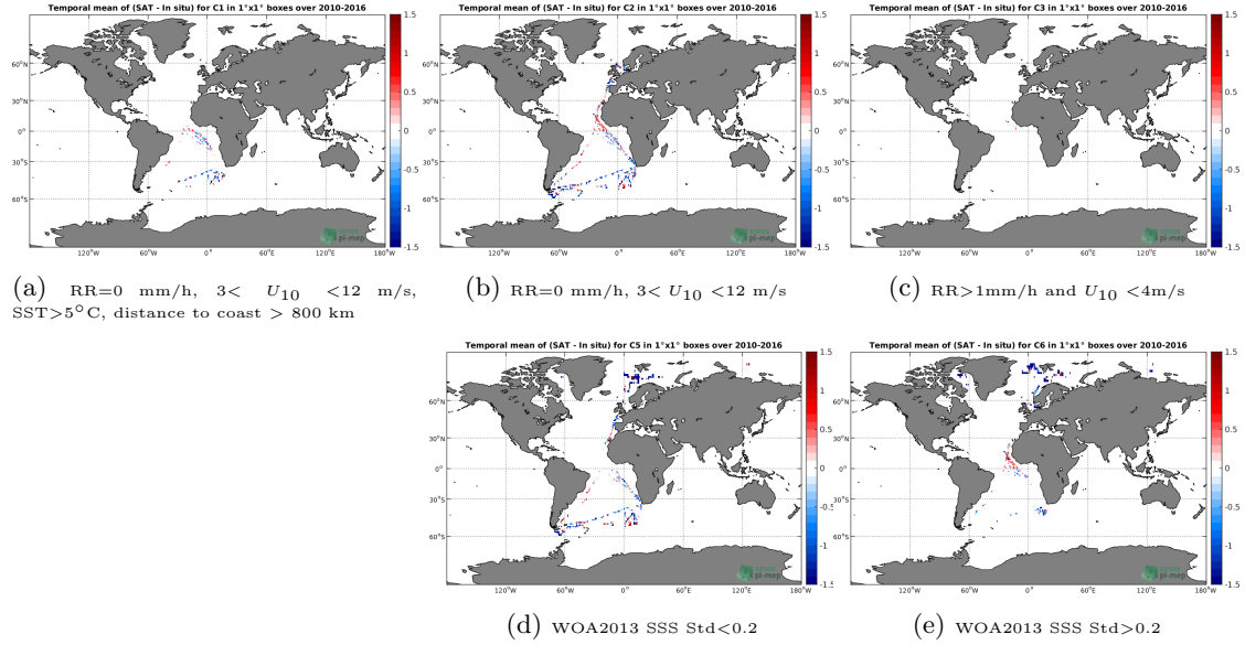
Figure 12: Temporal mean gridded over spatial boxes of size 1^\circ \times 1^\circ of \Delta SSS (SMOS-L2-DPGS-v662 - TSG-POLARSTERN) for 5 different subdatasets corresponding to: RR=0 mm/h, 3 < U_{10} < 12 m/s, SST > 5^\circ C , distance to coast > 800 km (a), RR=0 mm/h, 3 < U_{10} < 12 m/s (b), RR > 1 mm/h and U_{10} < 4 m/s (c), WOA2013 SSS Std < 0.2 (d), WOA2013 SSS Std > 0.2 (e).
