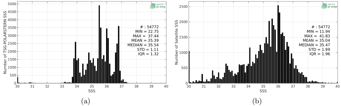
Figure 2: Histograms of SSS from TSG-POLARSTERN (a) and SMOS-L2-DPGS-v662 (b) considering all match-up pairs per bins of 0.1 over the Global Ocean Pi-MEP region and for the full satellite product period.
