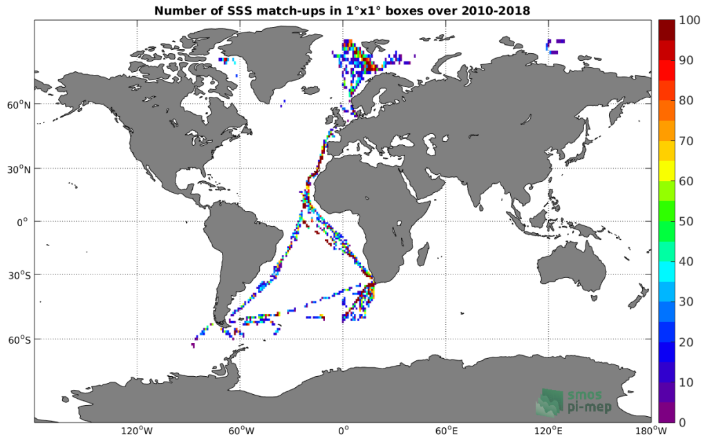
Figure 4: Number of SSS match-ups between TSG-POLARSTERN SSS and the SMOS-L2-DPGS-v662 SSS product for the Global Ocean Pi-MEP region over 1^\circ \times 1^\circ boxes and for the full satellite product period.
