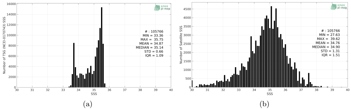
Figure 2: Histograms of SSS from TSG (NCEI-0170743) (a) and SMOS SSS L2 v662 (ESA) (b) considering all match-up pairs per bins of 0.1 over the Global Ocean Pi-MEP region and for the full satellite product period.
