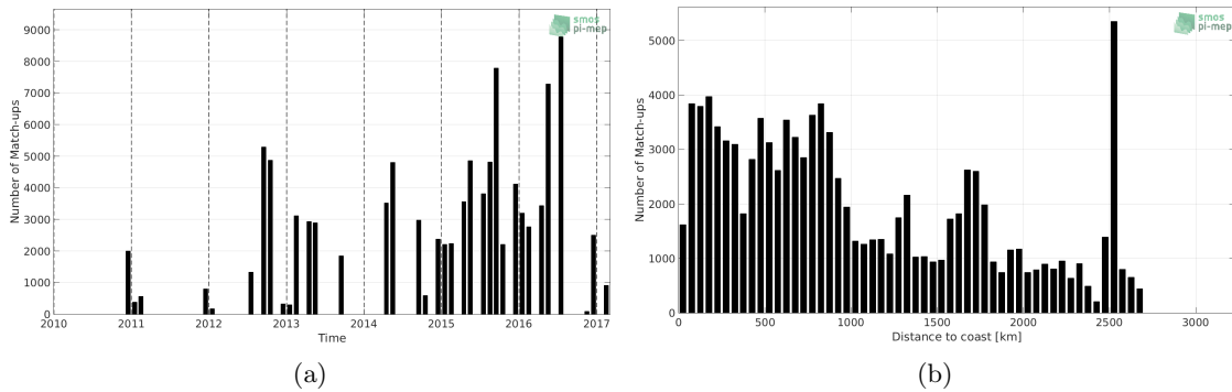
Figure 1: Number of match-ups between TSG (NCEI-0170743) and SMOS SSS L2 v662 (ESA) SSS as a function of time (a) and as function of the distance to coast (b) over the Global Ocean Pi-MEP region and for the full satellite product period.
