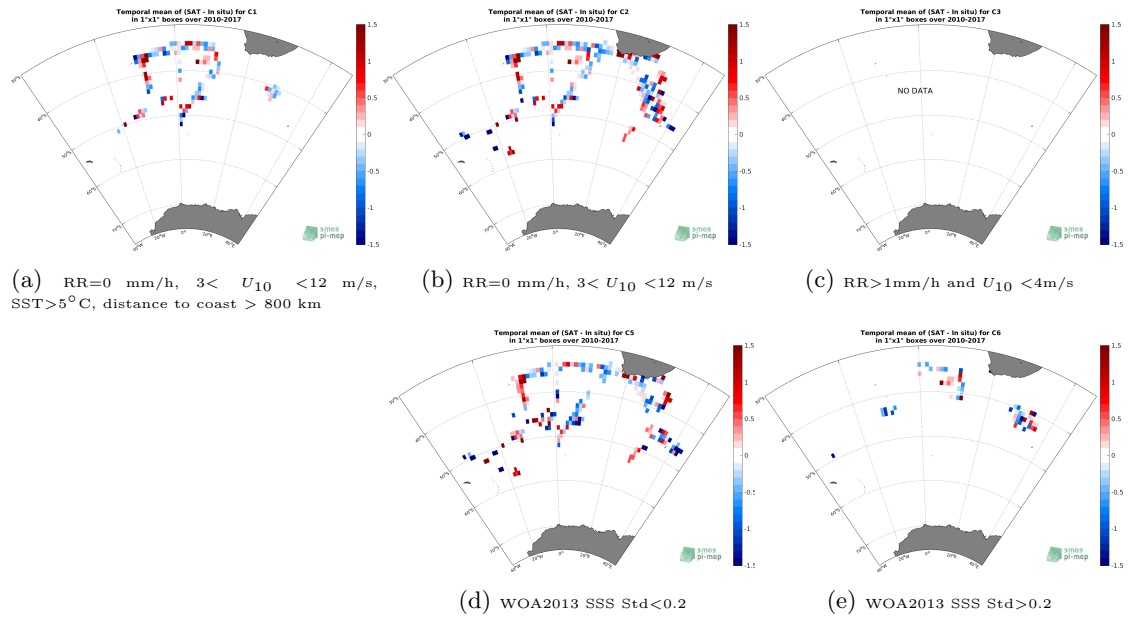
Figure 12: Temporal mean gridded over spatial boxes of size 1^\circ \times 1^\circ of \Delta SSS (SMOS SSS L2 v662 (ESA) - TSG (NCEI-0170743)) for 5 different subdatasets corresponding to:RR=0 mm/h, 3 < U_{10} < 12 m/s, SST >5^\circ C, distance to coast > 800 km (a), RR=0 mm/h, 3 < U_{10} < 12 m/s (b), RR >1 mm/h and U_{10} < 4 m/s (c), WOA2013 SSS Std <0.2 (d), WOA2013 SSS Std >0.2 (e).
