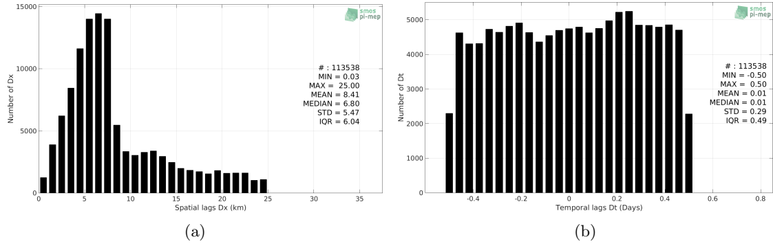
Figure 5: Histograms of the spatial (a) and temporal (b) lags between the time of the TSG (NCEI-0170743) measurements and the date of the corresponding SMOS SSS L2 v662 (ESA) SSS product.
