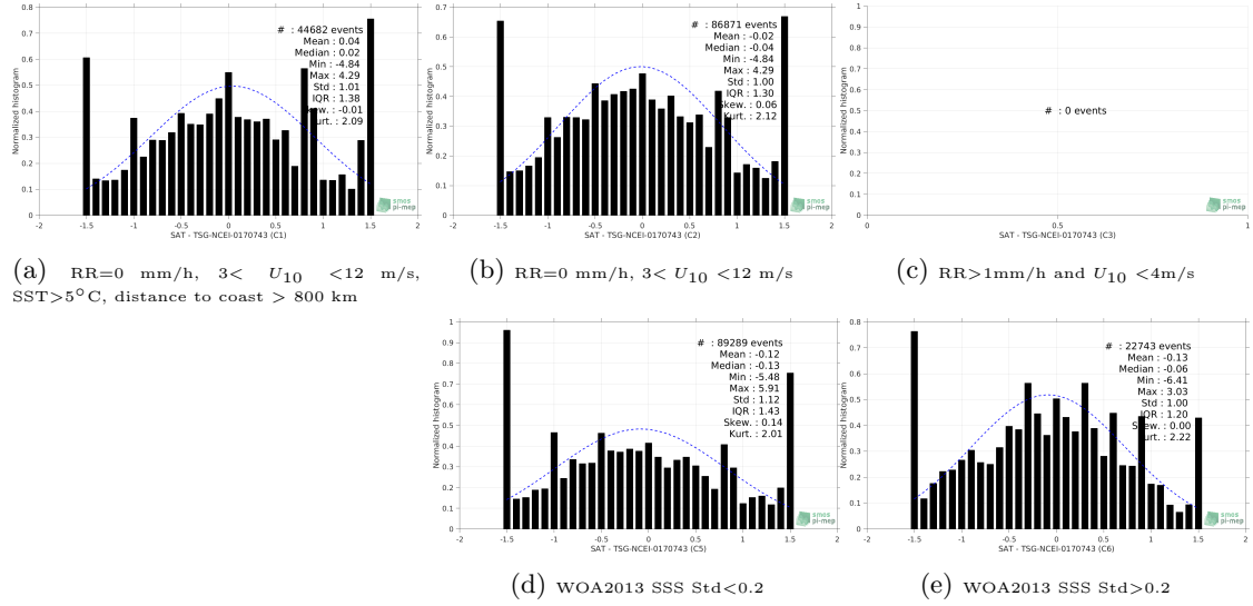
Figure 13: Normalized histogram of \Delta SSS (SMOS-L2-DPGS-v662 - TSG-NCEI-0170743) for 5 different subdatasets corresponding to: RR=0 mm/h, 3 < U_{10} < 12 m/s, SST > 5°C, distance to coast > 800 km (a), RR=0 mm/h, 3 < U_{10} < 12 m/s (b), RR > 1mm/h and U_{10} < 4 m/s (c), WOA2013 SSS Std < 0.2 (d), WOA2013 SSS Std > 0.2 (e).
