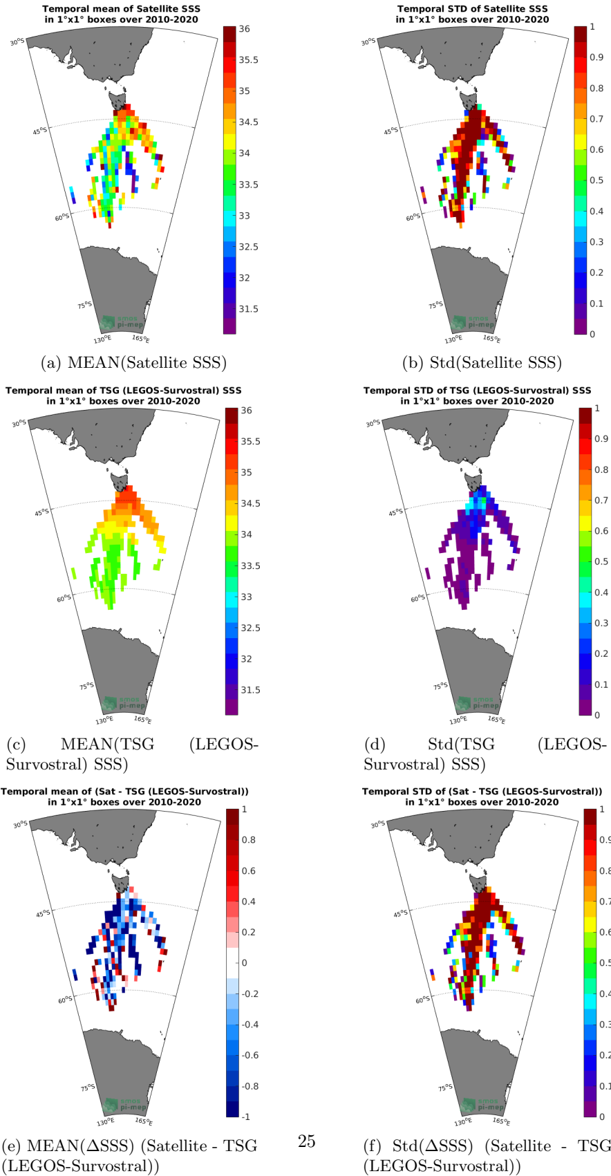
Figure 6: Temporal mean (left) and Std (right) of SSS from SMOS SSS L2 v662 (ESA) (top), TSG (LEGOS-Survostral) (middle), and of \Delta SSS (Satellite - TSG (LEGOS-Survostral)). Only match-up pairs are used to generate these maps.
