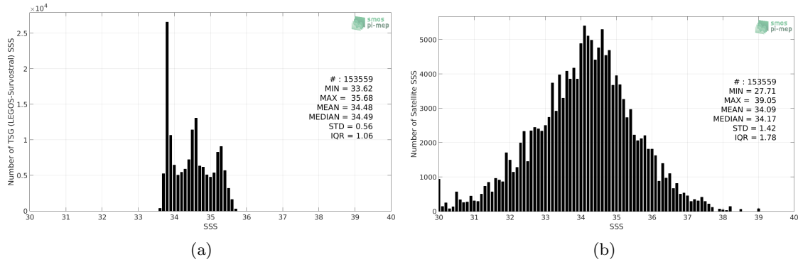
Figure 2: Histograms of SSS from TSG (LEGOS-Survostral) (a) and SMOS SSS L2 v662 (ESA) (b) considering all match-up pairs per bins of 0.1 over the Global Ocean Pi-MEP region and for the full satellite product period.
