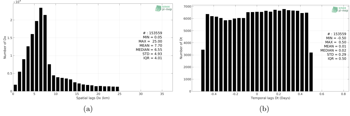
Figure 5: Histograms of the spatial (a) and temporal (b) lags between the location/time of the TSG (LEGOS-Survostral) measurement and the date of the corresponding SMOS SSS L2 v662 (ESA) SSS pixel.
