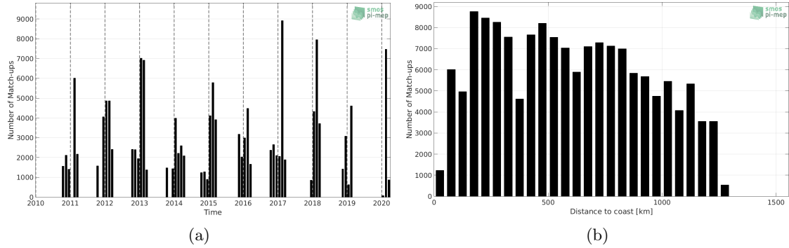
Figure 1: Number of match-ups between TSG (LEGOS-Survostral) and SMOS SSS L2 v662 (ESA) SSS as a function of time (a) and as function of the distance to coast (b) over the Global Ocean Pi-MEP region and for the full satellite product period.
