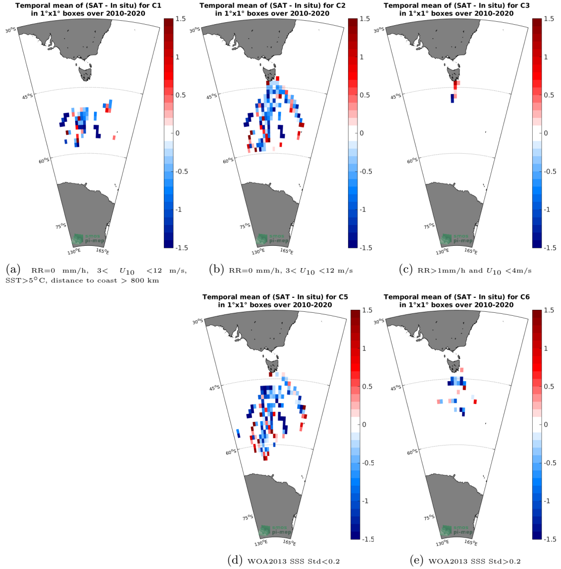
Figure 12: Temporal mean gridded over spatial boxes of size 1°x1° of \Delta\text{SSS} (SMOS SSS L2 v662 (ESA) - TSG (LEGOS-Survostral)) for 5 different subdatasets corresponding to: RR=0 mm/h, 3 < U_{10} < 12 m/s, SST > 5^\circ\text{C} , distance to coast > 800 km (a), RR=0 mm/h, 3 < U_{10} < 12 m/s (b), RR > 1 mm/h and U_{10} < 4 m/s (c), WOA2013 SSS Std < 0.2 (d), WOA2013 SSS Std > 0.2 (e).
