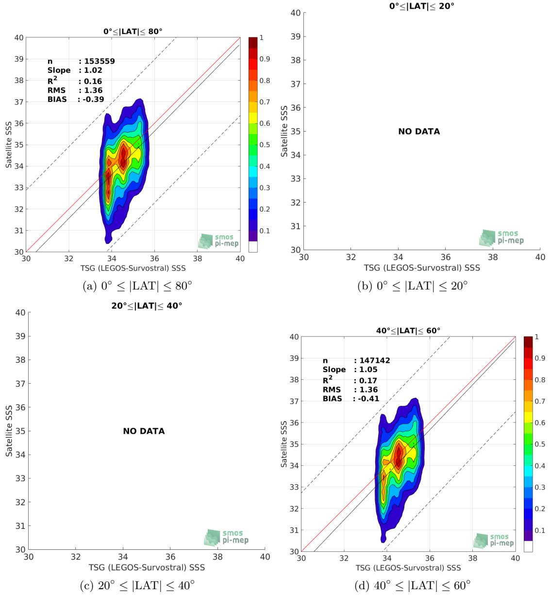
Figure 9: Contour maps of the concentration of SMOS SSS L2 v662 (ESA) SSS (y-axis) versus TSG (LEGOS-Survostral) SSS (x-axis) at match-up pairs for different latitude bands. For each plot, the red line shows x=y . The black thin and dashed lines indicate a linear fit through the data cloud and the \pm 95\% confidence levels, respectively. The number match-up pairs n , the slope and R^2 coefficient of the linear fit, the root mean square (RMS) and the mean bias between satellite and in situ data are indicated for each latitude band in each plots.
