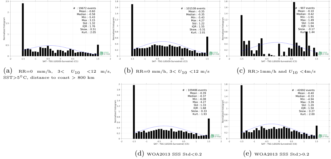
Figure 13: Normalized histogram of \Delta SSS (SMOS SSS L2 v662 (ESA) - TSG (LEGOS-Survostral)) for 5 different subdatasets corresponding to: RR=0 mm/h, 3 < U_{10} < 12 m/s, SST > 5°C, distance to coast > 800 km (a), RR=0 mm/h, 3 < U_{10} < 12 m/s (b), RR > 1 mm/h and U_{10} < 4 m/s (c), WOA2013 SSS Std < 0.2 (d), WOA2013 SSS Std > 0.2 (e).
