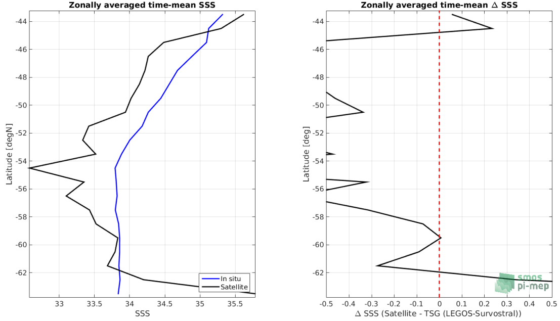
Figure 8: Left panel: Zonal mean SSS from SMOS SSS L2 v662 (ESA) satellite product (black) and from TSG (LEGOS-Survostral) (blue). Right panel: Zonal mean of \Delta SSS (Satellite - TSG (LEGOS-Survostral)) for all the collected Pi-MEP match-up pairs estimated over the full satellite product period.
