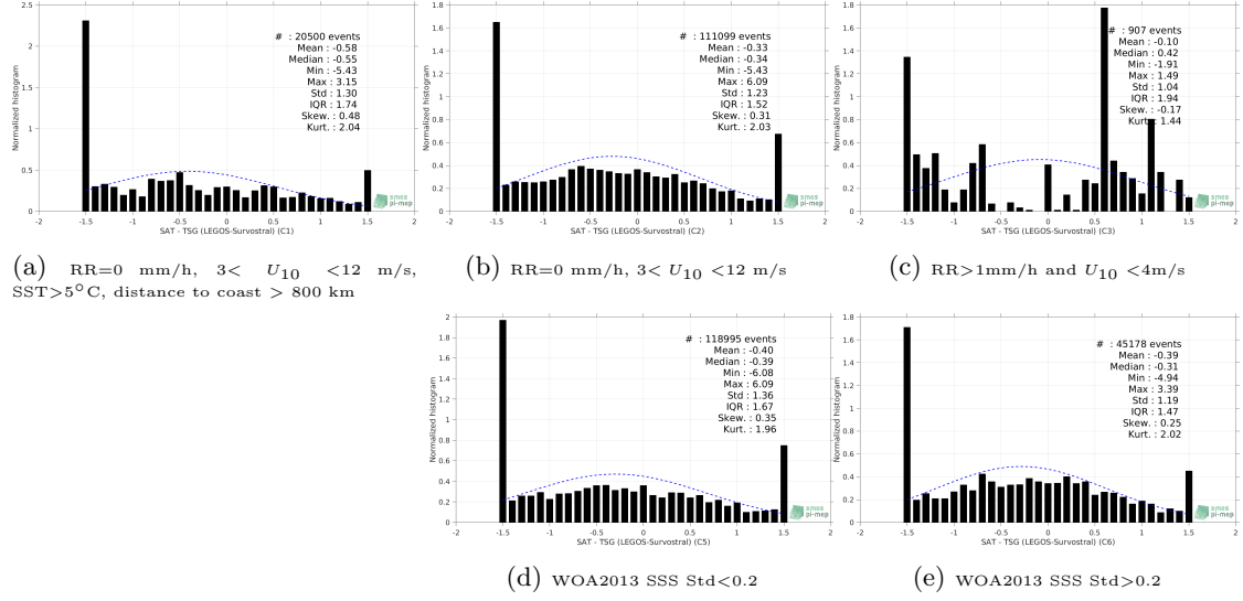
Figure 13: Normalized histogram of \Delta SSS (SMOS SSS L2 v662 (ESA) - TSG (LEGOS-Survostral)) for 5 different subdatasets corresponding to: RR=0 mm/h, 3 < U_{10} < 12 m/s, SST>5°C, distance to coast > 800 km (a), RR=0 mm/h, 3 < U_{10} < 12 m/s (b), RR>1mm/h and U_{10} < 4 m/s (c), WOA2013 SSS Std<0.2 (d), WOA2013 SSS Std>0.2 (e).
