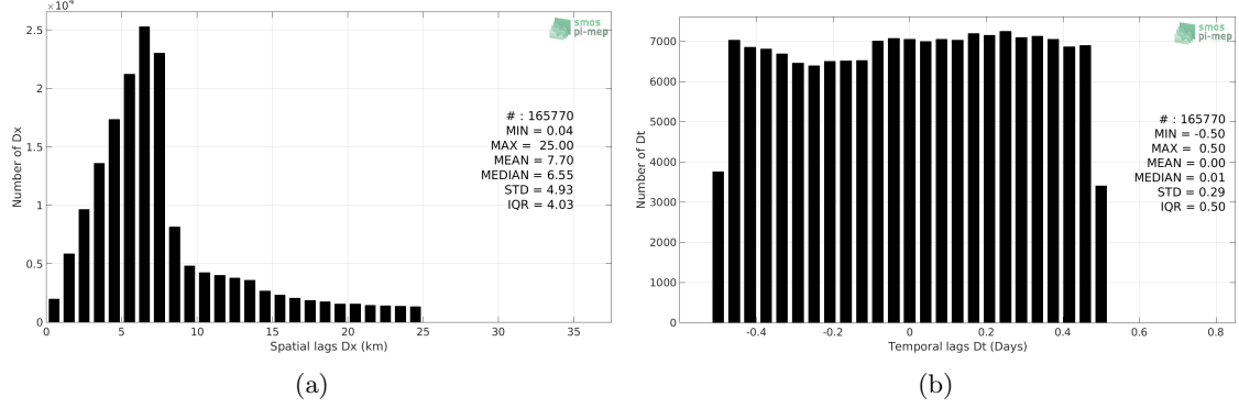
Figure 5: Histograms of the spatial (a) and temporal (b) lags between the time of the TSG (LEGOS-Survostral) measurements and the date of the corresponding SMOS SSS L2 v662 (ESA) SSS product.
