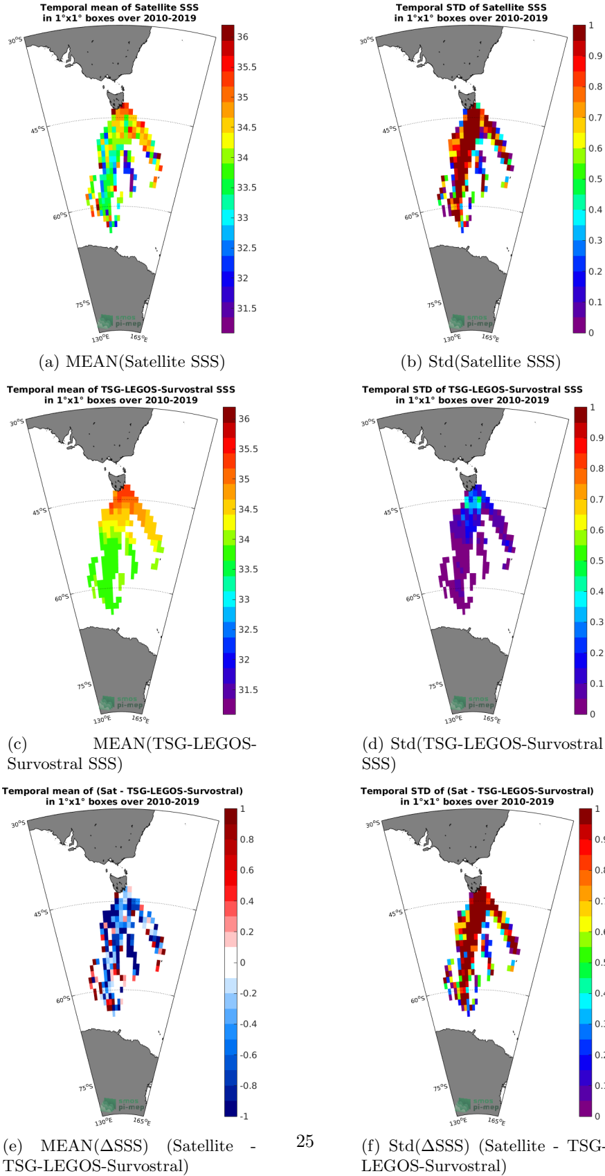
Figure 6: Temporal mean (left) and Std (right) of SSS from SMOS L2 v662 (ESA) (top), TSG-LEGOS-Survostral (middle), and of \Delta SSS (Satellite - TSG-LEGOS-Survostral). Only match-up pairs are used to generate these maps.
