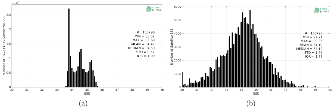
Figure 2: Histograms of SSS from TSG-LEGOS-Survostral (a) and SMOS L2 v662 (ESA) (b) considering all match-up pairs per bins of 0.1 over the Global Ocean Pi-MEP region and for the full satellite product period.
