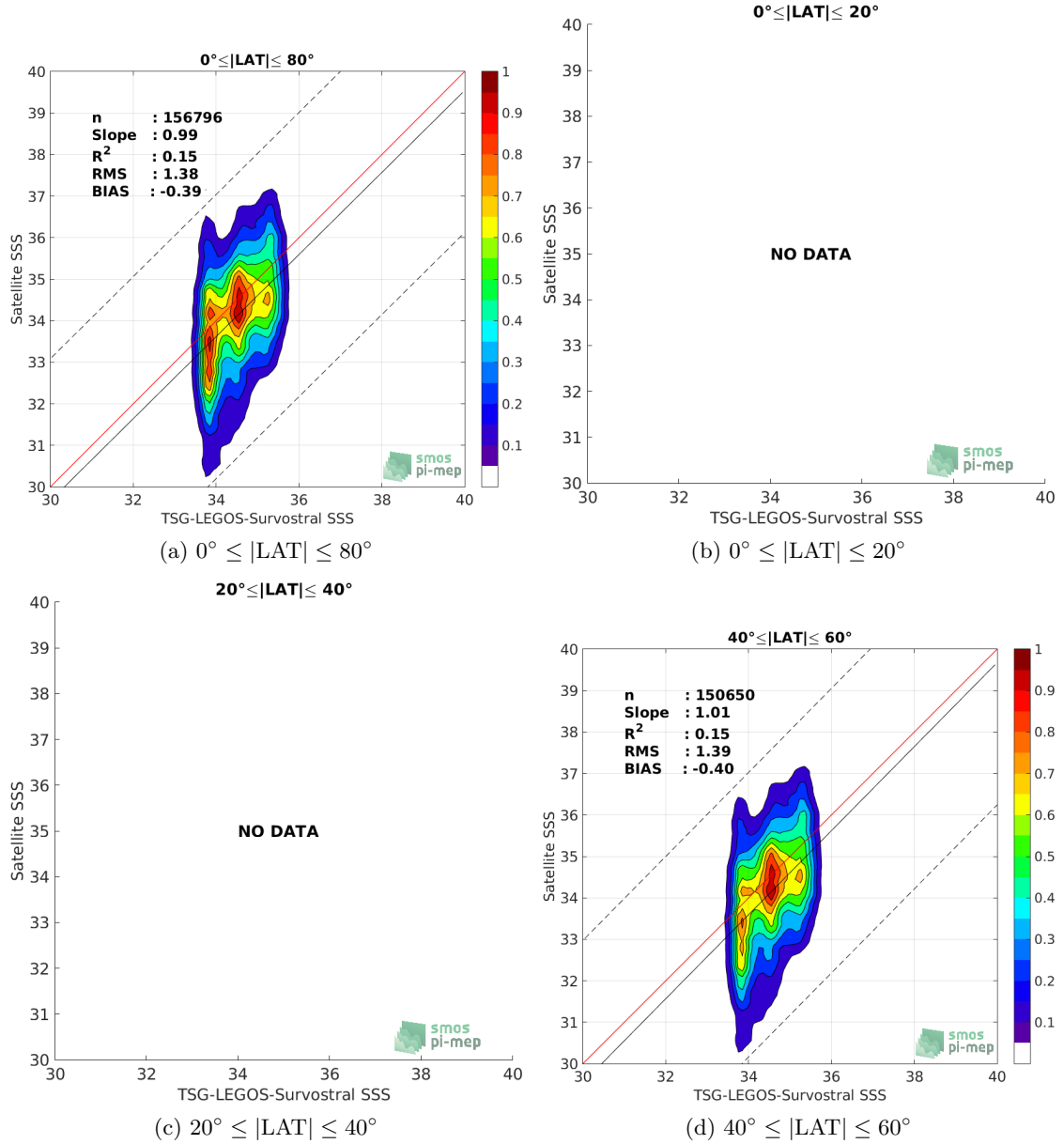
Figure 9: Contour maps of the concentration of SMOS L2 v662 (ESA) SSS (y-axis) versus TSG-LEGOS-Survostral SSS (x-axis) at match-up pairs for different latitude bands. For each plot, the red line shows x=y . The black thin and dashed lines indicate a linear fit through the data cloud and the \pm 95\% confidence levels, respectively. The number match-up pairs n , the slope and R^2 coefficient of the linear fit, the root mean square (RMS) and the mean bias between satellite and in situ data are indicated for each latitude band in each plots.
