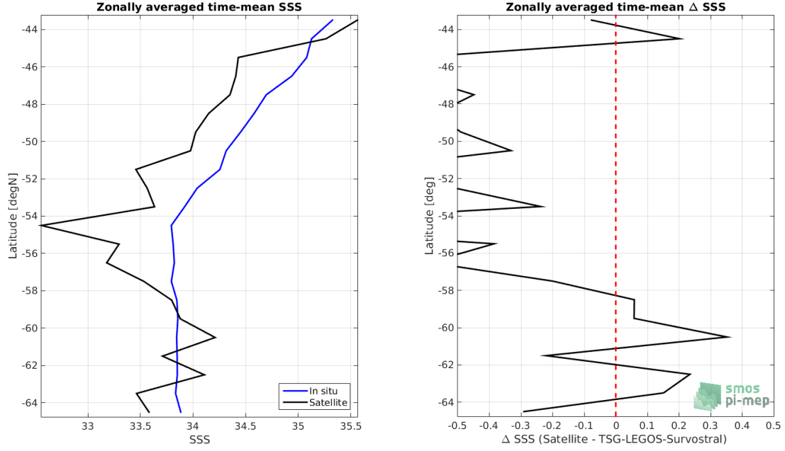
Figure 8: Left panel: Zonal mean SSS from SMOS L2 v662 (ESA) satellite product (black) and from TSG-LEGOS-Survostral (blue). Right panel: Zonal mean of \Delta SSS (Satellite - TSG-LEGOS-Survostral) for all the collected Pi-MEP match-up pairs estimated over the full satellite product period.
