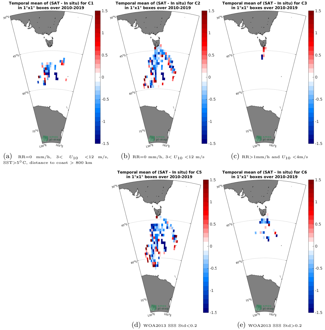
Figure 12: Temporal mean gridded over spatial boxes of size 1°x1° of \Delta\text{SSS} (SMOS L2 v662 (ESA) - TSG-LEGOS-Survostral) for 5 different subdatasets corresponding to: RR=0 mm/h, 3 < U_{10} < 12 m/s, SST > 5^\circ\text{C} , distance to coast > 800 km (a), RR=0 mm/h, 3 < U_{10} < 12 m/s (b), RR > 1 mm/h and U_{10} < 4 m/s (c), WOA2013 SSS Std < 0.2 (d), WOA2013 SSS Std > 0.2 (e).
