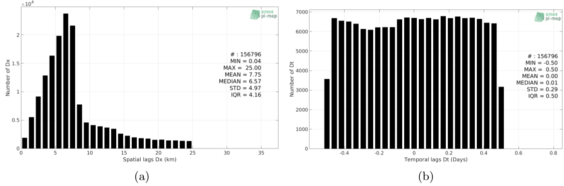
Figure 5: Histograms of the spatial (a) and temporal (b) lags between the time of the TSG-LEGOS-Survostral measurements and the date of the corresponding SMOS L2 v662 (ESA) SSS product.
