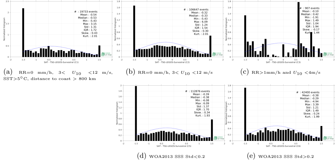
Figure 13: Normalized histogram of \Delta SSS (SMOS L2 v662 (ESA) - TSG-LEGOS-Survostral) for 5 different subdatasets corresponding to: RR=0 mm/h, 3 < U_{10} < 12 m/s, SST > 5°C, distance to coast > 800 km (a), RR=0 mm/h, 3 < U_{10} < 12 m/s (b), RR > 1mm/h and U_{10} < 4 m/s (c), WOA2013 SSS Std < 0.2 (d), WOA2013 SSS Std > 0.2 (e).
