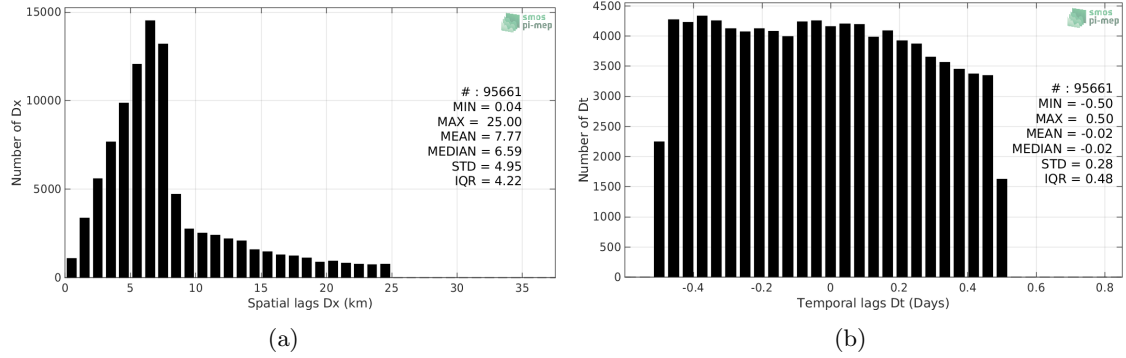
Figure 5: Histograms of the spatial (a) and temporal (b) lags between the time of the TSG-LEGOS-Survostral measurements and the date of the corresponding SMOS-L2-DPGS-v662 SSS product.
