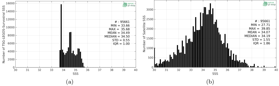
Figure 2: Histograms of SSS from TSG-LEGOS-Survostral (a) and SMOS-L2-DPGS-v662 (b) considering all match-up pairs per bins of 0.1 over the Global Ocean Pi-MEP region and for the full satellite product period.
