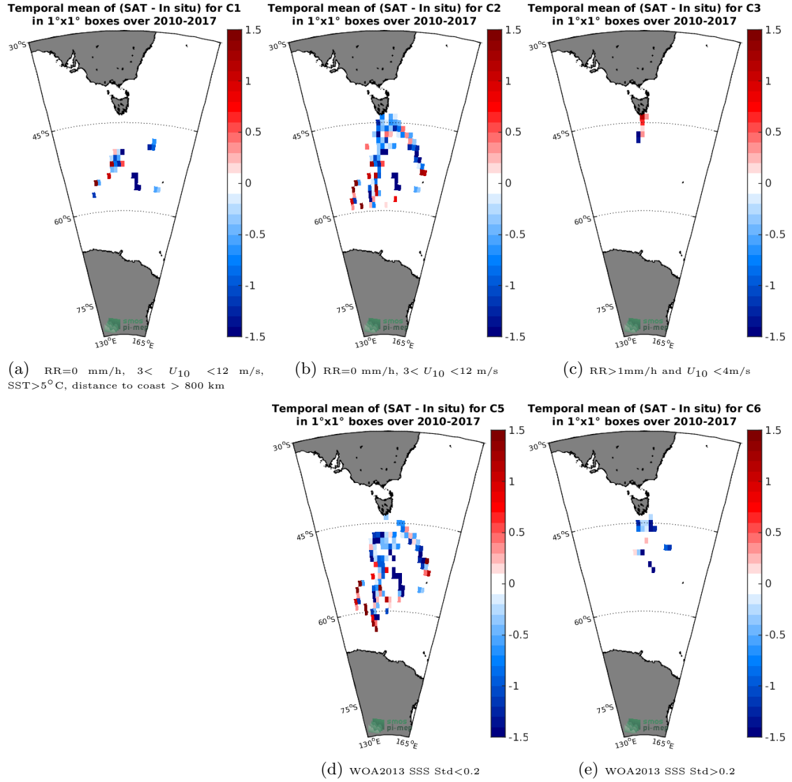
Figure 12: Temporal mean gridded over spatial boxes of size 1°x1° of \Delta SSS (SMOS-L2-DPGS-v662 - TSG-LEGOS-Survostral) for 5 different subdatasets corresponding to:RR=0 mm/h, 3 < U_{10} < 12 m/s, SST>5°C, distance to coast > 800 km (a), RR=0 mm/h, 3 < U_{10} < 12 m/s (b), RR>1mm/h and U_{10} < 4 m/s (c), WOA2013 SSS Std<0.2 (d), WOA2013 SSS Std>0.2 (e).
