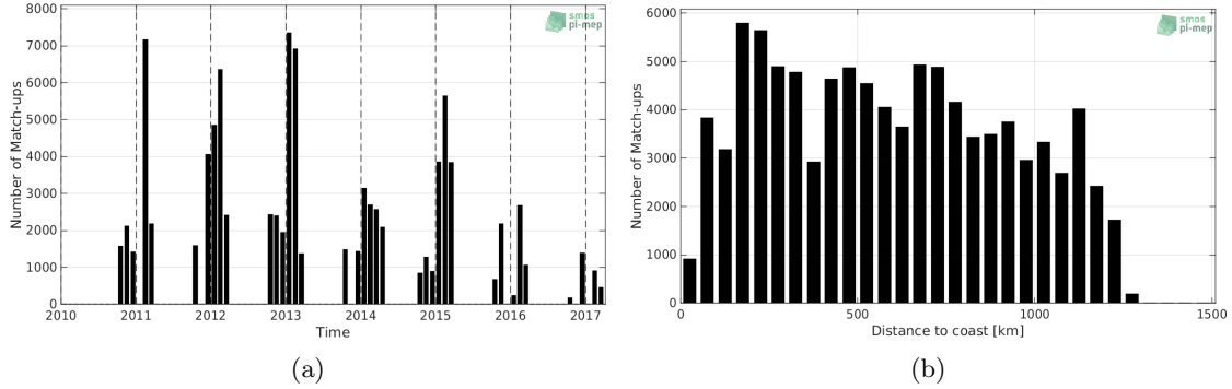
Figure 1: Number of match-ups between TSG-LEGOS-Survostral and SMOS-L2-DPGS-v662 SSS as a function of time (a) and as function of the distance to coast (b) over the Global Ocean Pi-MEP region and for the full satellite product period.
