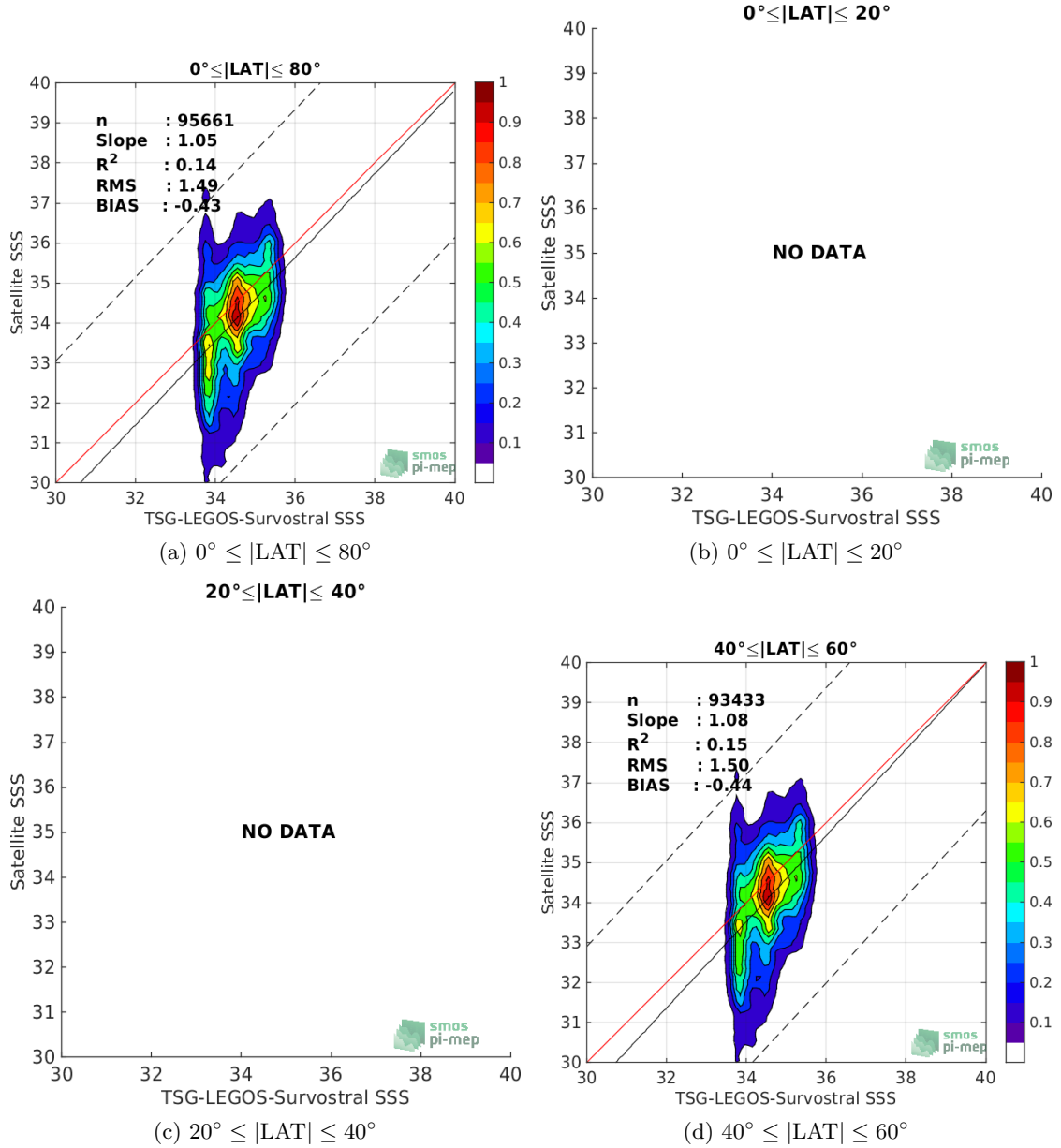
Figure 9: Contour maps of the concentration of SMOS-L2-DPGS-v662 SSS (y-axis) versus TSG-LEGOS-Survostral SSS (x-axis) at match-up pairs for different latitude bands. For each plot, the red line shows x=y . The black thin and dashed lines indicate a linear fit through the data cloud and the \pm 95\% confidence levels, respectively. The number match-up pairs n , the slope and R^2 coefficient of the linear fit, the root mean square (RMS) and the mean bias between satellite and in situ data are indicated for each latitude band in each plots.
