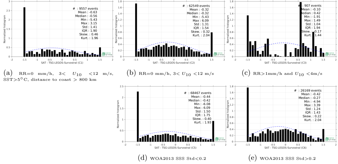
Figure 13: Normalized histogram of \Delta SSS (SMOS-L2-DPGS-v662 - TSG-LEGOS-Survostral) for 5 different subdatasets corresponding to: RR=0 mm/h, 3 < U_{10} < 12 m/s, SST>5°C, distance to coast > 800 km (a), RR=0 mm/h, 3 < U_{10} < 12 m/s (b), RR>1mm/h and U_{10} < 4 m/s (c), WOA2013 SSS Std<0.2 (d), WOA2013 SSS Std>0.2 (e).
