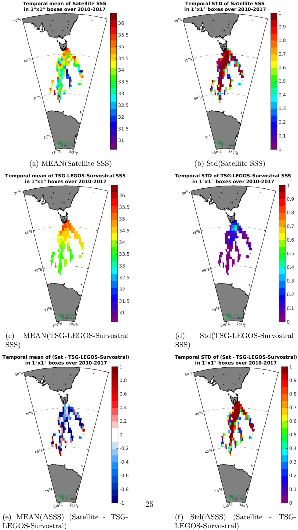
Figure 6: Temporal mean (left) and Std (right) of SSS from SMOS-L2-DPGS-v662 (top), TSG-LEGOS-Survostral (middle), and of \Delta SSS (Satellite - TSG-LEGOS-Survostral). Only match-up pairs are used to generate these maps.
