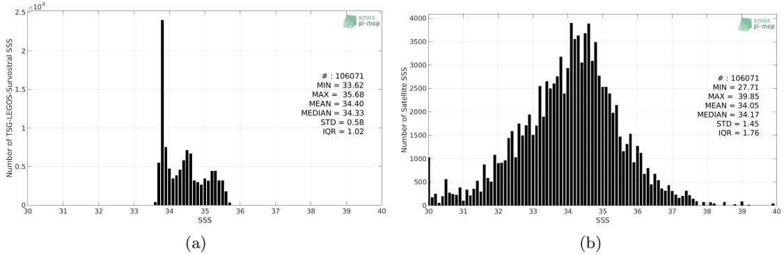
Figure 2: Histograms of SSS from TSG-LEGOS-Survostral (a) and SMOS-L2-DPGS-v662 (b) considering all match-up pairs per bins of 0.1 over the Global Ocean Pi-MEP region and for the full satellite product period.
