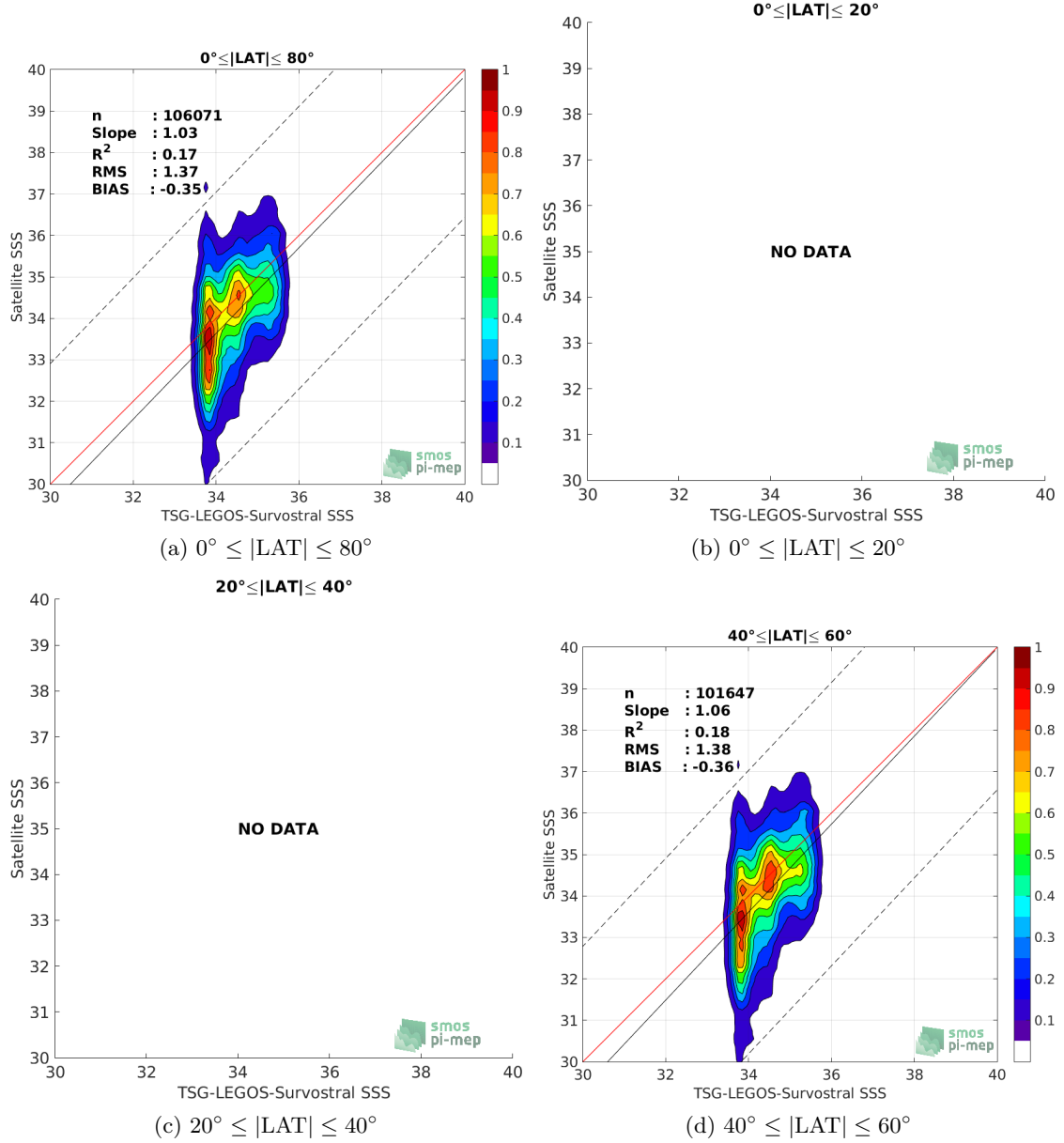
Figure 9: Contour maps of the concentration of SMOS-L2-DPGS-v662 SSS (y-axis) versus TSG-LEGOS-Survostral SSS (x-axis) at match-up pairs for different latitude bands. For each plot, the red line shows x=y . The black thin and dashed lines indicate a linear fit through the data cloud and the \pm 95\% confidence levels, respectively. The number match-up pairs n , the slope and R^2 coefficient of the linear fit, the root mean square (RMS) and the mean bias between satellite and in situ data are indicated for each latitude band in each plots.
