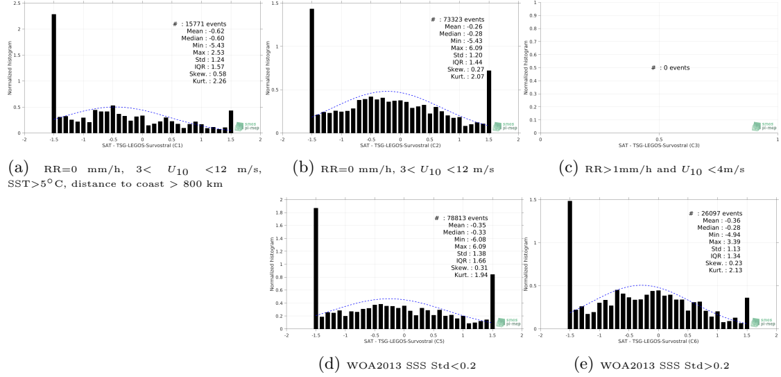
Figure 13: Normalized histogram of \Delta SSS (SMOS-L2-DPGS-v662 - TSG-LEGOS-Survostral) for 5 different subdatasets corresponding to: RR=0 mm/h, 3 < U_{10} < 12 m/s, SST > 5^\circ C , distance to coast > 800 km (a), RR=0 mm/h, 3 < U_{10} < 12 m/s (b), RR > 1 mm/h and U_{10} < 4 m/s (c), WOA2013 SSS Std < 0.2 (d), WOA2013 SSS Std > 0.2 (e).
