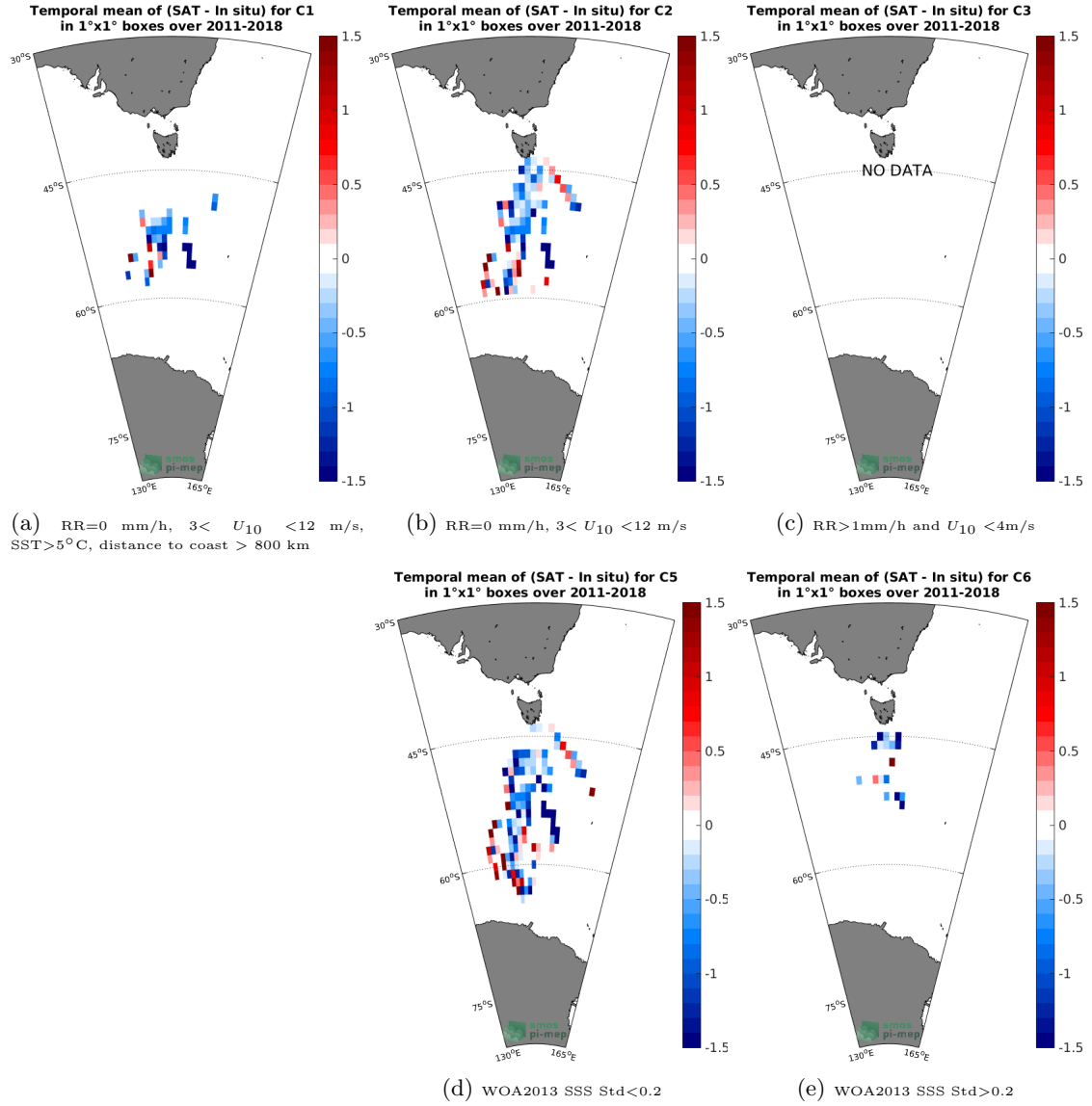
Figure 12: Temporal mean gridded over spatial boxes of size 1°x1° of \Delta\text{SSS} (SMOS-L2-DPGS-v662 - TSG-LEGOS-Survostral) for 5 different subdatasets corresponding to: RR=0 mm/h, 3 < U_{10} < 12 m/s, SST > 5^{\circ}\text{C} , distance to coast > 800 km (a), RR=0 mm/h, 3 < U_{10} < 12 m/s (b), RR > 1\text{mm/h} and U_{10} < 4\text{m/s} (c), WOA2013 SSS Std < 0.2 (d), WOA2013 SSS Std > 0.2 (e).
