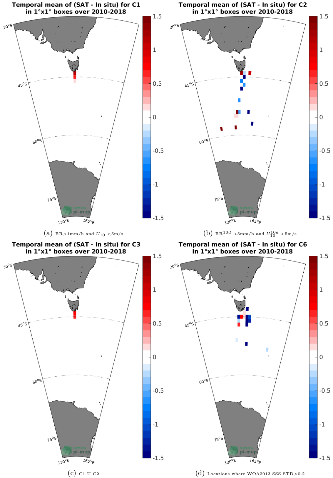
Figure 12: Temporal mean gridded over spatial boxes of size 1°x1° of \Delta\text{SSS} (SMOS-L2-DPGS-v662 - TSG-LEGOS-Survostral) for 4 different subdatasets corresponding to: RR > 1\text{mm/h} and U_{10} < 5\text{m/s} (a), RR^{10d} > 5\text{mm/h} and U_{10}^{10d} < 5\text{m/s} (b), C1 U C2 (c), Locations where WOA2013 SSS STD > 0.2 (d).
