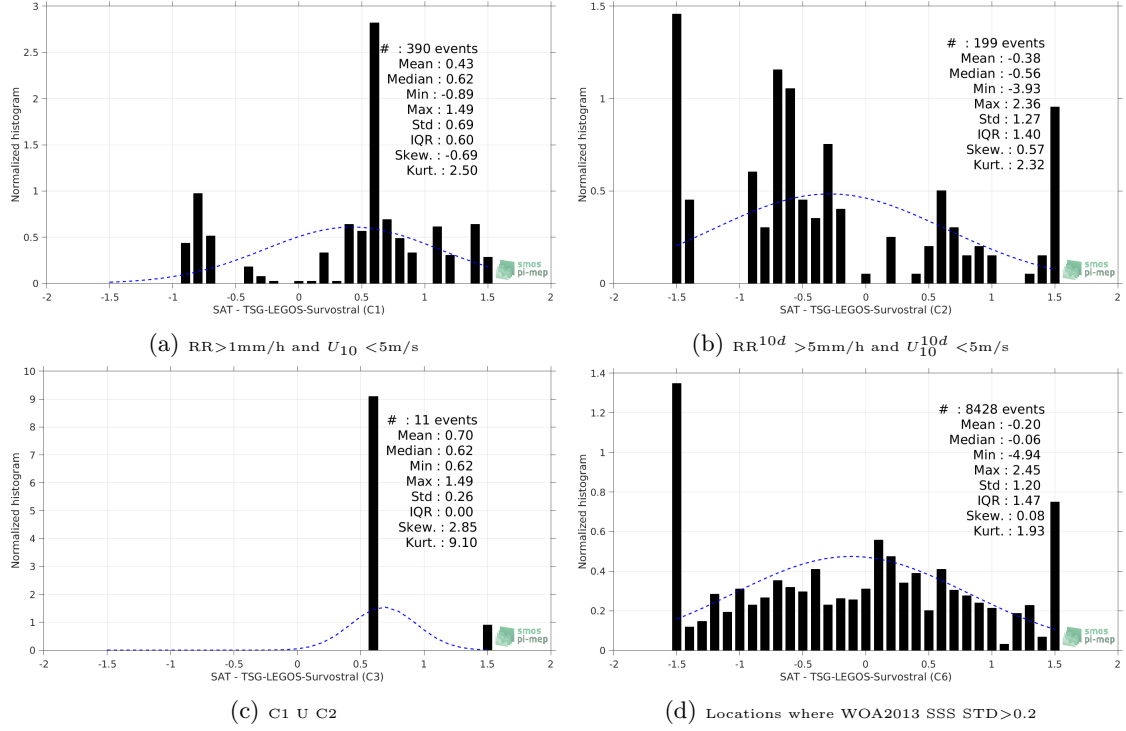
Figure 13: Normalized histogram of \Delta SSS (SMOS-L2-DPGS-v662 - TSG-LEGOS-Survostral) for 6 different subdatasets corresponding to: RR > 1\text{mm/h} and U_{10} < 5\text{m/s} (a), RR^{10d} > 5\text{mm/h} and U_{10}^{10d} < 5\text{m/s} (b), C1 U C2 (c), Locations where WOA2013 SSS STD > 0.2 (d).
