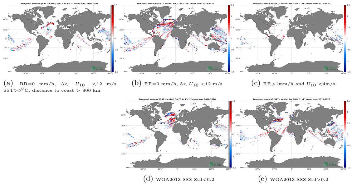
Figure 12: Temporal mean gridded over spatial boxes of size 1^\circ \times 1^\circ of \Delta SSS (SMOS SSS L2 v662 (ESA) - TSG (LEGOS-DM)) for 5 different subdatasets corresponding to:RR=0 mm/h, 3 < U_{10} < 12 m/s, SST >5^\circ C, distance to coast > 800 km (a), RR=0 mm/h, 3 < U_{10} < 12 m/s (b), RR >1 mm/h and U_{10} < 4 m/s (c), WOA2013 SSS Std <0.2 (d), WOA2013 SSS Std >0.2 (e).
