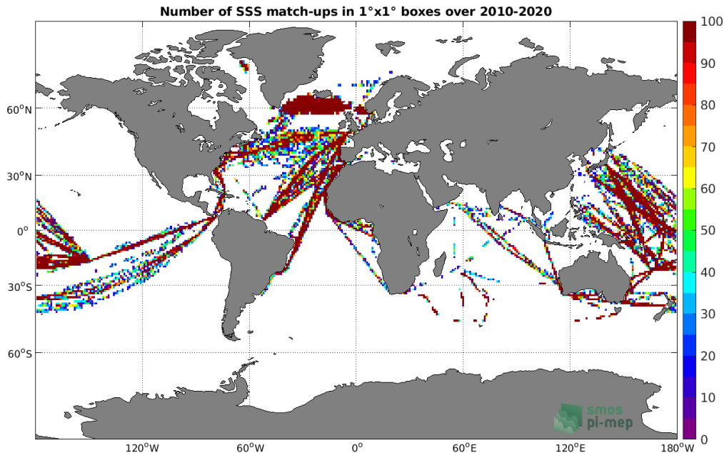
Figure 4: Number of SSS match-ups between TSG (LEGOS-DM) SSS and the SMOS SSS L2 v662 (ESA) SSS product for the Global Ocean Pi-MEP region over 1^\circ \times 1^\circ boxes and for the full satellite product period.
