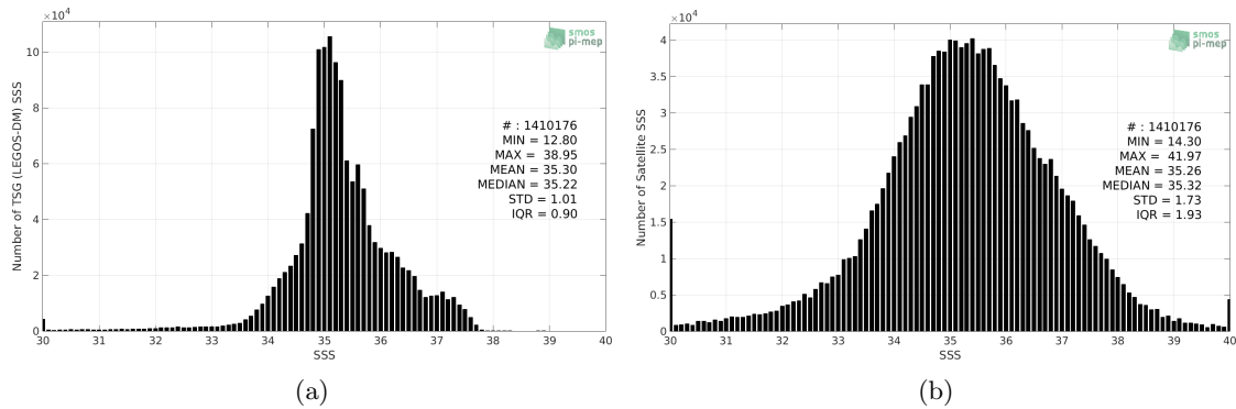
Figure 2: Histograms of SSS from TSG (LEGOS-DM) (a) and SMOS SSS L2 v662 (ESA) (b) considering all match-up pairs per bins of 0.1 over the Global Ocean Pi-MEP region and for the full satellite product period.
