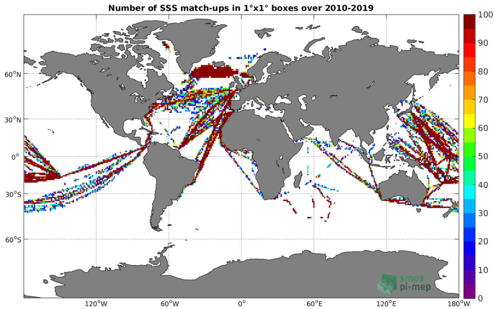
Figure 4: Number of SSS match-ups between TSG (LEGOS-DM) SSS and the SMOS SSS L2 v662 (ESA) SSS product for the Global Ocean Pi-MEP region over 1°x1° boxes and for the full satellite product period.
