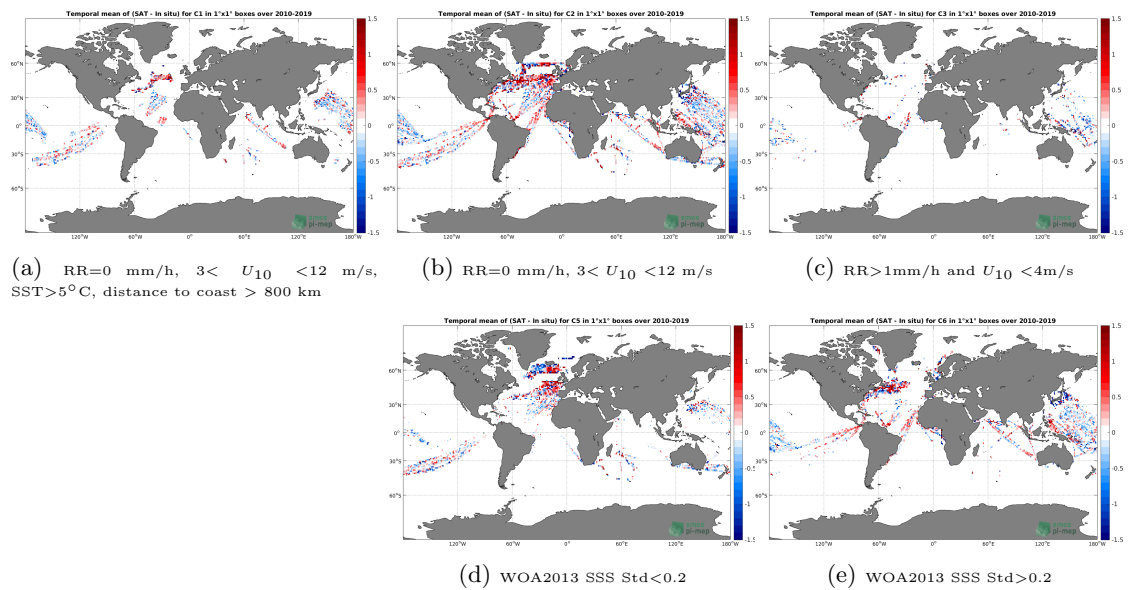
Figure 12: Temporal mean gridded over spatial boxes of size 1°x1° of \Delta SSS (SMOS SSS L2 v662 (ESA) - TSG (LEGOS-DM)) for 5 different subdatasets corresponding to:RR=0 mm/h, 3 < U_{10} < 12 m/s, SST>5°C, distance to coast > 800 km (a), RR=0 mm/h, 3 < U_{10} < 12 m/s (b), RR>1mm/h and U_{10} < 4 m/s (c), WOA2013 SSS Std<0.2 (d), WOA2013 SSS Std>0.2 (e).
