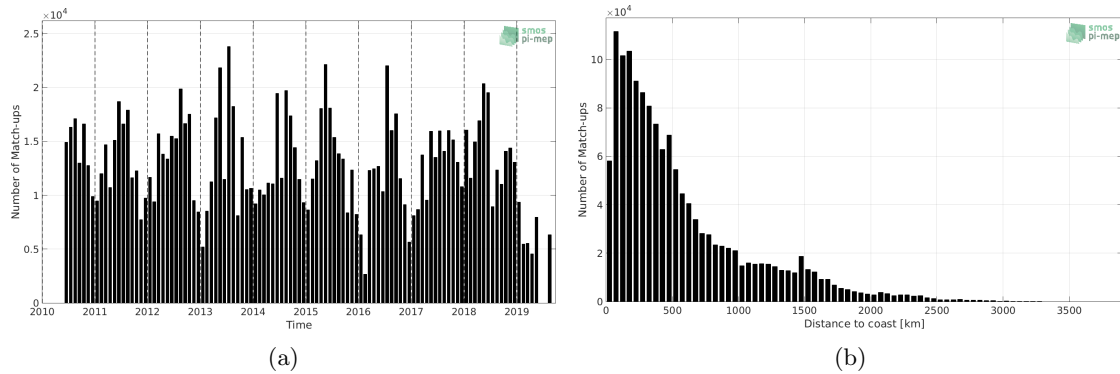
Figure 1: Number of match-ups between TSG (LEGOS-DM) and SMOS SSS L2 v662 (ESA) SSS as a function of time (a) and as function of the distance to coast (b) over the Global Ocean Pi-MEP region and for the full satellite product period.
