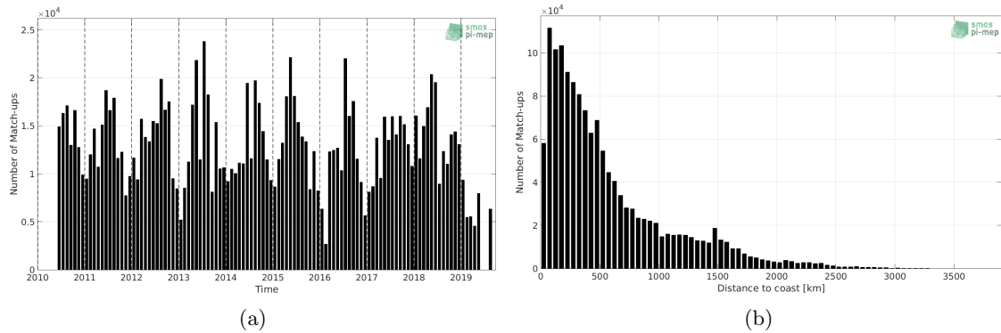
Figure 1: Number of match-ups between TSG-LEGOS-DM and SMOS L2 v662 (ESA) SSS as a function of time (a) and as function of the distance to coast (b) over the Global Ocean Pi-MEP region and for the full satellite product period.
