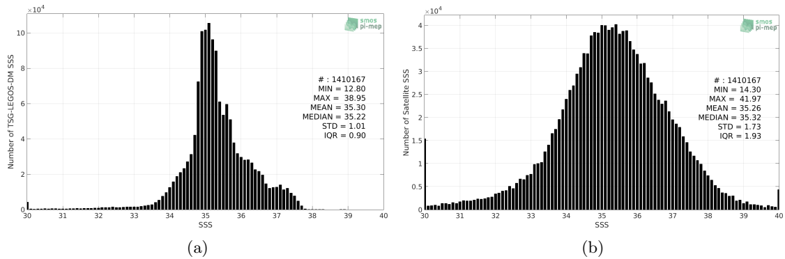
Figure 2: Histograms of SSS from TSG-LEGOS-DM (a) and SMOS L2 v662 (ESA) (b) considering all match-up pairs per bins of 0.1 over the Global Ocean Pi-MEP region and for the full satellite product period.
