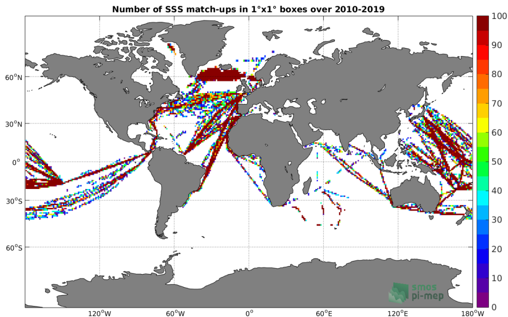
Figure 4: Number of SSS match-ups between TSG-LEGOS-DM SSS and the SMOS L2 v662 (ESA) SSS product for the Global Ocean Pi-MEP region over 1^\circ \times 1^\circ boxes and for the full satellite product period.
