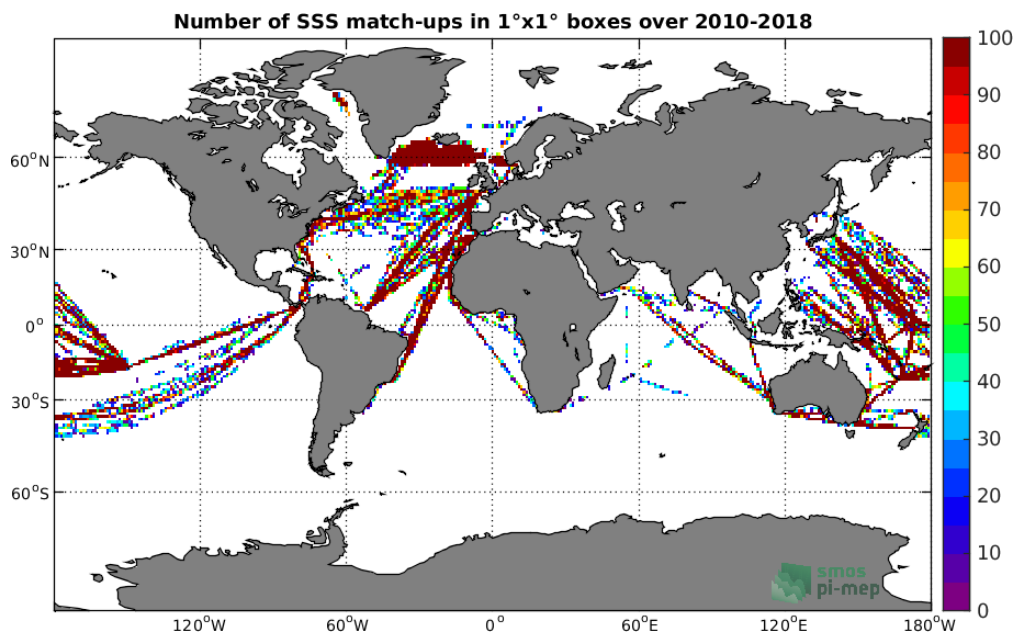
Figure 4: Number of SSS match-ups between TSG-LEGOS-DM SSS and the SMOS-L2-DPGS-v662 SSS product for the Global Ocean Pi-MEP region over 1°x1° boxes and for the full satellite product period.
