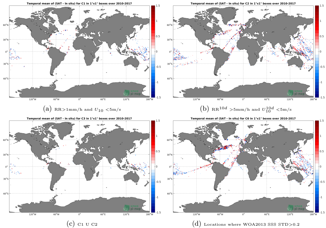
Figure 12: Temporal mean gridded over spatial boxes of size 1^\circ \times 1^\circ of \Delta SSS (SMOS-L2-DPGS-v662 - TSG-LEGOS-DM) for 4 different subdatasets corresponding to: RR > 1\text{mm/h} and U_{10} < 5\text{m/s} (a), RR^{10d} > 5\text{mm/h} and U_{10}^{10d} < 5\text{m/s} (b), C1 U C2 (c), Locations where WOA2013 SSS STD > 0.2 (d).
