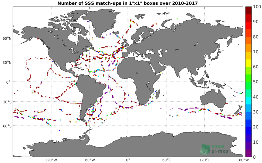
Figure 4: Number of SSS match-ups between TSG (GOSUD-Sailing-ship) SSS and the SMOS SSS L2 v662 (ESA) SSS product for the Global Ocean Pi-MEP region over 1^\circ \times 1^\circ boxes and for the full satellite product period.
