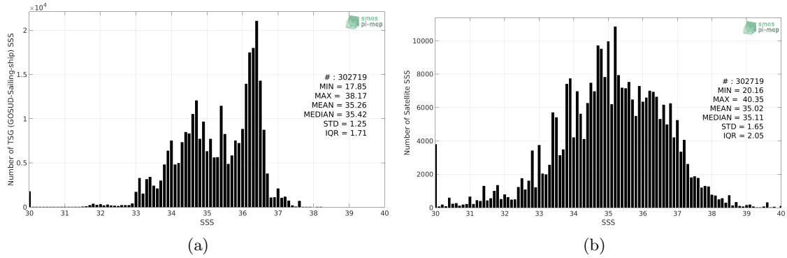
Figure 2: Histograms of SSS from TSG (GOSUD-Sailing-ship) (a) and SMOS SSS L2 v662 (ESA) (b) considering all match-up pairs per bins of 0.1 over the Global Ocean Pi-MEP region and for the full satellite product period.
