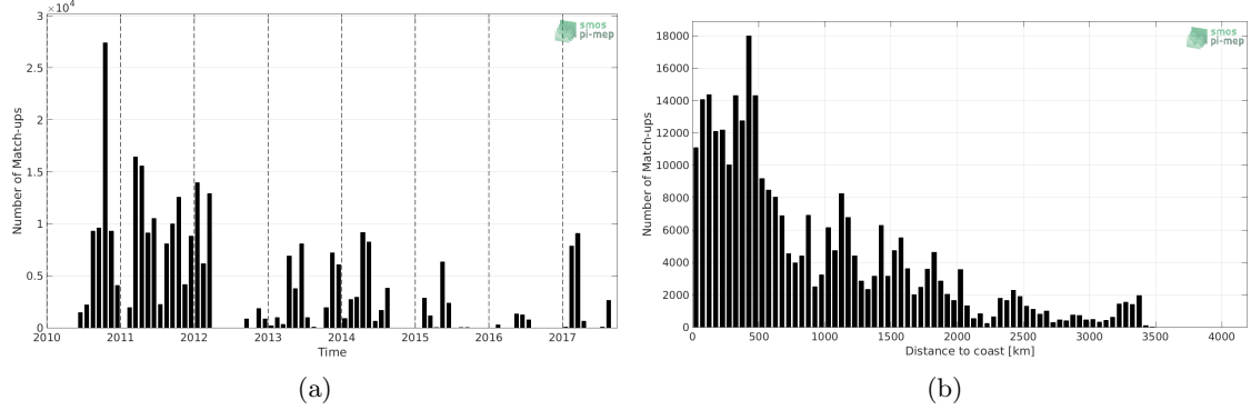
Figure 1: Number of match-ups between TSG (GOSUD-Sailing-ship) and SMOS SSS L2 v662 (ESA) SSS as a function of time (a) and as function of the distance to coast (b) over the Global Ocean Pi-MEP region and for the full satellite product period.
