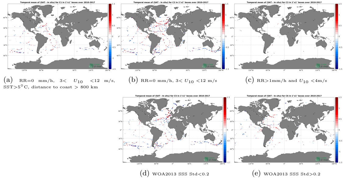
Figure 12: Temporal mean gridded over spatial boxes of size 1^\circ \times 1^\circ of \Delta SSS (SMOS SSS L2 v662 (ESA) - TSG (GOSUD-Sailing-ship)) for 5 different subdatasets corresponding to: RR=0 mm/h, 3 < U_{10} < 12 m/s, SST > 5^\circ C , distance to coast > 800 km (a), RR=0 mm/h, 3 < U_{10} < 12 m/s (b), RR > 1 mm/h and U_{10} < 4 m/s (c), WOA2013 SSS Std < 0.2 (d), WOA2013 SSS Std > 0.2 (e).
