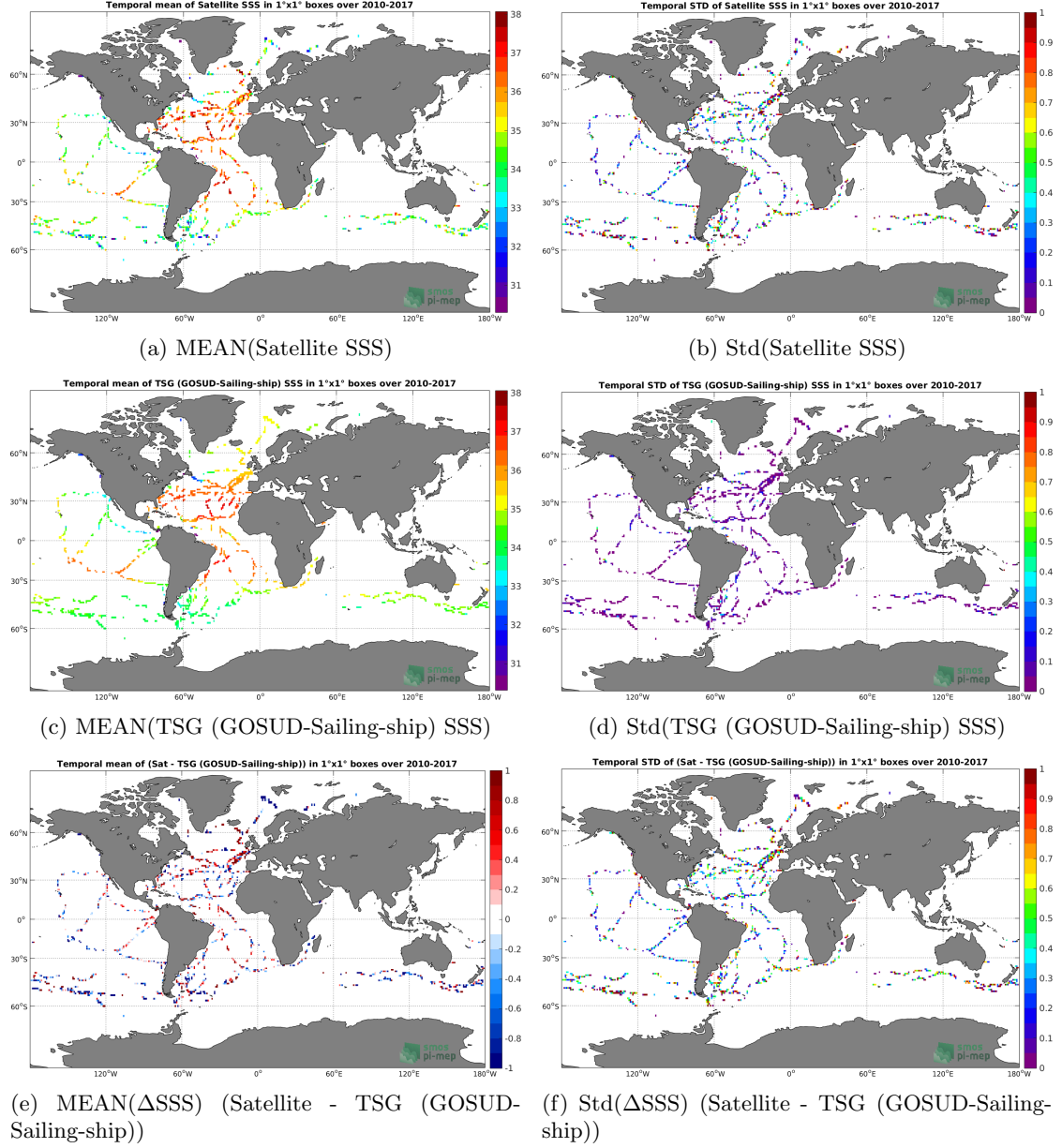
Figure 6: Temporal mean (left) and Std (right) of SSS from SMOS SSS L2 v662 (ESA) (top), TSG (GOSUD-Sailing-ship) (middle), and of \Delta SSS (Satellite - TSG (GOSUD-Sailing-ship)). Only match-up pairs are used to generate these maps.
