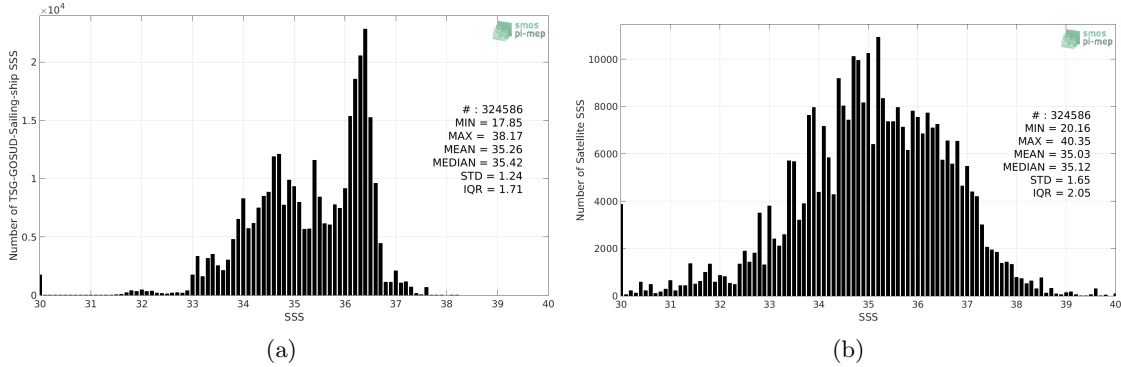
Figure 2: Histograms of SSS from TSG-GOSUD-Sailing-ship (a) and SMOS L2 v662 (ESA) (b) considering all match-up pairs per bins of 0.1 over the Global Ocean Pi-MEP region and for the full satellite product period.
