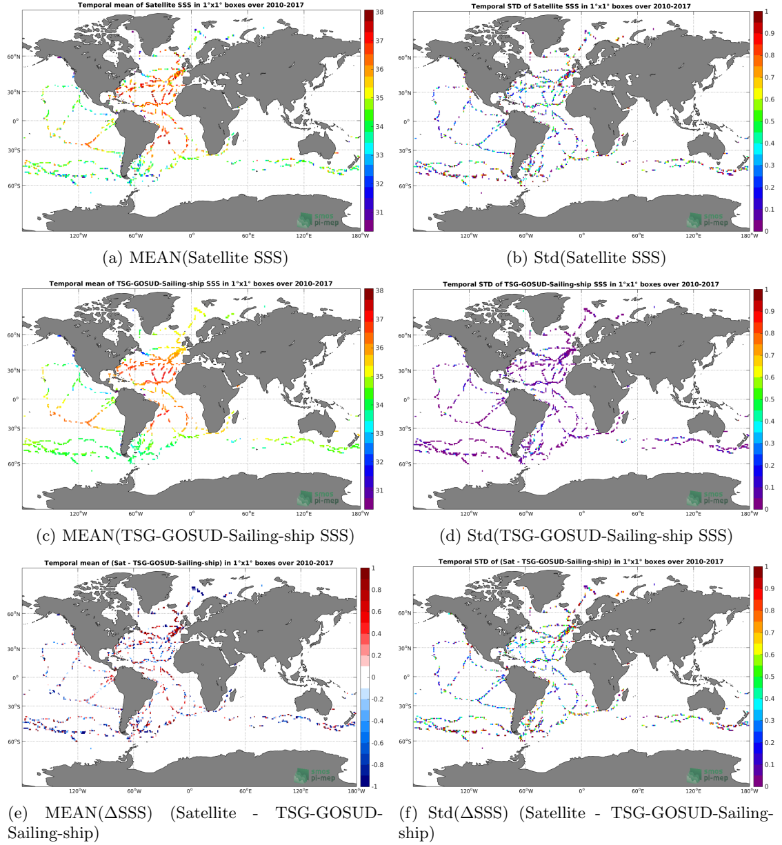
Figure 6: Temporal mean (left) and Std (right) of SSS from SMOS L2 v662 (ESA) (top), TSG-GOSUD-Sailing-ship (middle), and of \Delta SSS (Satellite - TSG-GOSUD-Sailing-ship). Only match-up pairs are used to generate these maps.
