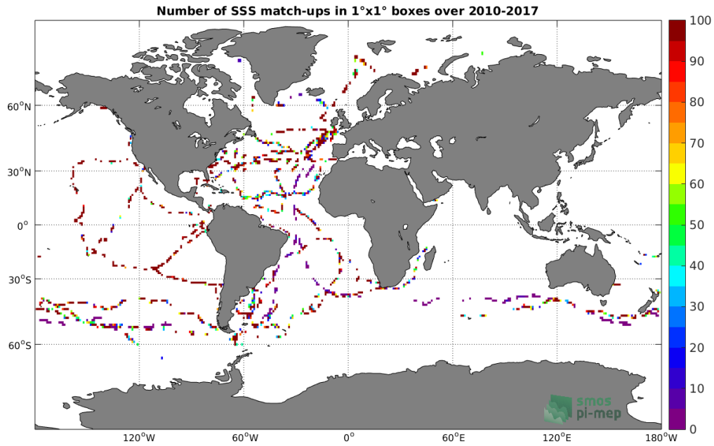
Figure 4: Number of SSS match-ups between TSG-GOSUD-Sailing-ship SSS and the SMOS L2 v662 (ESA) SSS product for the Global Ocean Pi-MEP region over 1^\circ \times 1^\circ boxes and for the full satellite product period.
