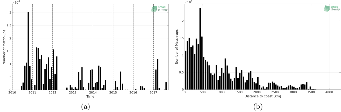
Figure 1: Number of match-ups between TSG-GOSUD-Sailing-ship and SMOS L2 v662 (ESA) SSS as a function of time (a) and as function of the distance to coast (b) over the Global Ocean Pi-MEP region and for the full satellite product period.
