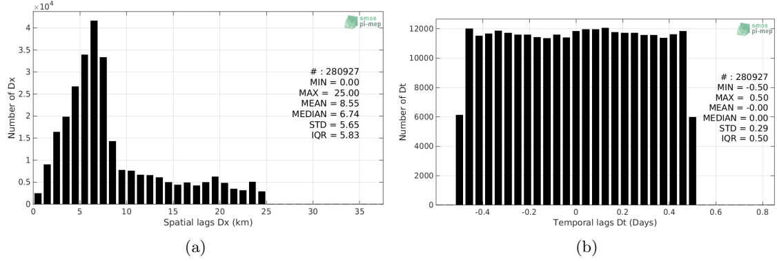
Figure 5: Histograms of the spatial (a) and temporal (b) lags between the time of the TSG-GOSUD-Sailing-ship measurements and the date of the corresponding SMOS-L2-DPGS-v662 SSS product.
