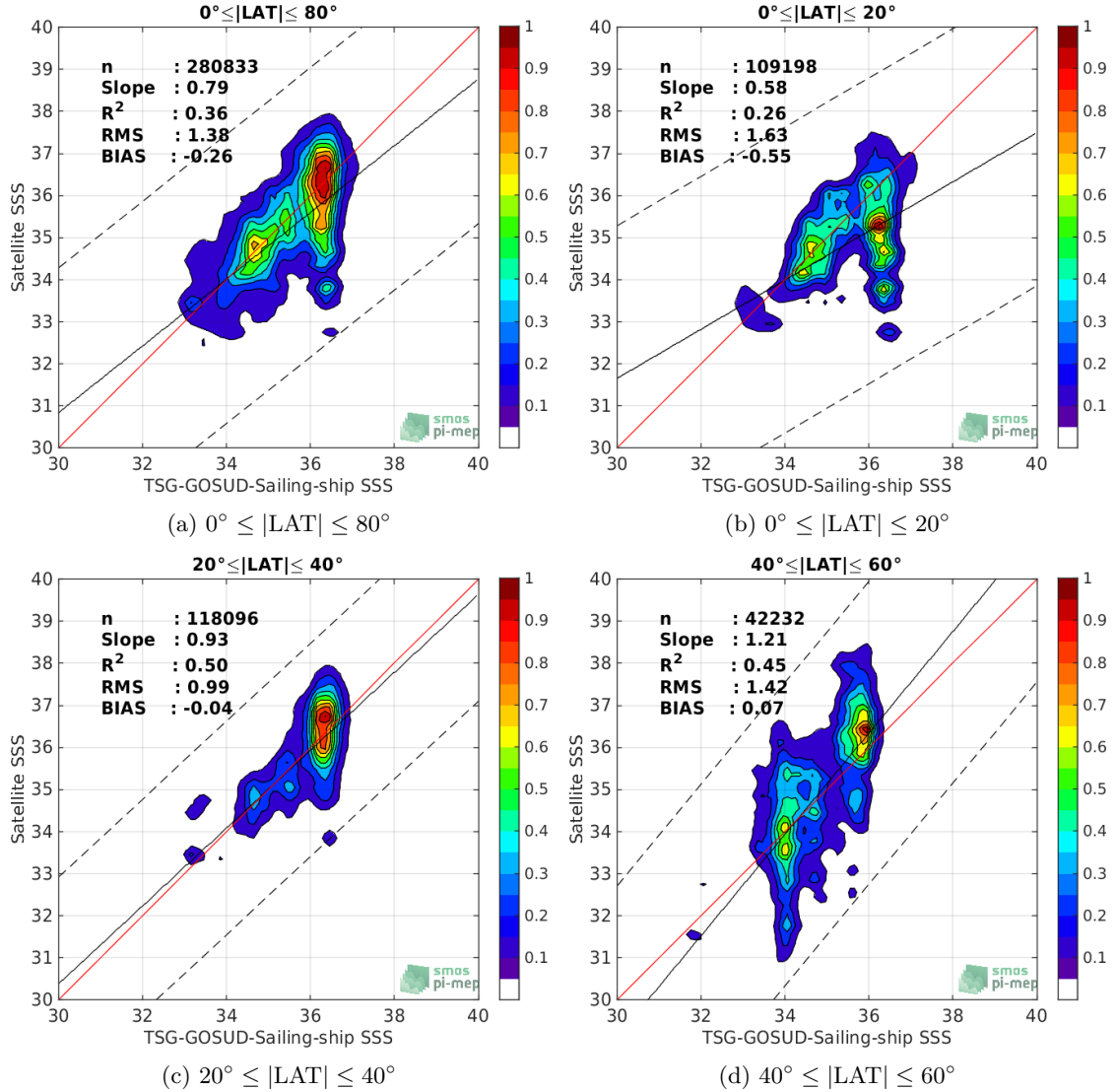
Figure 9: Contour maps of the concentration of SMOS-L2-DPGS-v662 SSS (y-axis) versus TSG-GOSUD-Sailing-ship SSS (x-axis) at match-up pairs for different latitude bands. For each plot, the red line shows x=y . The black thin and dashed lines indicate a linear fit through the data cloud and the \pm 95\% confidence levels, respectively. The number match-up pairs n , the slope and R^2 coefficient of the linear fit, the root mean square (RMS) and the mean bias between satellite and in situ data are indicated for each latitude band in each plots.
