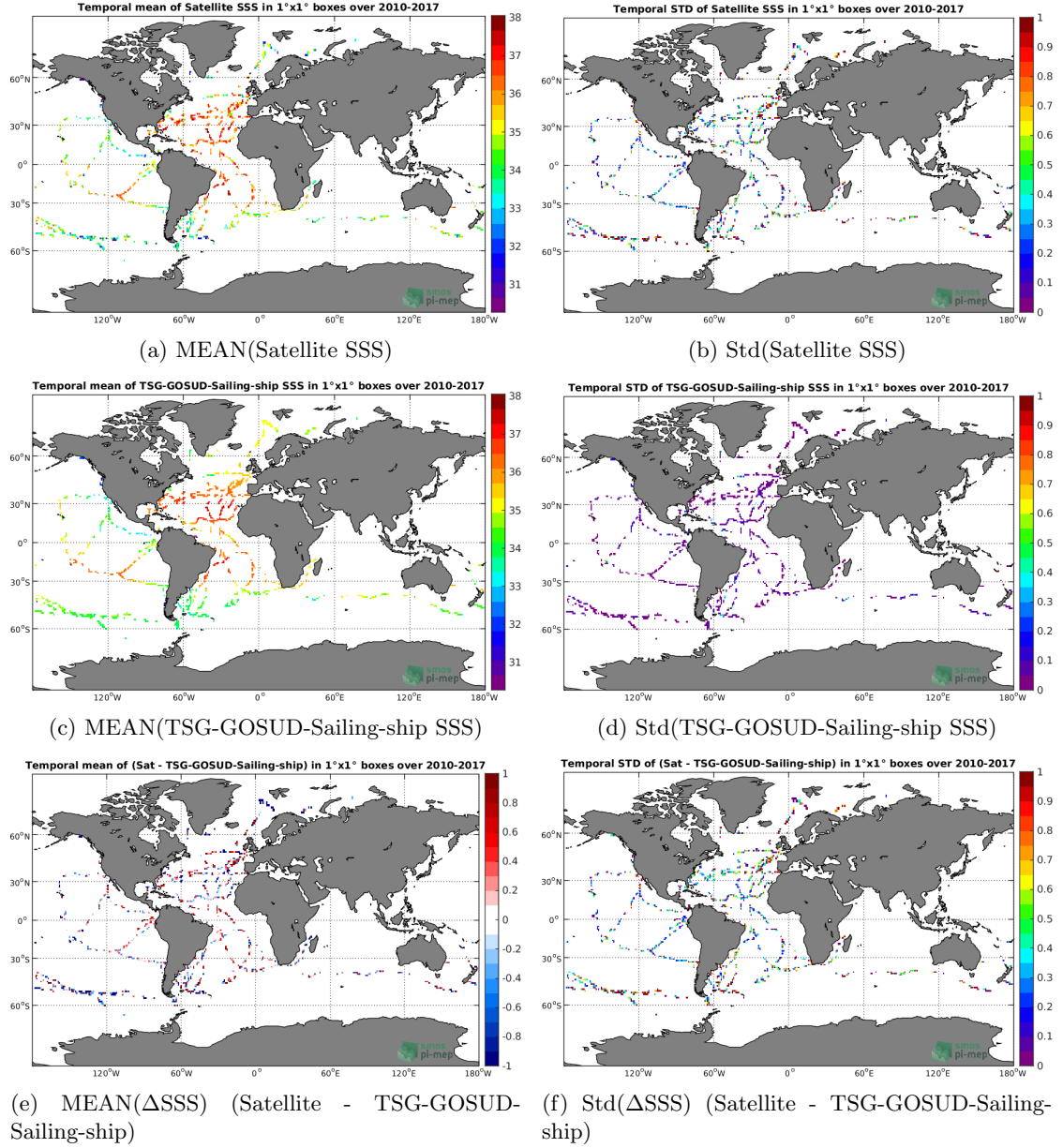
Figure 6: Temporal mean (left) and Std (right) of SSS from SMOS-L2-DPGS-v662 (top), TSG-GOSUD-Sailing-ship (middle), and of \Delta SSS (Satellite - TSG-GOSUD-Sailing-ship). Only match-up pairs are used to generate these maps.
