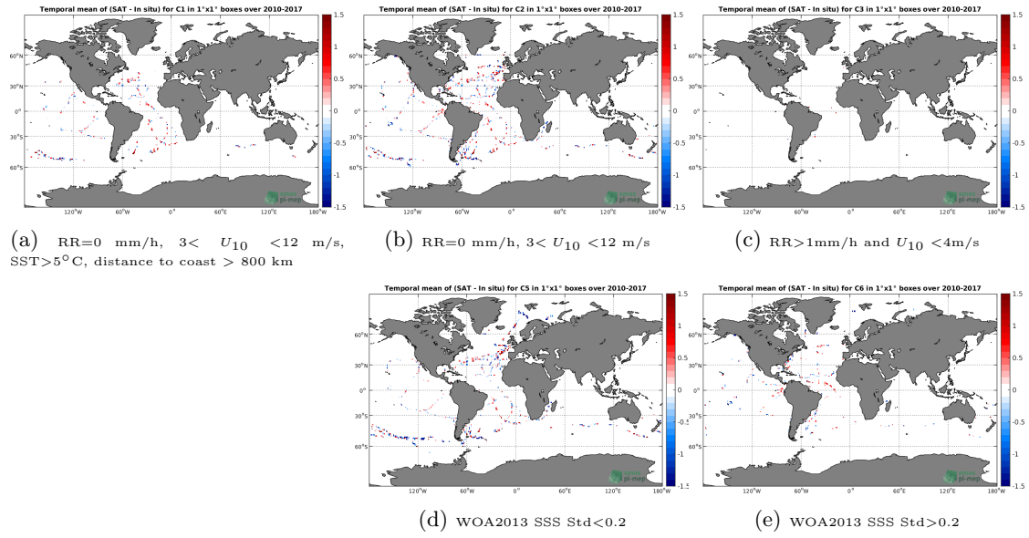
Figure 12: Temporal mean gridded over spatial boxes of size 1^\circ \times 1^\circ of \Delta SSS (SMOS-L2-DPGS-v662 - TSG-GOSUD-Sailing-ship) for 5 different subdatasets corresponding to: RR=0 mm/h, 3 < U_{10} < 12 m/s, SST >5^\circ C, distance to coast > 800 km (a), RR=0 mm/h, 3 < U_{10} < 12 m/s (b), RR >1 mm/h and U_{10} < 4 m/s (c), WOA2013 SSS Std <0.2 (d), WOA2013 SSS Std >0.2 (e).
