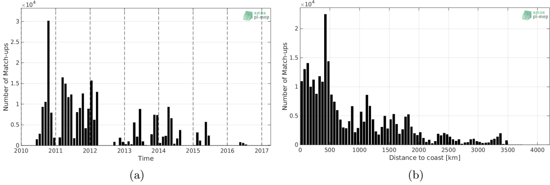
Figure 1: Number of match-ups between TSG-GOSUD-Sailing-ship and SMOS-L2-DPGS-v662 SSS as a function of time (a) and as function of the distance to coast (b) over the Global Ocean Pi-MEP region and for the full satellite product period.
