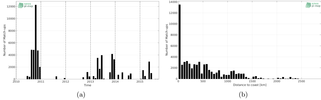
Figure 1: Number of match-ups between TSG-GOSUD-Sailing-ship and SMOS-L2-DPGS-v662 SSS as a function of time (a) and as function of the distance to coast (b) over the Global Ocean Pi-MEP region and for the full satellite product period.
