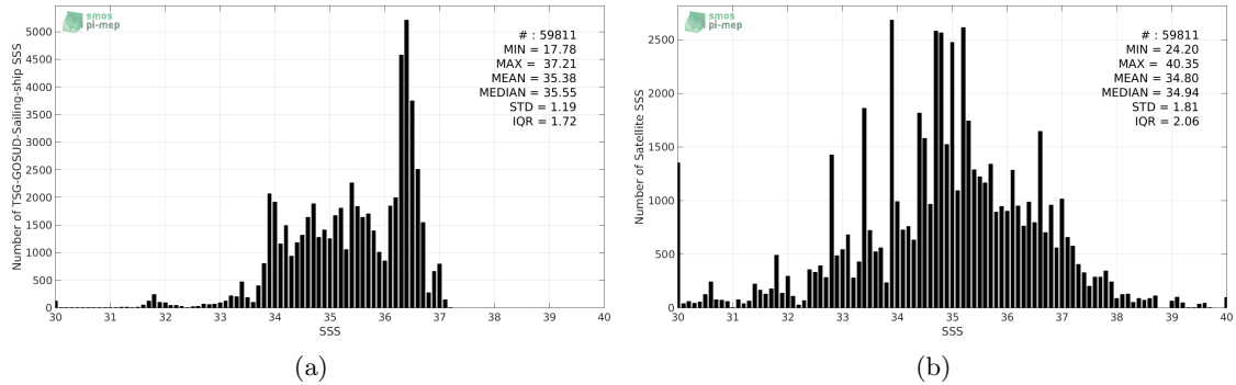
Figure 2: Histograms of SSS from TSG-GOSUD-Sailing-ship (a) and SMOS-L2-DPGS-v662 (b) considering all match-up pairs per bins of 0.1 over the Global Ocean Pi-MEP region and for the full satellite product period.
