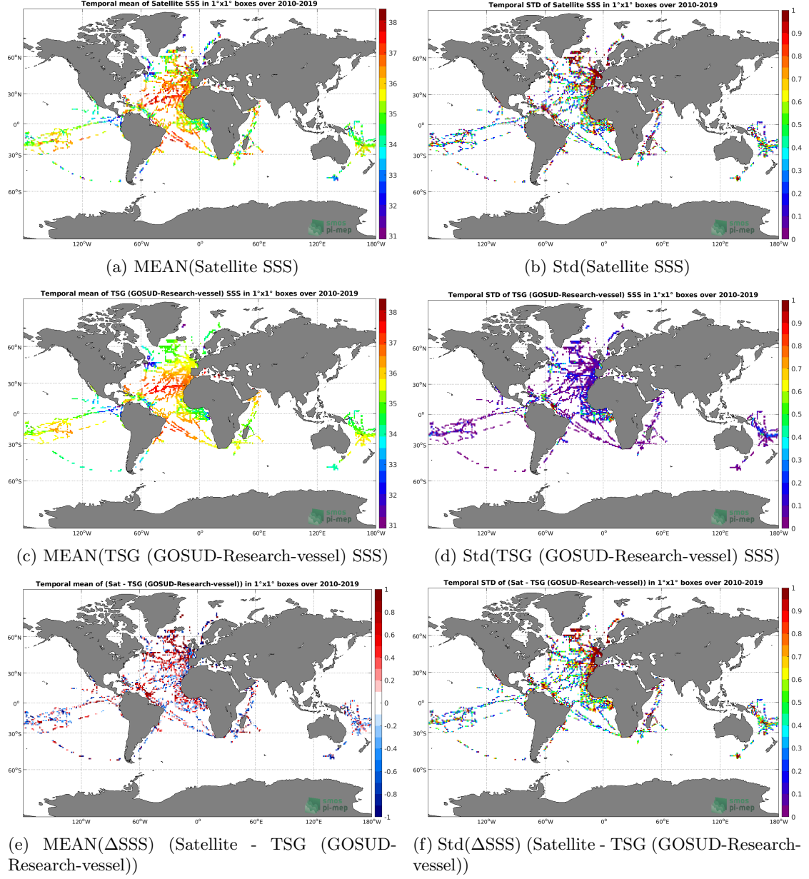
Figure 6: Temporal mean (left) and Std (right) of SSS from SMOS SSS L2 v662 (ESA) (top), TSG (GOSUD-Research-vessel) (middle), and of \Delta SSS (Satellite - TSG (GOSUD-Research-vessel)). Only match-up pairs are used to generate these maps.
