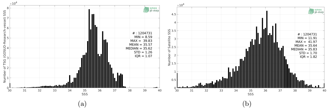
Figure 2: Histograms of SSS from TSG (GOSUD-Research-vessel) (a) and SMOS SSS L2 v662 (ESA) (b) considering all match-up pairs per bins of 0.1 over the Global Ocean Pi-MEP region and for the full satellite product period.
