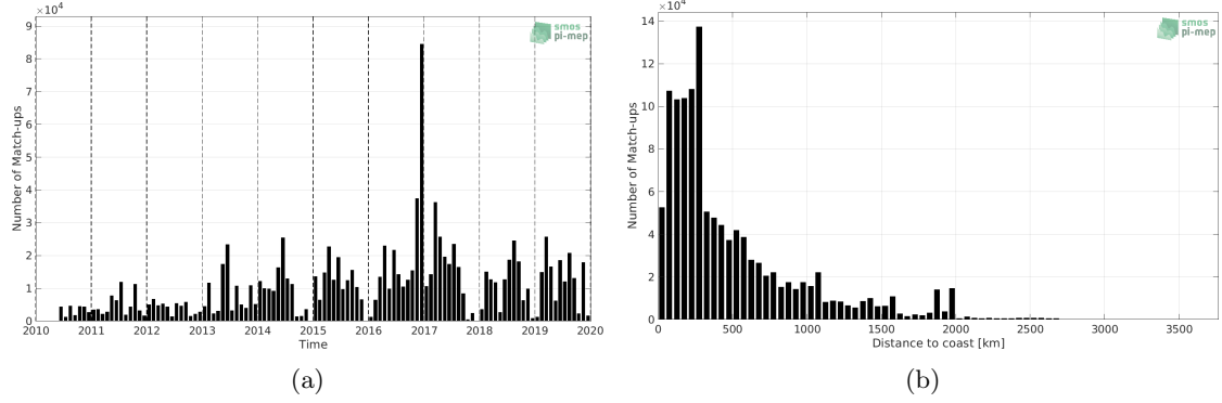
Figure 1: Number of match-ups between TSG (GOSUD-Research-vessel) and SMOS SSS L2 v662 (ESA) SSS as a function of time (a) and as function of the distance to coast (b) over the Global Ocean Pi-MEP region and for the full satellite product period.
