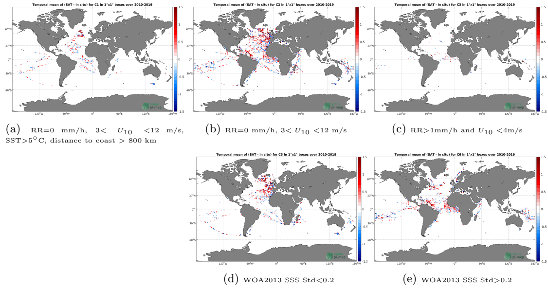
Figure 12: Temporal mean gridded over spatial boxes of size 1^\circ \times 1^\circ of \Delta SSS (SMOS SSS L2 v662 (ESA) - TSG (GOSUD-Research-vessel)) for 5 different subdatasets corresponding to: RR=0 mm/h, 3 < U_{10} < 12 m/s, SST > 5^\circ\text{C} , distance to coast > 800 km (a), RR=0 mm/h, 3 < U_{10} < 12 m/s (b), RR > 1 mm/h and U_{10} < 4 m/s (c), WOA2013 SSS Std < 0.2 (d), WOA2013 SSS Std > 0.2 (e).
