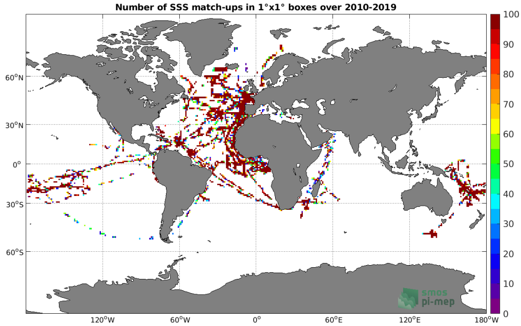
Figure 4: Number of SSS match-ups between TSG (GOSUD-Research-vessel) SSS and the SMOS SSS L2 v662 (ESA) SSS product for the Global Ocean Pi-MEP region over 1^\circ \times 1^\circ boxes and for the full satellite product period.
