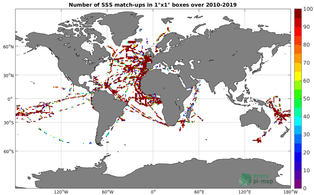
Figure 4: Number of SSS match-ups between TSG (GOSUD-Research-vessel) SSS and the SMOS SSS L2 v662 (ESA) SSS product for the Global Ocean Pi-MEP region over 1^\circ \times 1^\circ boxes and for the full satellite product period.
