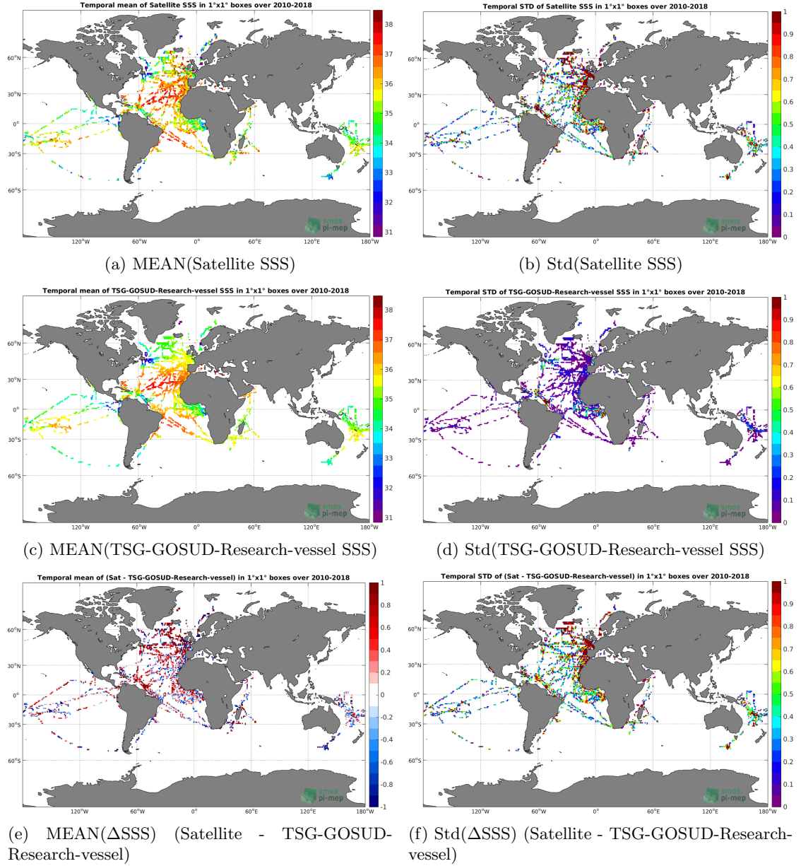
Figure 6: Temporal mean (left) and Std (right) of SSS from SMOS L2 v662 (ESA) (top), TSG-GOSUD-Research-vessel (middle), and of \Delta SSS (Satellite - TSG-GOSUD-Research-vessel). Only match-up pairs are used to generate these maps.
