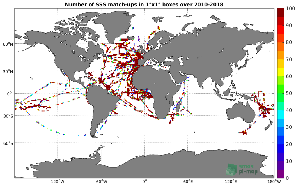
Figure 4: Number of SSS match-ups between TSG-GOSUD-Research-vessel SSS and the SMOS L2 v662 (ESA) SSS product for the Global Ocean Pi-MEP region over 1^\circ \times 1^\circ boxes and for the full satellite product period.
