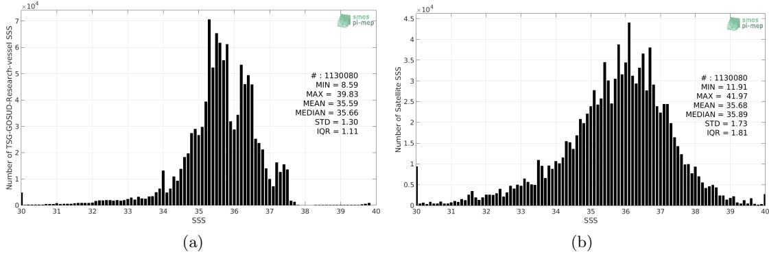
Figure 2: Histograms of SSS from TSG-GOSUD-Research-vessel (a) and SMOS L2 v662 (ESA) (b) considering all match-up pairs per bins of 0.1 over the Global Ocean Pi-MEP region and for the full satellite product period.
