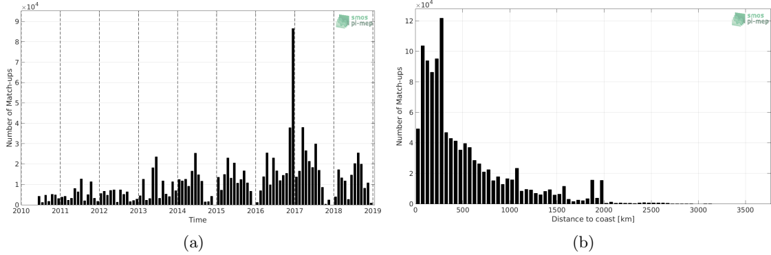
Figure 1: Number of match-ups between TSG-GOSUD-Research-vessel and SMOS L2 v662 (ESA) SSS as a function of time (a) and as function of the distance to coast (b) over the Global Ocean Pi-MEP region and for the full satellite product period.
