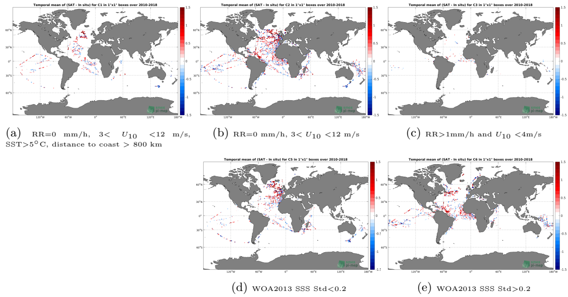
Figure 12: Temporal mean gridded over spatial boxes of size 1^\circ \times 1^\circ of \Delta SSS (SMOS L2 v662 (ESA) - TSG-GOSUD-Research-vessel) for 5 different subdatasets corresponding to: RR=0 mm/h, 3 < U_{10} < 12 m/s, SST > 5^\circ\text{C} , distance to coast > 800 km (a), RR=0 mm/h, 3 < U_{10} < 12 m/s (b), RR > 1 mm/h and U_{10} < 4 m/s (c), WOA2013 SSS Std < 0.2 (d), WOA2013 SSS Std > 0.2 (e).
