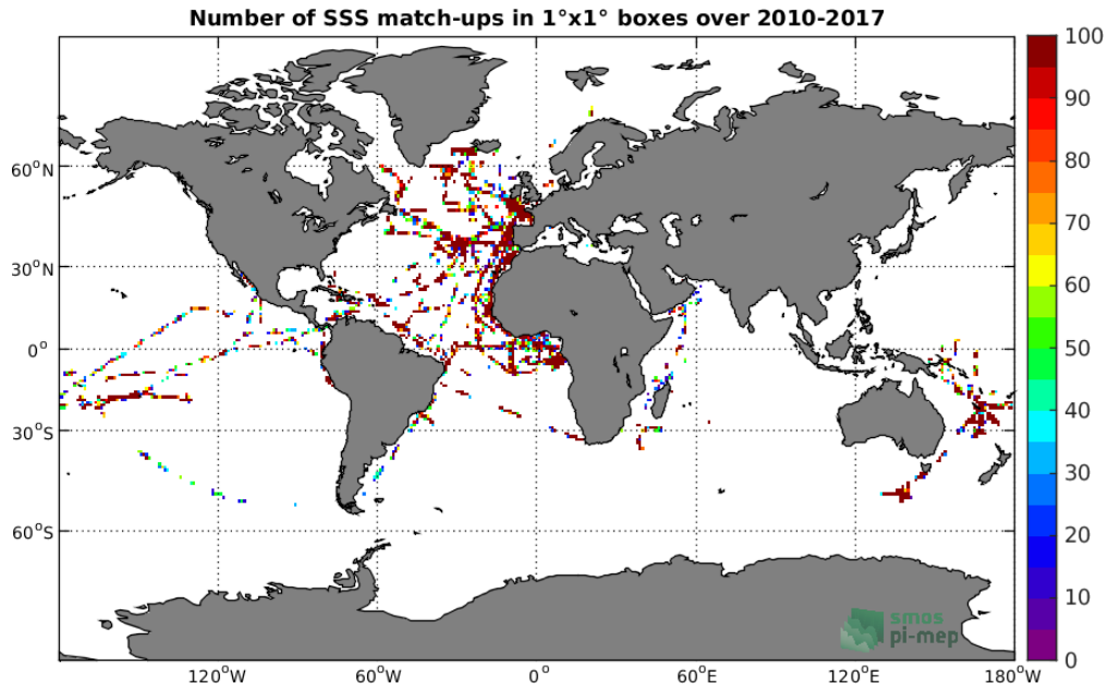
Figure 4: Number of SSS match-ups between TSG-GOSUD-Research-vessel SSS and the SMOS-L2-DPGS-v662 SSS product for the Global Ocean Pi-MEP region over 1^\circ \times 1^\circ boxes and for the full satellite product period.
