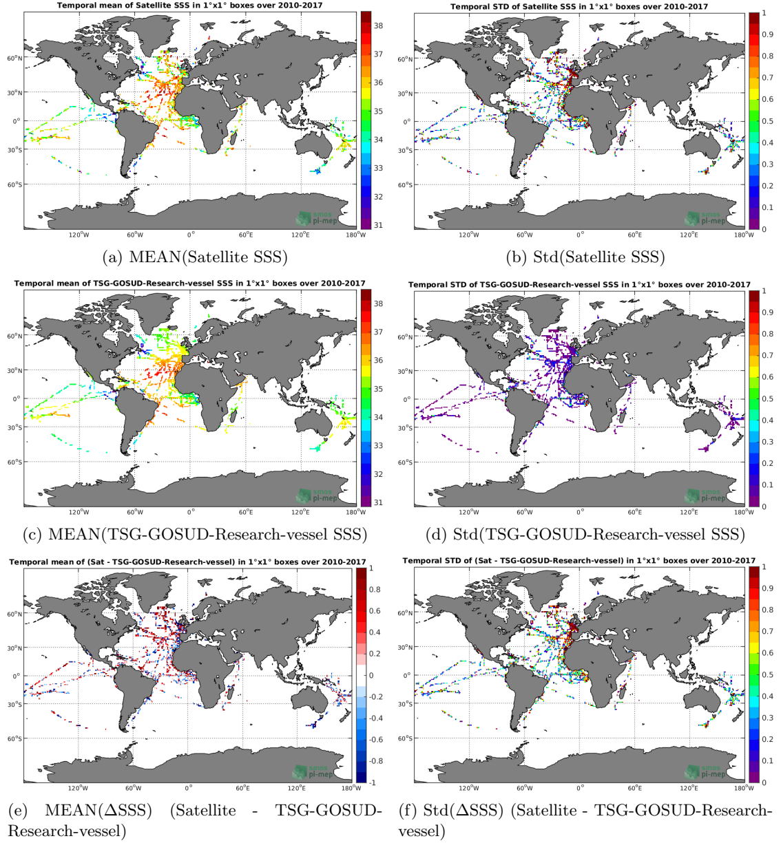
Figure 6: Temporal mean (left) and Std (right) of SSS from SMOS-L2-DPGS-v662 (top), TSG-GOSUD-Research-vessel (middle), and of \Delta SSS (Satellite - TSG-GOSUD-Research-vessel). Only match-up pairs are used to generate these maps.
