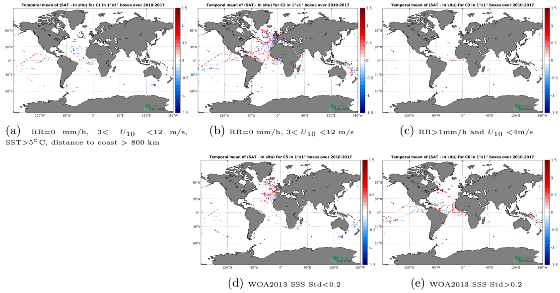
Figure 12: Temporal mean gridded over spatial boxes of size 1^\circ \times 1^\circ of \Delta SSS (SMOS-L2-DPGS-v662 - TSG-GOSUD-Research-vessel) for 5 different subdatasets corresponding to:RR=0 mm/h, 3 < U_{10} < 12 m/s, SST >5^\circ\text{C} , distance to coast > 800 km (a), RR=0 mm/h, 3 < U_{10} < 12 m/s (b), RR >1 mm/h and U_{10} < 4 m/s (c), WOA2013 SSS Std <0.2 (d), WOA2013 SSS Std >0.2 (e).
