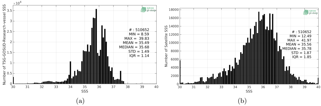
Figure 2: Histograms of SSS from TSG-GOSUD-Research-vessel (a) and SMOS-L2-DPGS-v662 (b) considering all match-up pairs per bins of 0.1 over the Global Ocean Pi-MEP region and for the full satellite product period.
