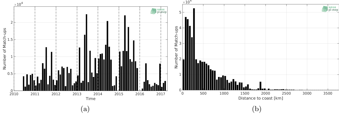
Figure 1: Number of match-ups between TSG-GOSUD-Research-vessel and SMOS-L2-DPGS-v662 SSS as a function of time (a) and as function of the distance to coast (b) over the Global Ocean Pi-MEP region and for the full satellite product period.
