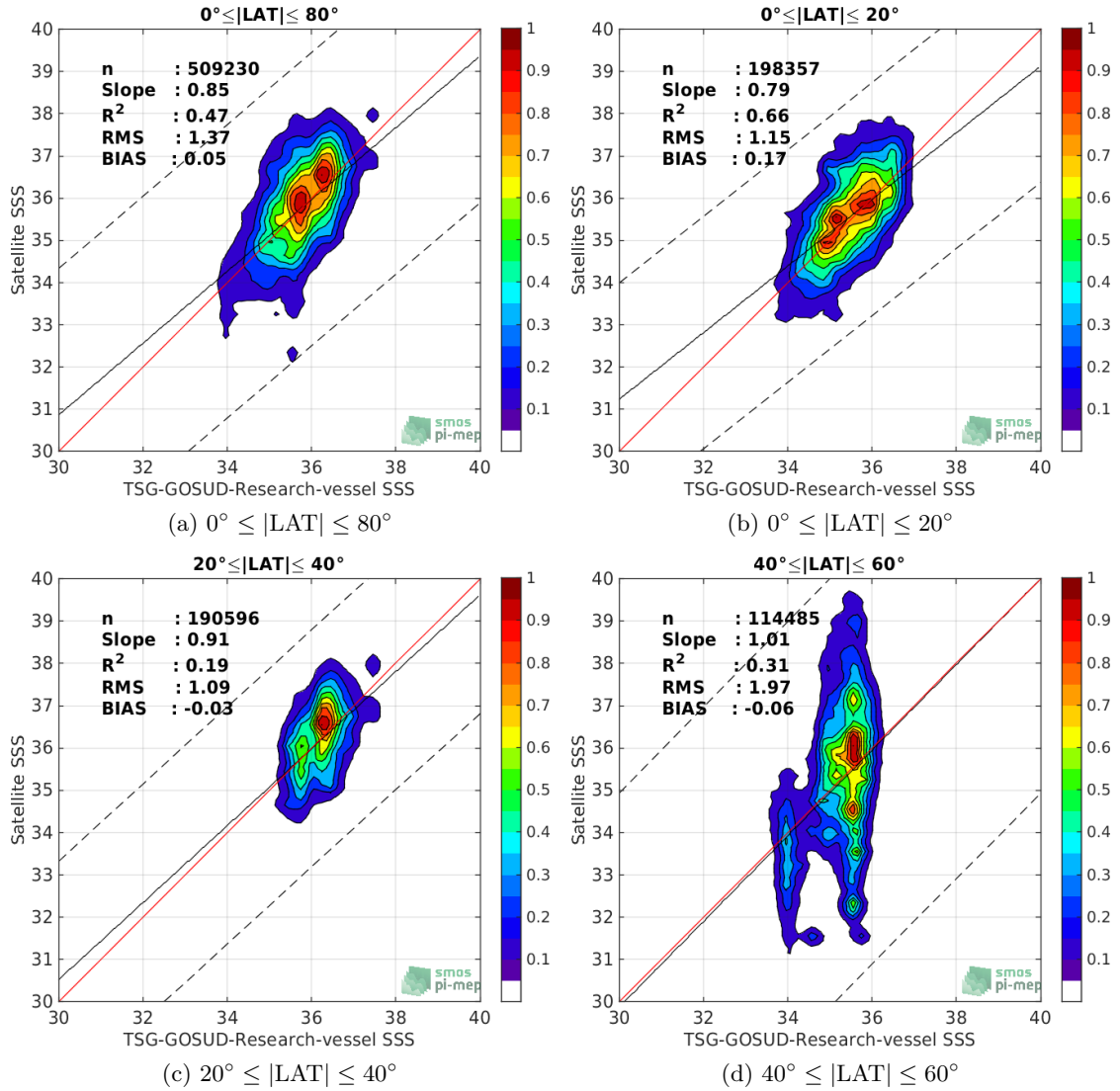
Figure 9: Contour maps of the concentration of SMOS-L2-DPGS-v662 SSS (y-axis) versus TSG-GOSUD-Research-vessel SSS (x-axis) at match-up pairs for different latitude bands. For each plot, the red line shows x=y . The black thin and dashed lines indicate a linear fit through the data cloud and the \pm 95\% confidence levels, respectively. The number match-up pairs n , the slope and R^2 coefficient of the linear fit, the root mean square (RMS) and the mean bias between satellite and in situ data are indicated for each latitude band in each plots.
